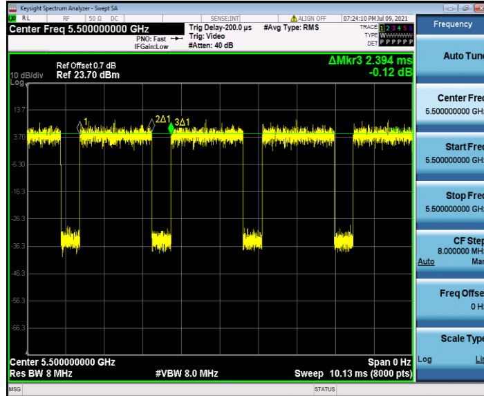
11AC20SISO_Ant2_5500
