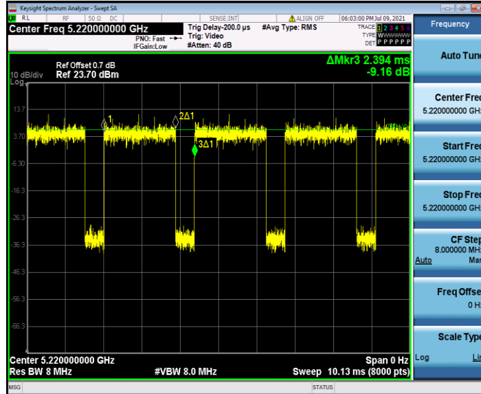
11AC20SISO_Ant2_5220
