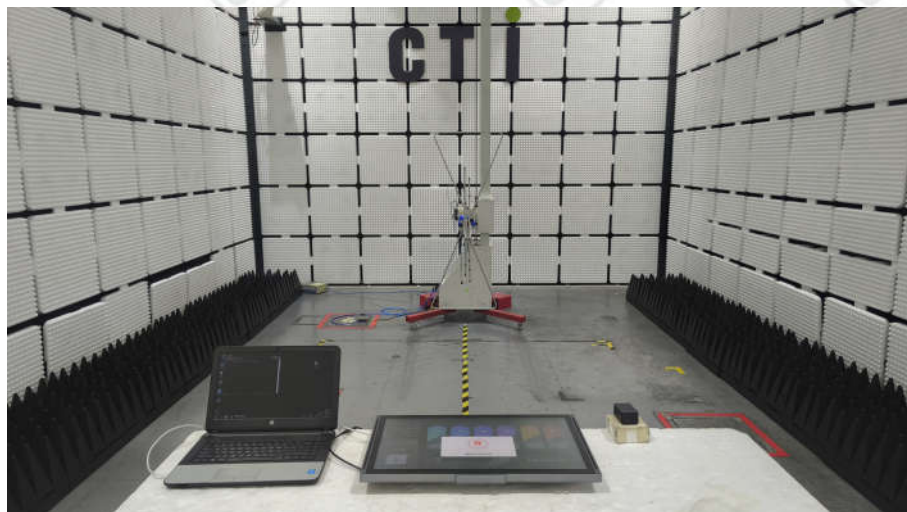
Radiated spurious emission Test Setup-1(Below 1GHz)
