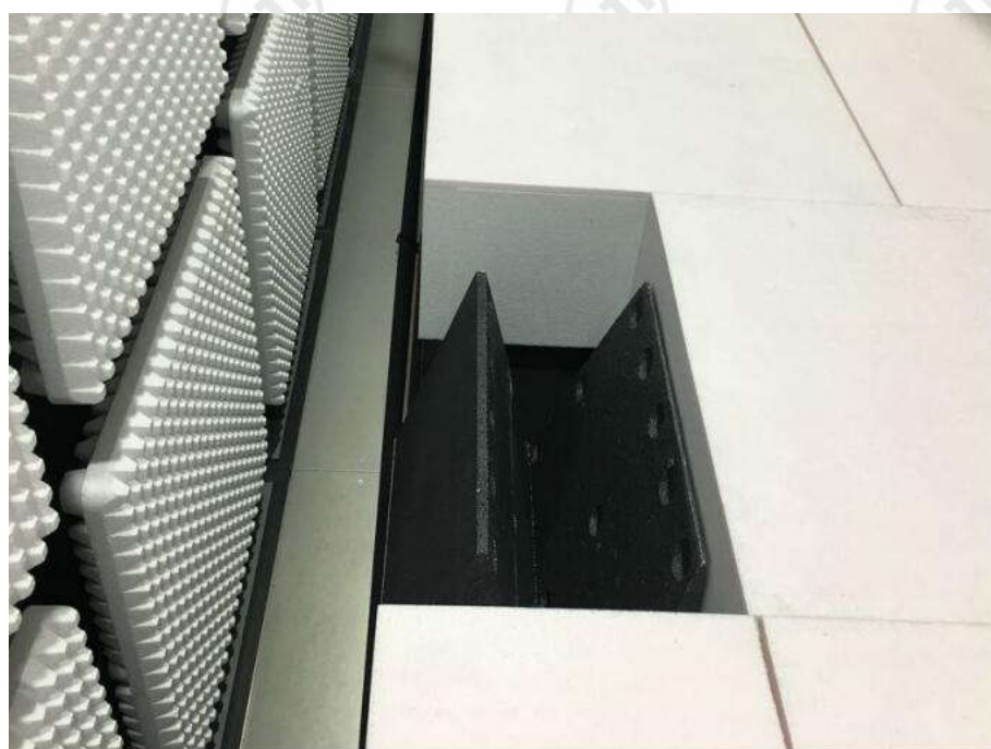
Radiated spurious emission Test Setup-3 There are absorbing materials under the ground.
