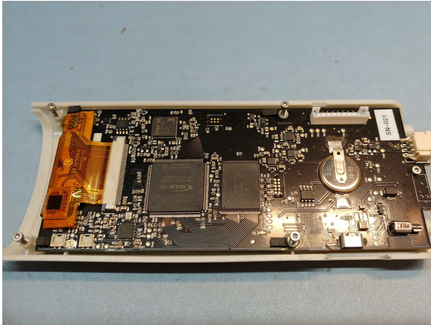
Right Side – Mainboard attached to Front Cover
