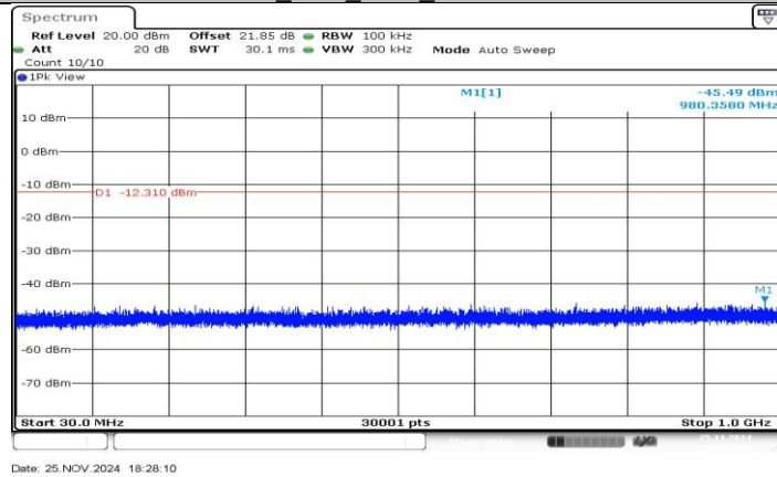
3DH5_Ant1_2480_30~1000
