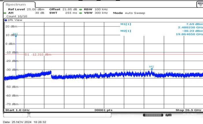
3DH5_Ant1_2480_1000~26500
