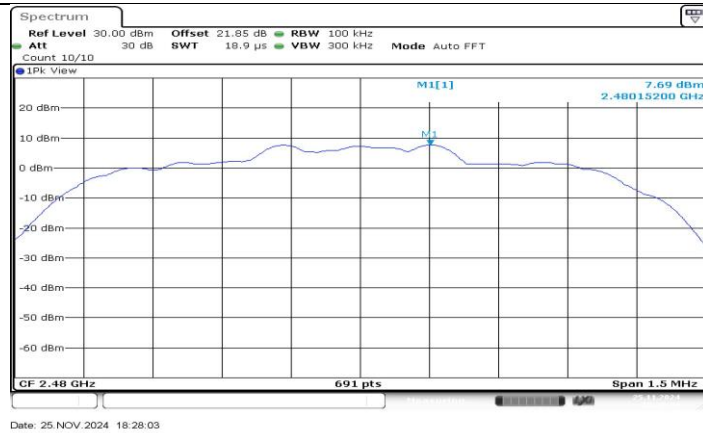
3DH5_Ant1_2480_0~Reference
