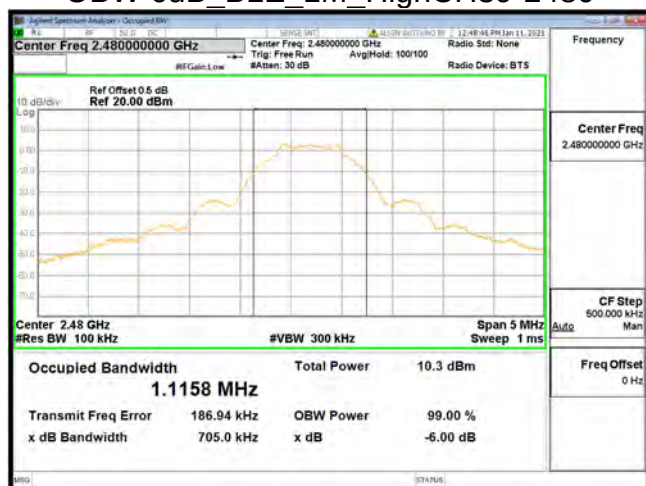
OBW 6dB_BLE_1M_HighCH39-2480
