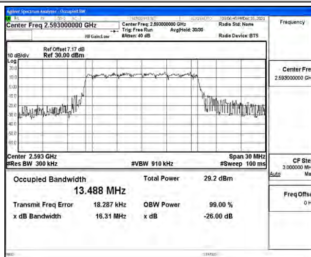
Band41-15MHz-QPSK-41515
