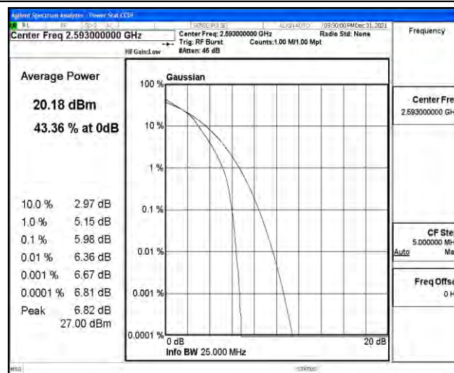
Band41-15MHz-16QAM-41515
