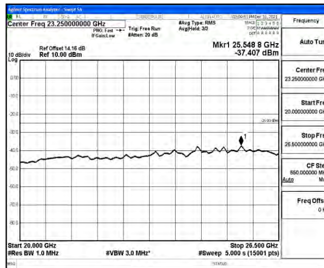
Band41-5MHz-16QAM-40620-Range1:0.009~0.15MHz
