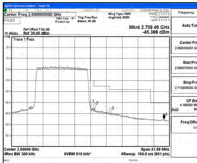
Band41-20MHz-QPSK-39750
