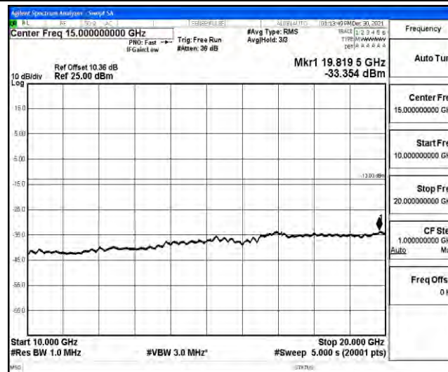
Band4-20MHz-16QAM-20300-Range5:10000~20000MHz
