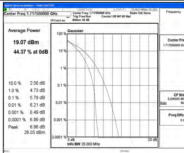
Band4-15MHz-QPSK-20175
