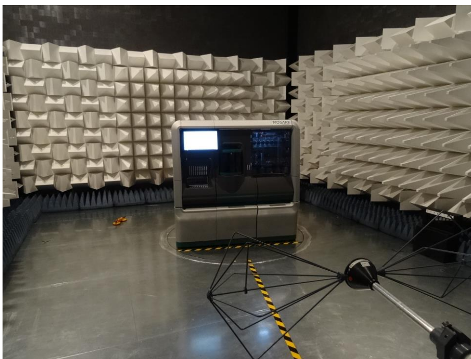
Figure 2 EUT / set up - test module ER low (radiated emissions 30 - 200 MHz)
