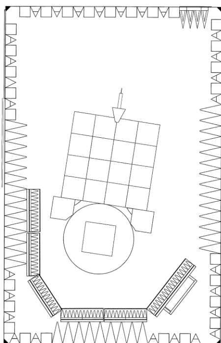
Figure 8 Set-up - ER2 (1 - 18 GHz)
