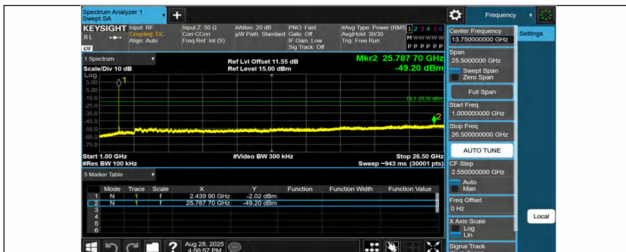
BLE_2M-Ant1-2440-1000~26500-PASS
