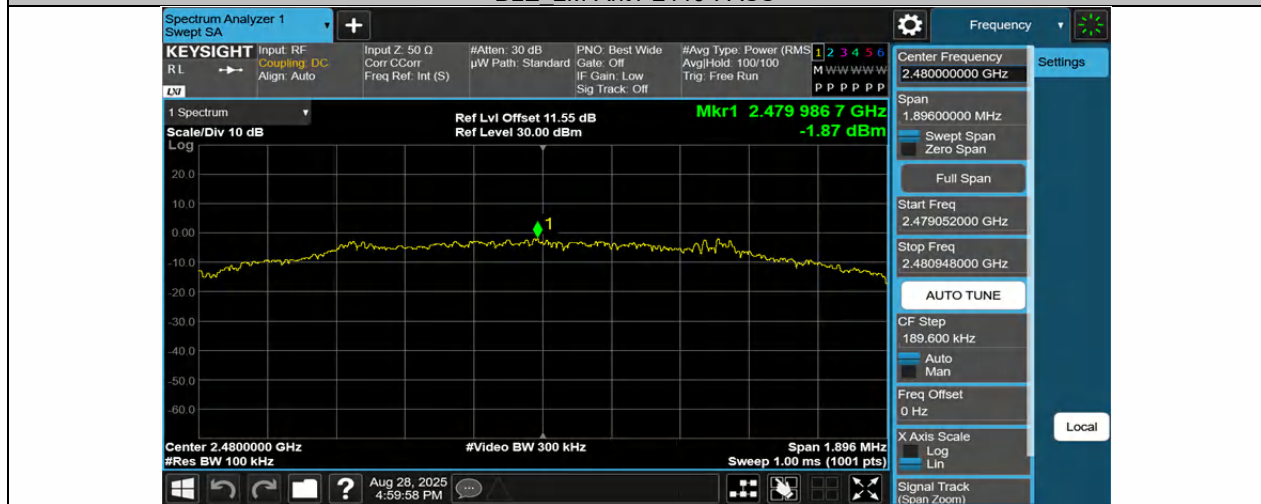
BLE_2M-Ant1-2480-PASS
