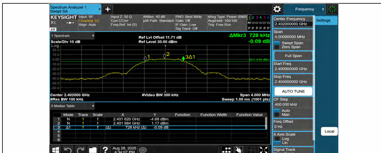
BLE_1M-Ant1-2402-PASS
