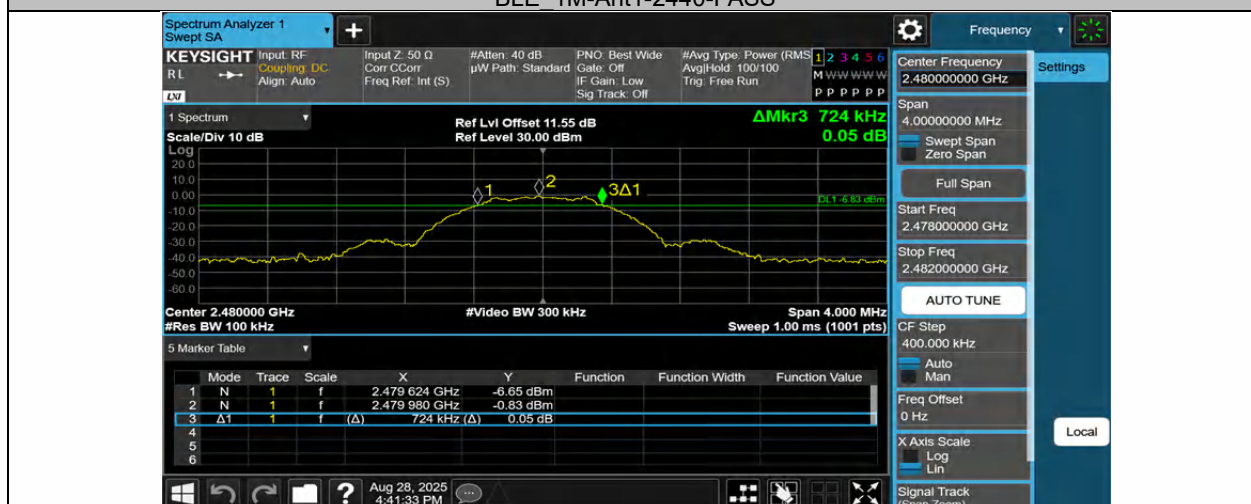
BLE_1M-Ant1-2480-PASS
