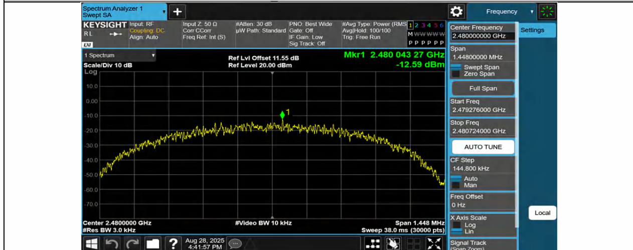
BLE_1M-Ant1-2480-PASS
