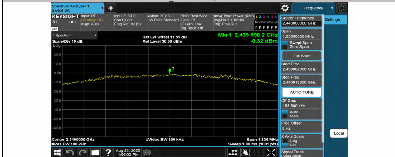
BLE_2M-Ant1-2440-PASS
