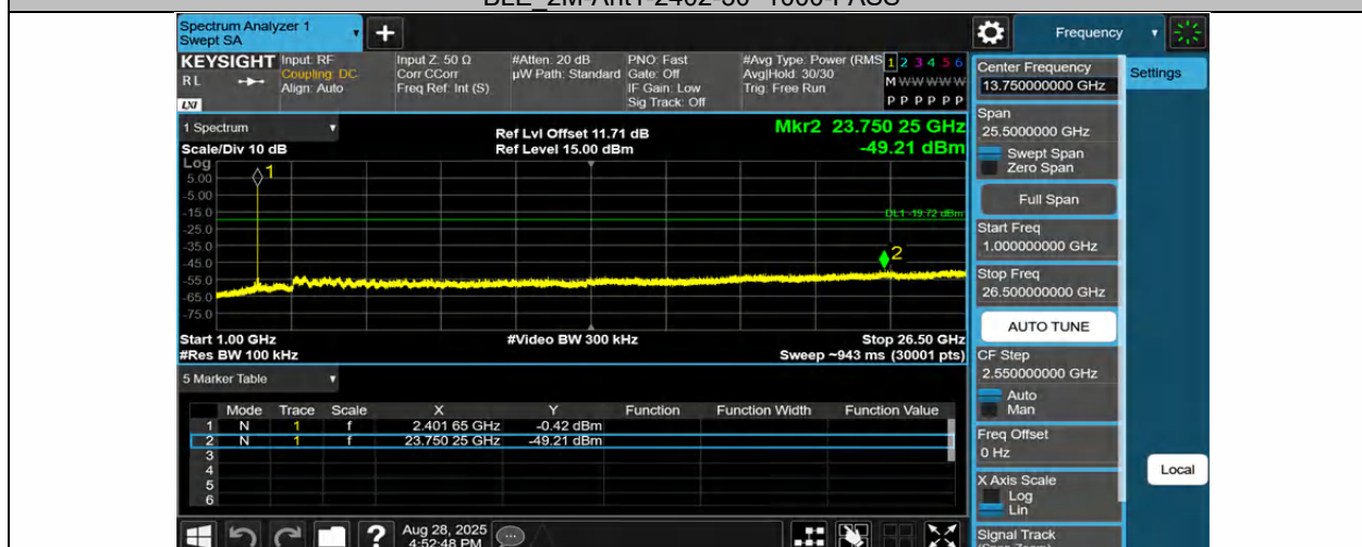
BLE_2M-Ant1-2402-1000~26500-PASS
