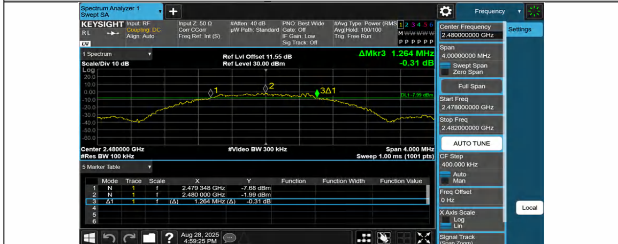
BLE_2M-Ant1-2480-PASS
