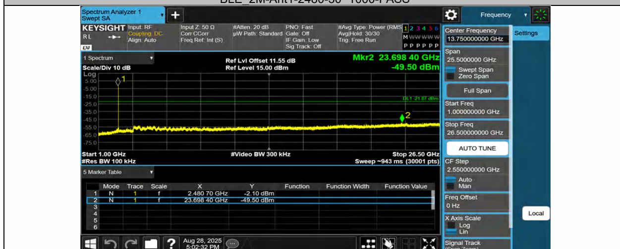
BLE_2M-Ant1-2480-1000~26500-PASS
