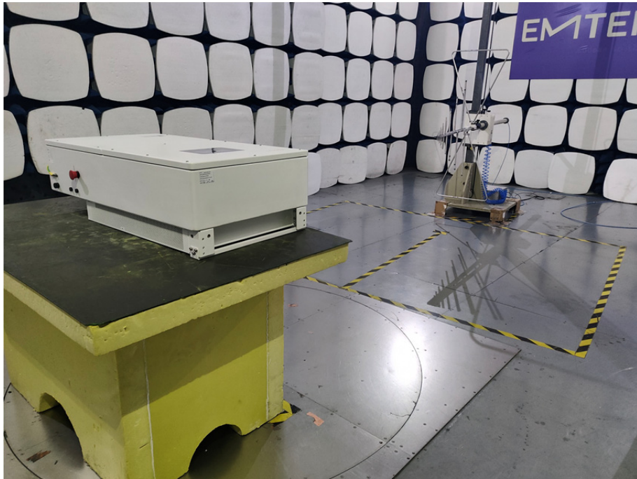
Radiation emission below 1 GHz
