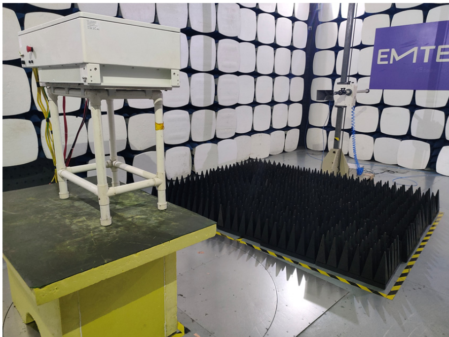
Radiation emission above 1 GHz
