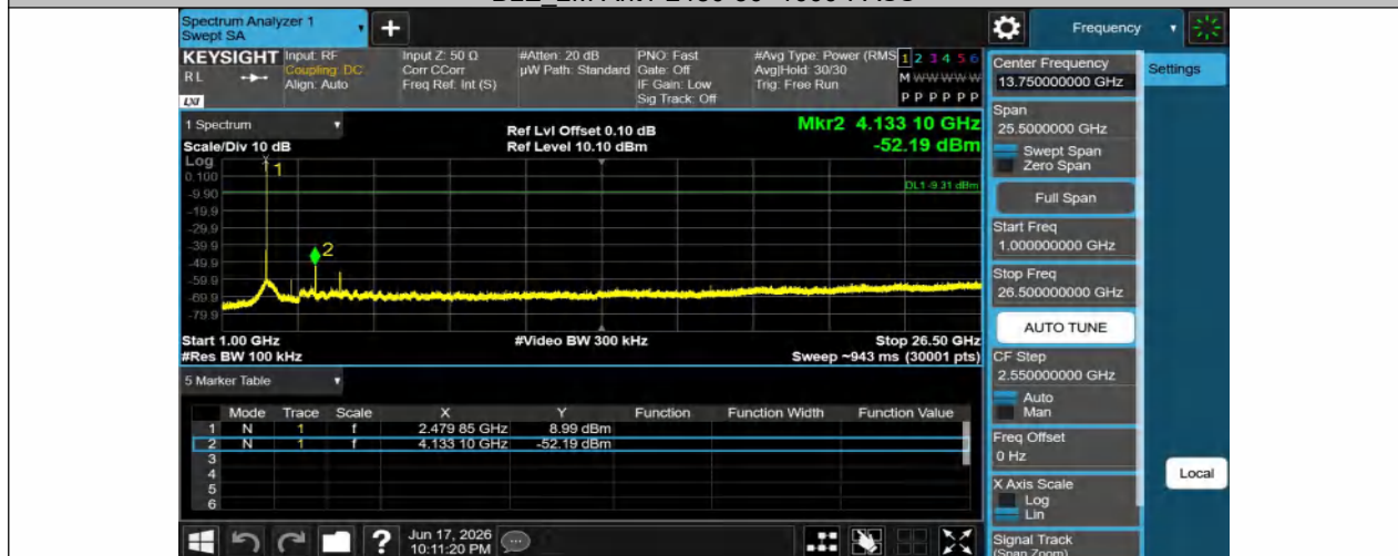
BLE_2M-Ant1-2480-1000~26500-PASS
