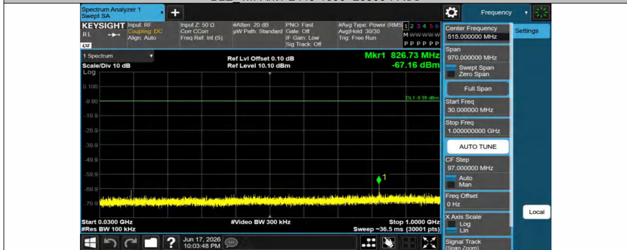
BLE_1M-Ant1-2480-30~1000-PASS
