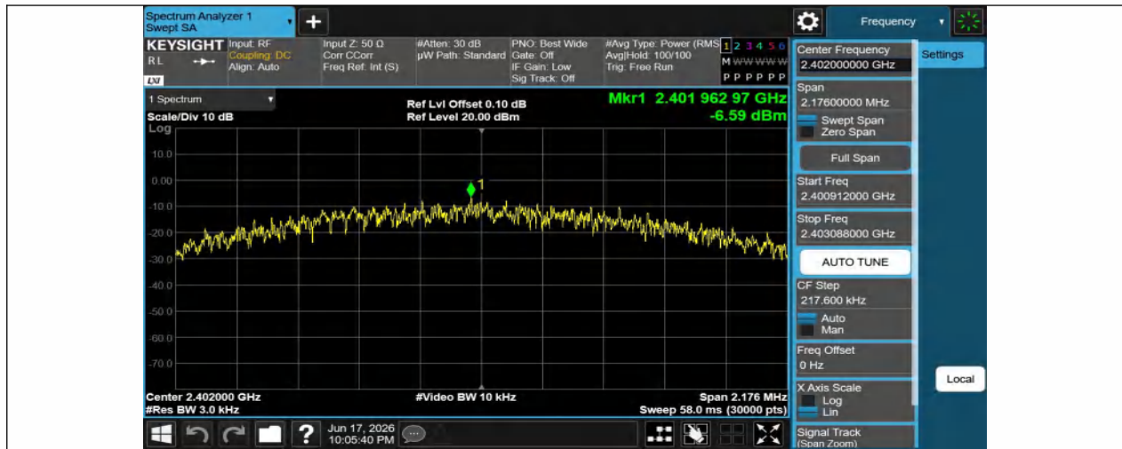
BLE_2M-Ant1-2402-PASS
