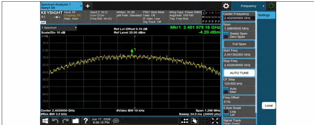
BLE_1M-Ant1-2402-PASS
