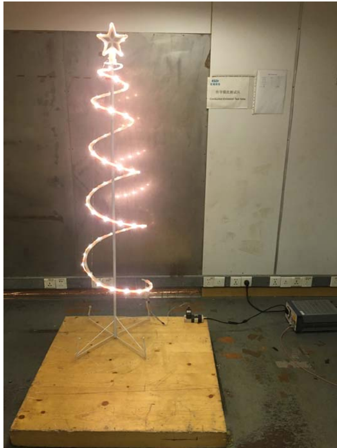
Photograph of set-up for AC Power line Conducted Emission
