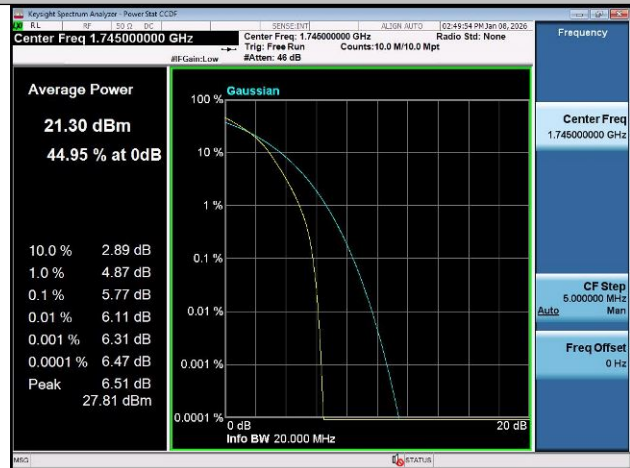
Band66-20MHz-16QAM-132572-100RB#0-PASS
