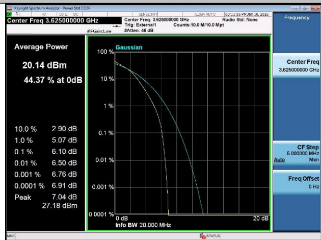
Band48-20MHz-16QAM-56640-100RB#0-PASS
