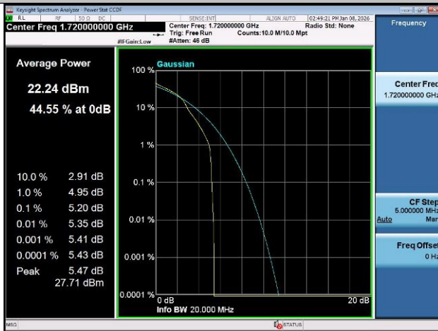
Band66-20MHz-16QAM-132322-1RB#0-PASS
