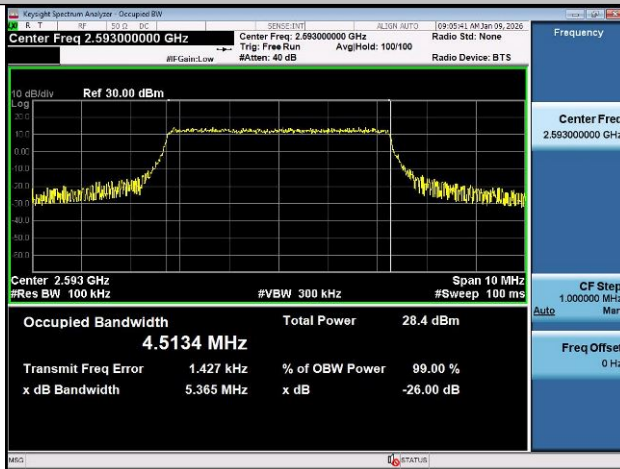
Band41-10MHz-QPSK-40620-50RB#0-PASS
