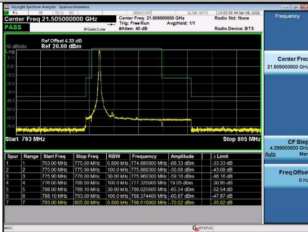
Band13-5MHz-QPSK-23255-1RB#24-PASS
