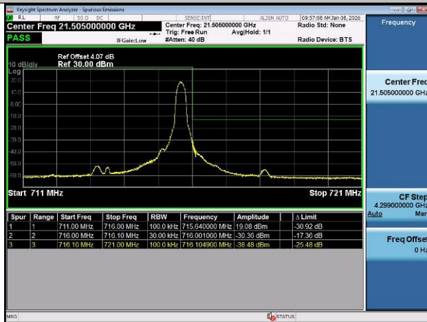
Band12-10MHz-QPSK-23060-1RB#0-PASS
