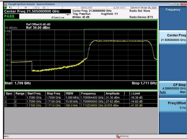
Band4-1.4MHz-QPSK-20393-6RB#0-PASS
