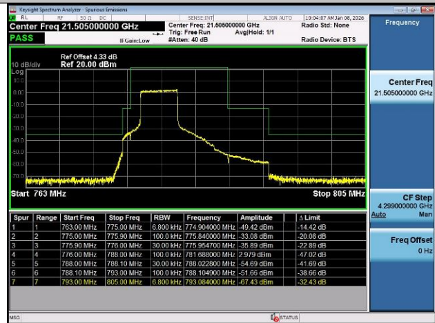
Band13-5MHz-QPSK-23255-25RB#0-PASS
