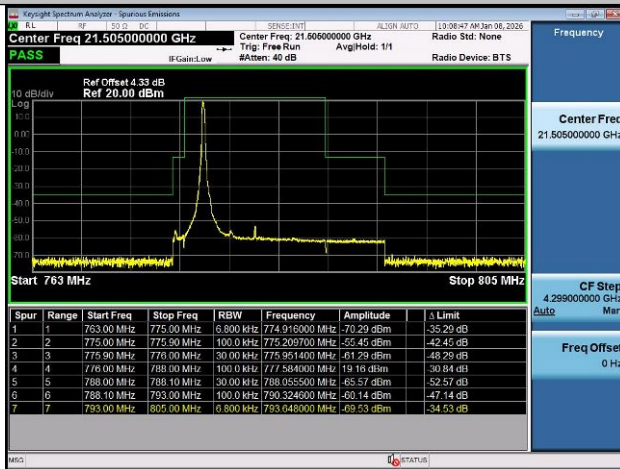
Band13-10MHz-QPSK-23230-50RB#0-PASS
