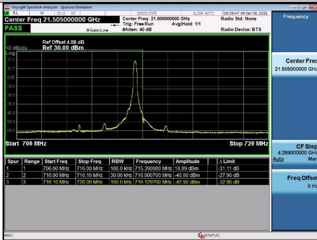
Band13-5MHz-QPSK-23205-1RB#0-PASS
