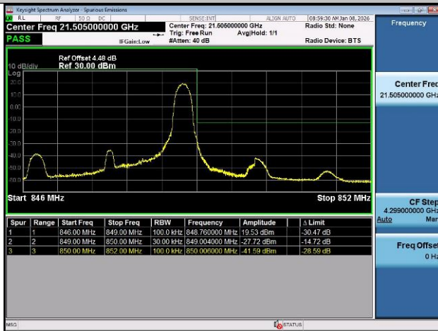
Band5-5MHz-QPSK-20425-1RB#0-PASS
