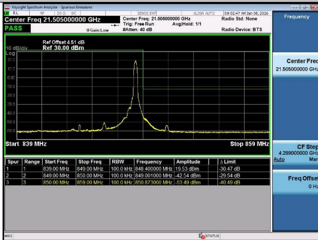
Band12-1.4MHz-QPSK-23017-1RB#0-PASS
