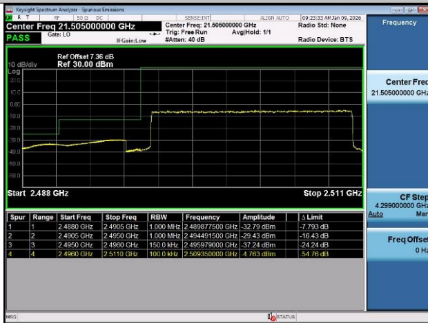
Band41-15MHz-QPSK-41515-75RB#0-PASS
