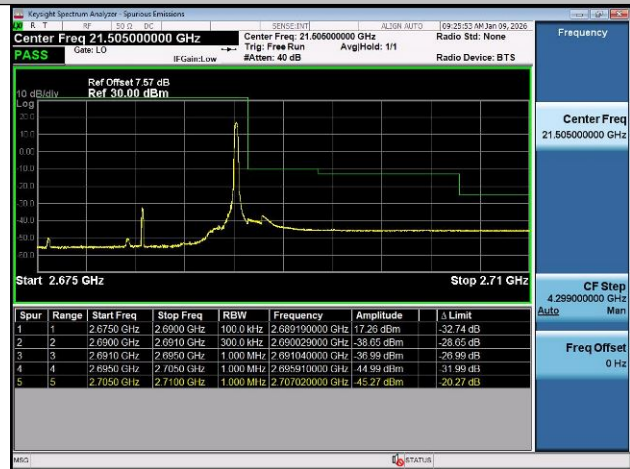
Band41-20MHz-QPSK-39750-1RB#0-PASS
