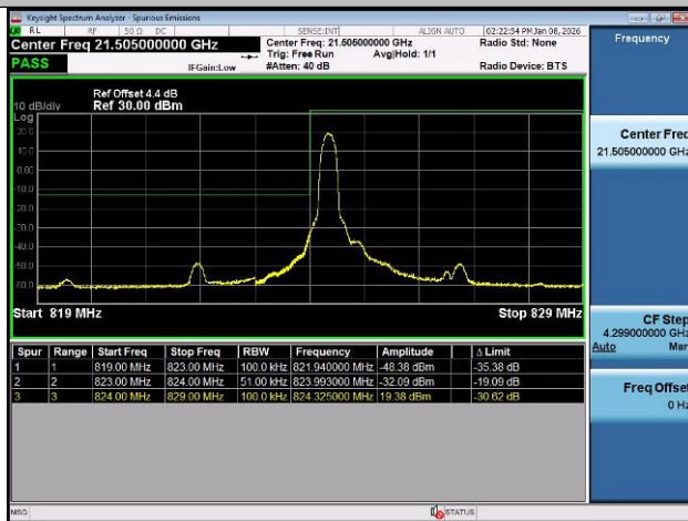
Band26(824-849)-5MHz-QPSK-27015-1RB#24-PASS
