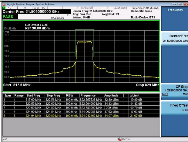
Band26(814-824)-3MHz-QPSK-26705-15RB#0-PASS
