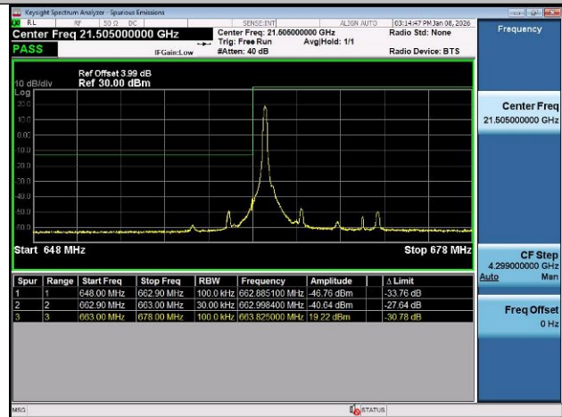
Band71-15MHz-QPSK-133397-1RB#74-PASS
