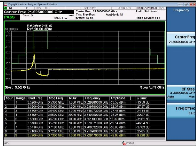
Band48-20MHz-QPSK-55340-100RB#0-PASS
