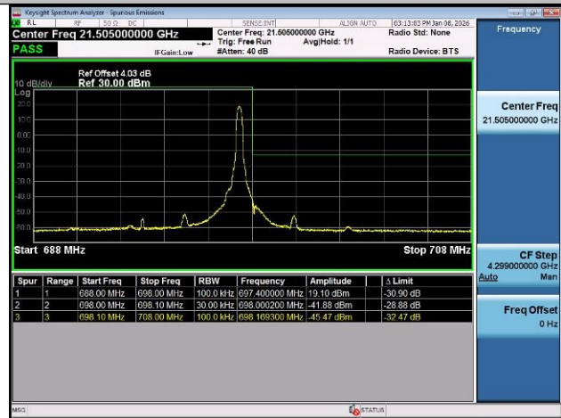
Band71-15MHz-QPSK-133197-1RB#0-PASS
