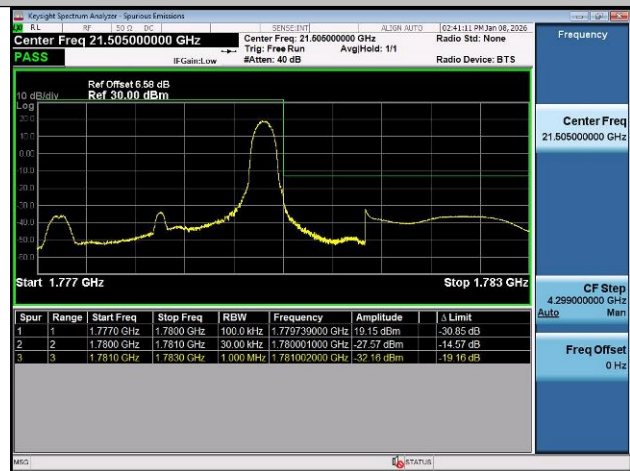
Band66-5MHz-QPSK-131997-1RB#0-PASS
