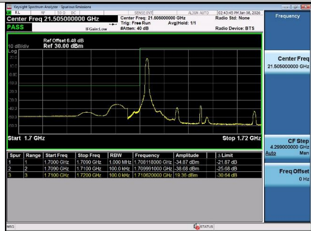
Band66-10MHz-QPSK-132622-1RB#49-PASS
