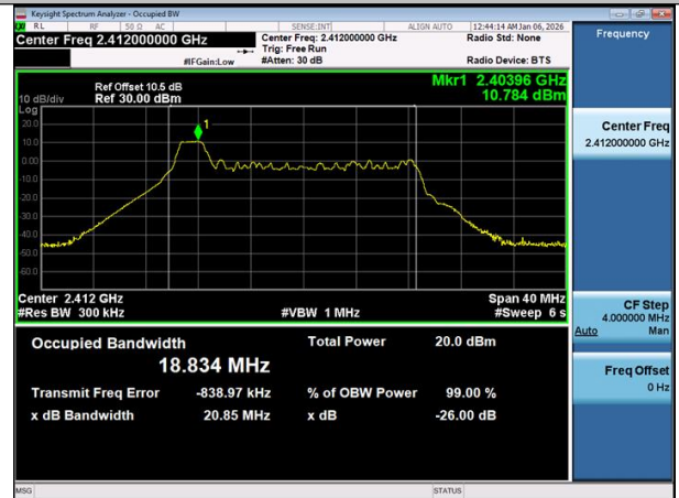
11AX20MIMO-Ant2-2412-26Tone-RU8
