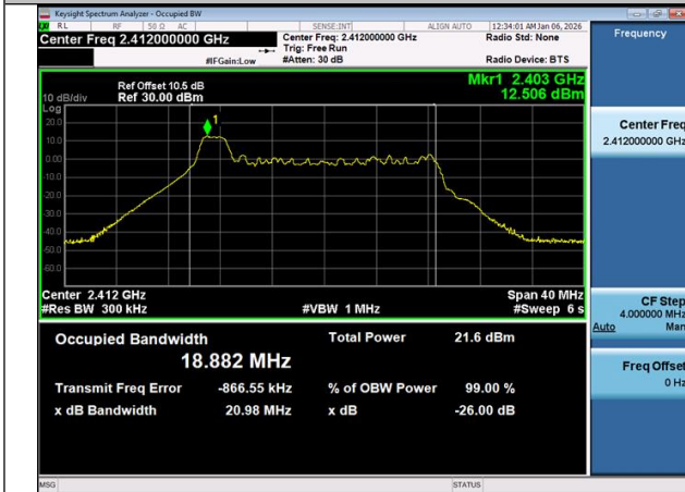
11AX20MIMO-Ant1-2412-26Tone-RU8
