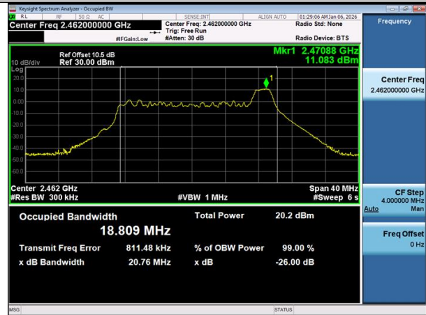
11AX20MIMO-Ant2-2462-26Tone-RU8
