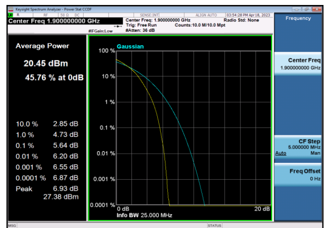
FDD02_HighRange_20MHz_1900_fullRB _Q16
