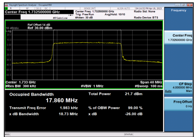
FDD04_MidRange_20_1732.5_Q16
