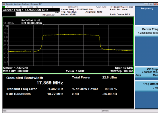
FDD04_MidRange_20_1732.5_QPSK
