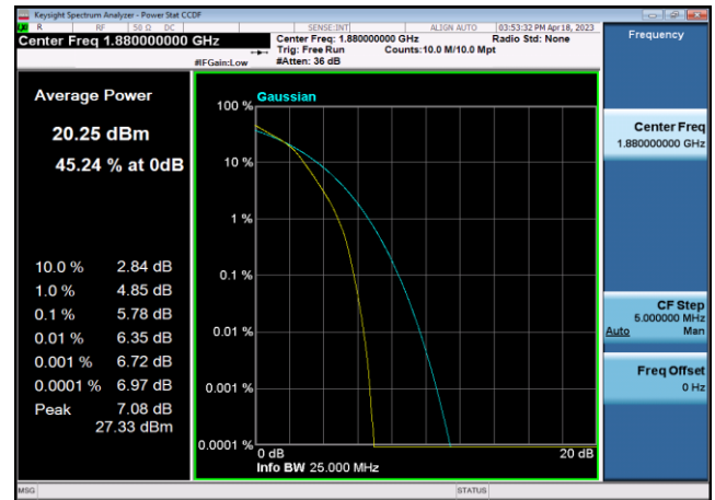
FDD02_HighRange_20MHz_1900_fullRB _Q16
