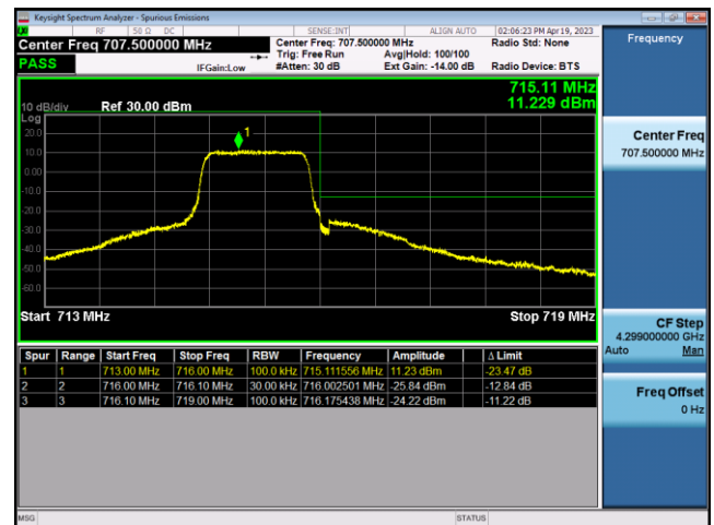
FDD12-3MHz-16QAM-LCH-1RB#0
