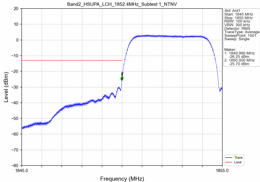
Band2_HSUPA_LCH_1852.4MHz_Subtest 1_NTNV
