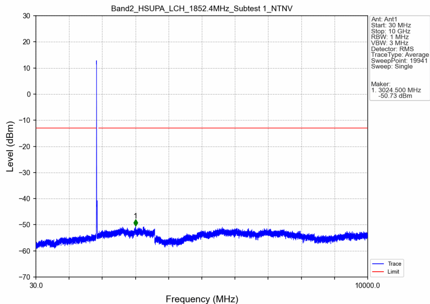
Band2_HSUPA_LCH_1852.4MHz_Subtest 1_NTNV
