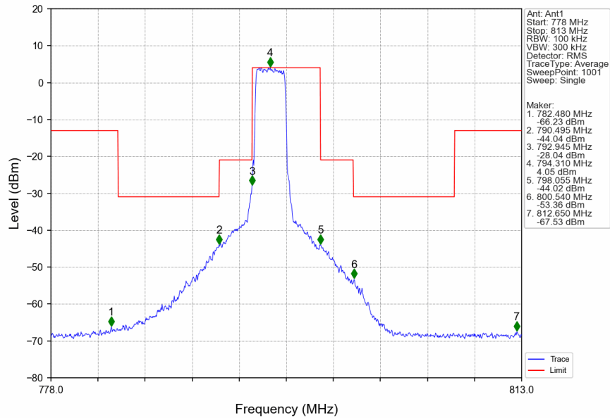
Band14_5MHz_16QAM_HCH_795.5MHz_RB_12_6_NTNV
