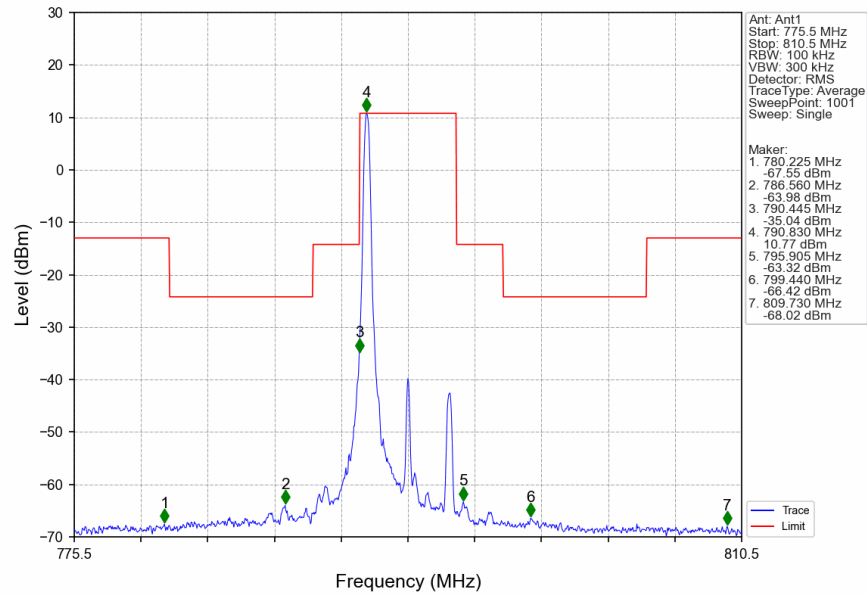
Band14_5MHz_256QAM_MCH_793MHz_RB_1_13_NTNV
