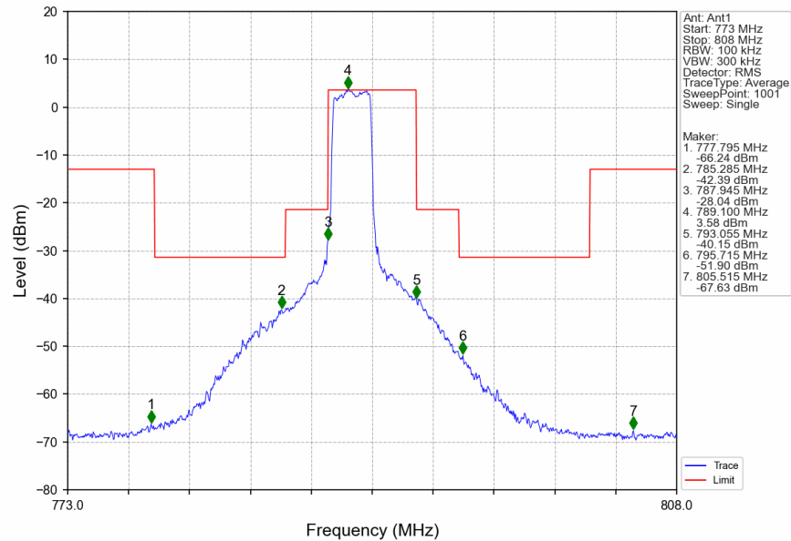
Band14_5MHz_64QAM_LCH_790.5MHz_RB_12_0_NTNV
