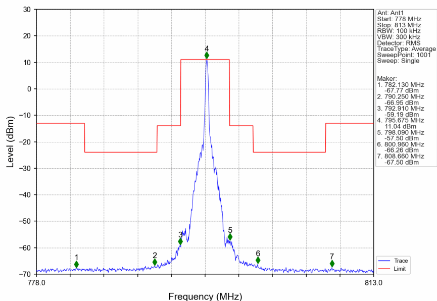
Band14_5MHz_256QAM_HCH_795.5MHz_RB_1_24_NTNV
