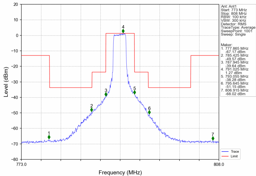
Band14_5MHz_256QAM_LCH_790.5MHz_RB_12_6_NTNV
