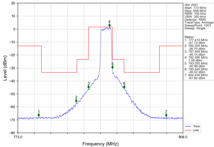
Band14_5MHz_256QAM_LCH_790.5MHz_RB_25_0_NTNV
