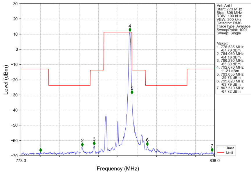
Band14_5MHz_256QAM_LCH_790.5MHz_RB_1_24_NTNV
