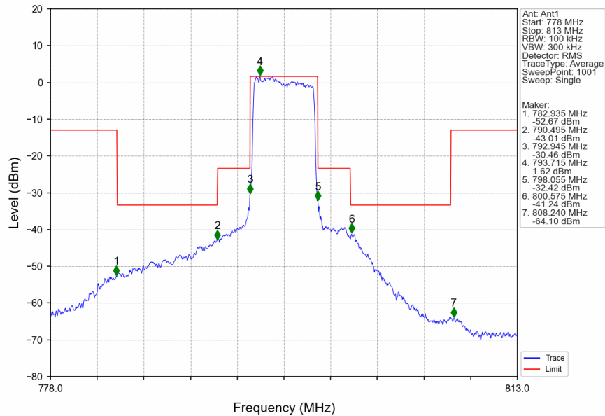
Band14_5MHz_16QAM_HCH_795.5MHz_RB_25_0_NTNV
