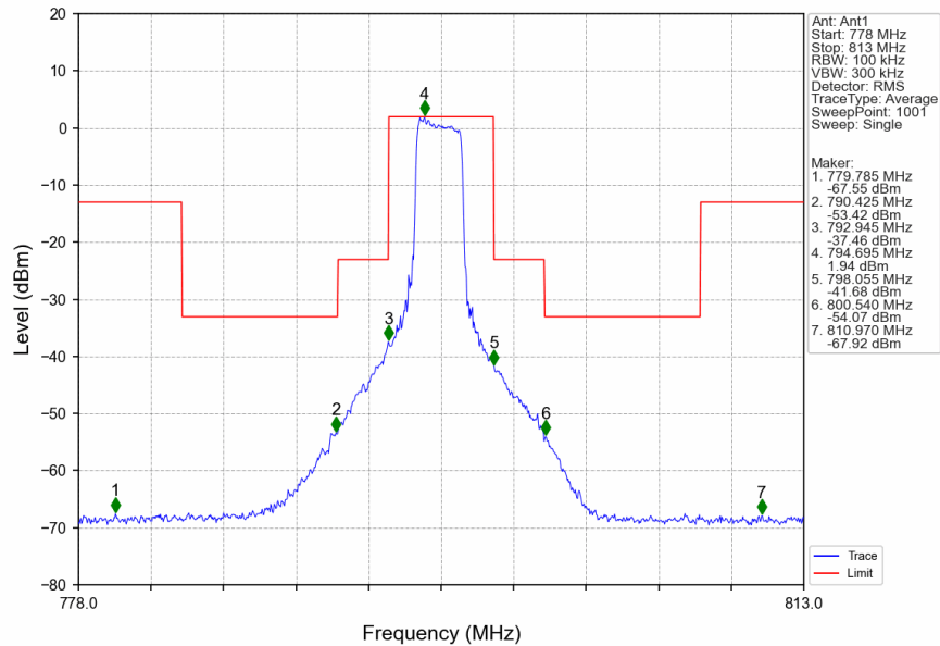
Band14_5MHz_256QAM_HCH_795.5MHz_RB_12_6_NTNV
