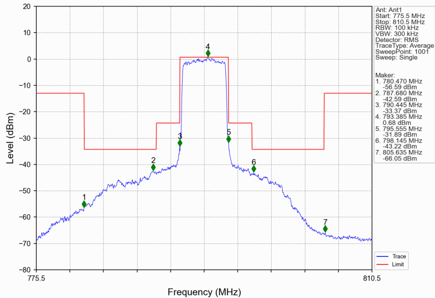
Band14_5MHz_64QAM_MCH_793MHz_RB_25_0_NTNV
