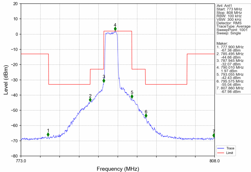
Band14_5MHz_256QAM_LCH_790.5MHz_RB_12_6_NTNV
