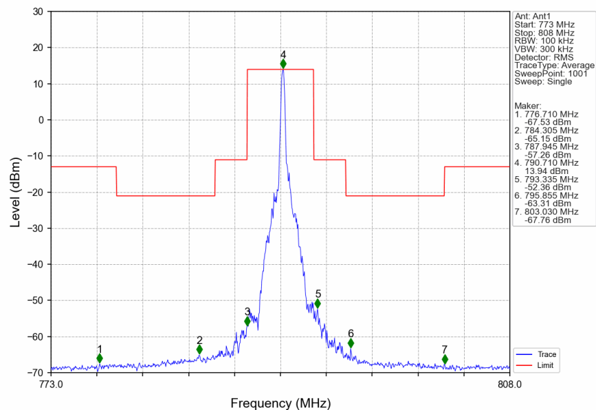
Band14_5MHz_64QAM_LCH_790.5MHz_RB_1_13_NTNV
