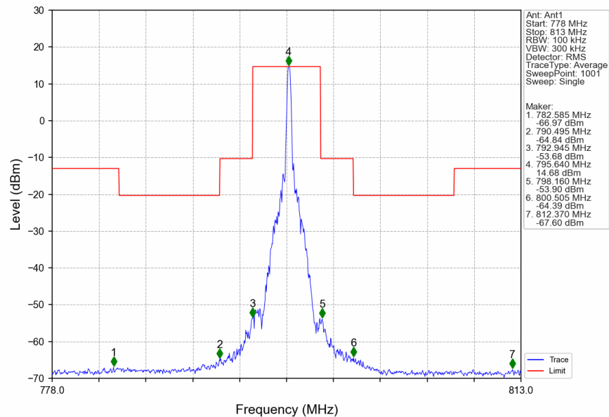
Band14_5MHz_16QAM_HCH_795.5MHz_RB_1_24_NTNV
