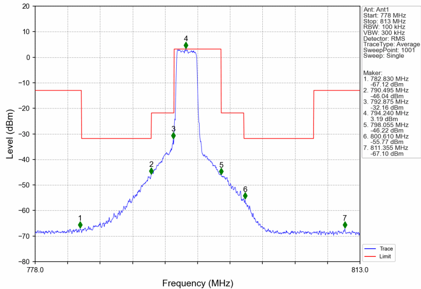
Band14_5MHz_64QAM_HCH_795.5MHz_RB_12_0_NTNV
