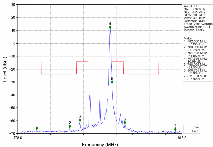
Band14_5MHz_256QAM_HCH_795.5MHz_RB_1_24_NTNV
