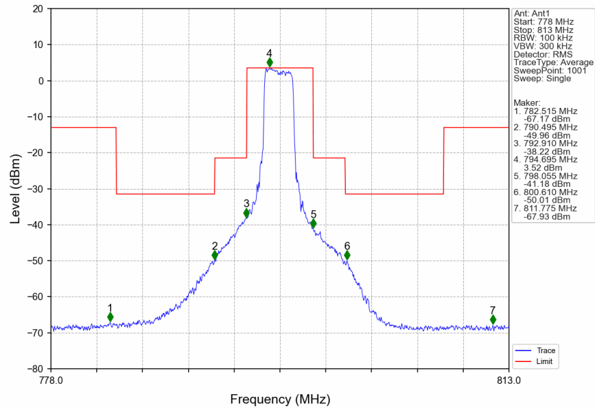
Band14_5MHz_64QAM_HCH_795.5MHz_RB_12_13_NTNV
