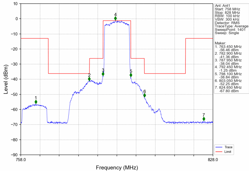
Band14_10MHz_16QAM_MCH_793MHz_RB_50_0_NTNV
