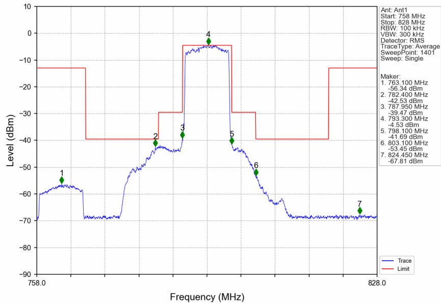
Band14_10MHz_256QAM_MCH_793MHz_RB_50_0_NTNV
