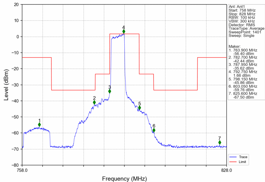
Band14_10MHz_16QAM_MCH_793MHz_RB_25_13_NTNV
