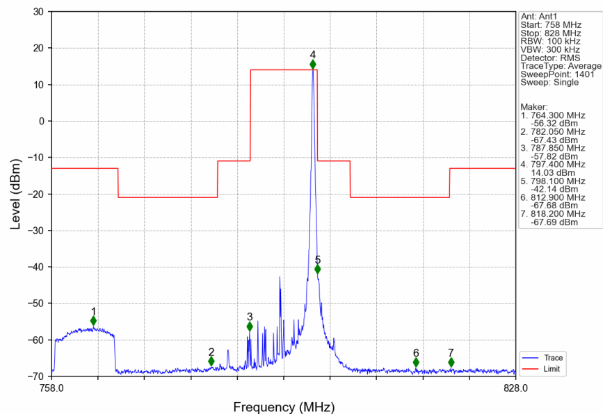
Band14_10MHz_16QAM_MCH_793MHz_RB_1_49_NTNV
