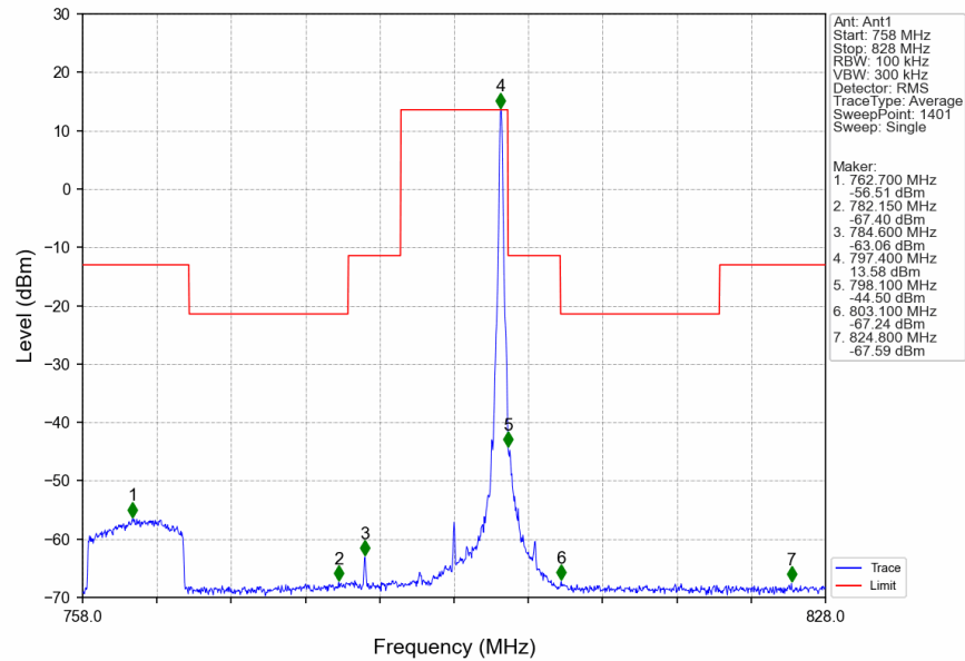
Band14_10MHz_64QAM_MCH_793MHz_RB_25_0_NTNV
