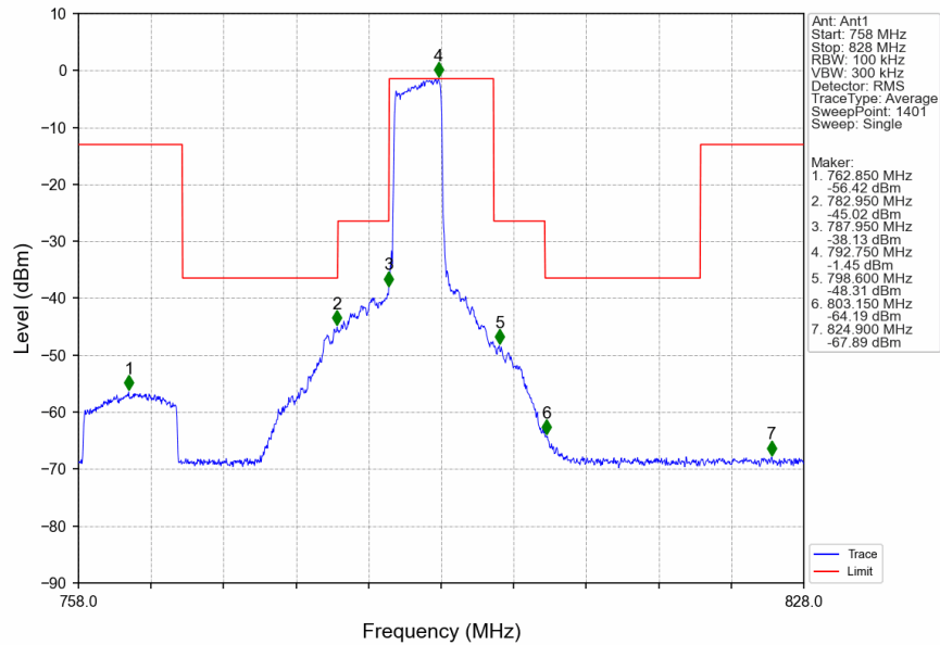
Band14_10MHz_256QAM_MCH_793MHz_RB_25_13_NTNV
