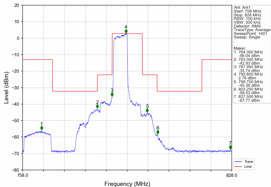
Band14_10MHz_QPSK_MCH_793MHz_RB_25_0_NTNV
