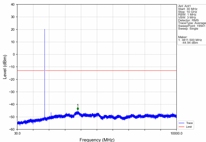
Band66_1.4MHz_QPSK_MCH_1745MHz_RB_1_0_NTNV
