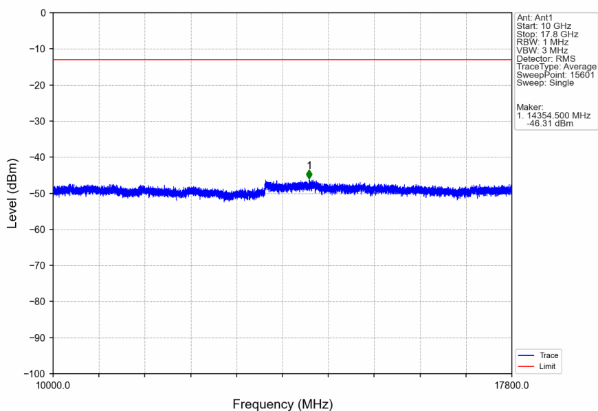
Band66_3MHz_QPSK_MCH_1745MHz_RB_1_0_NTNV
