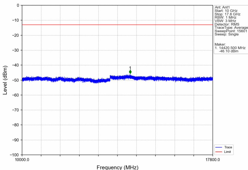
Band66_3MHz_QPSK_LCH_1711.5MHz_RB_15_0_NTNV
