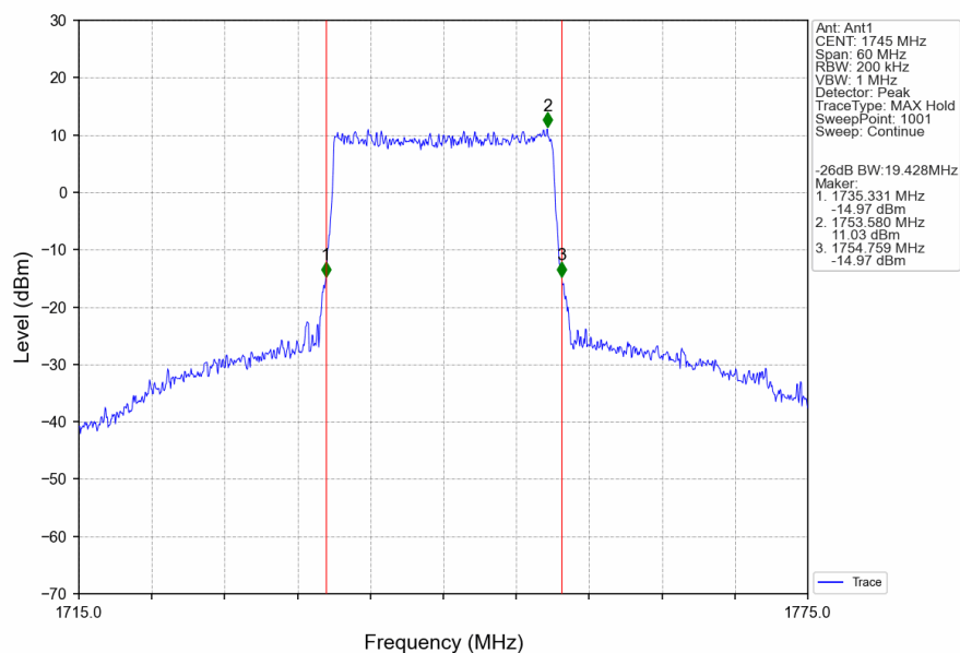
Band66_20MHz_16QAM_MCH_1745MHz_RB_100_0_NTNV
