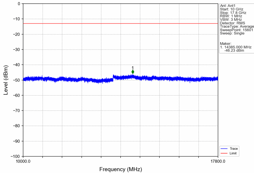
Band66_1.4MHz_QPSK_LCH_1710.7MHz_RB_6_0_NTNV
