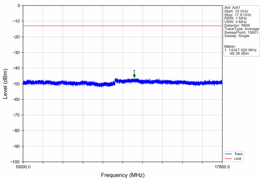
Band66_3MHz_QPSK_HCH_1778.5MHz_RB_1_0_NTNV
