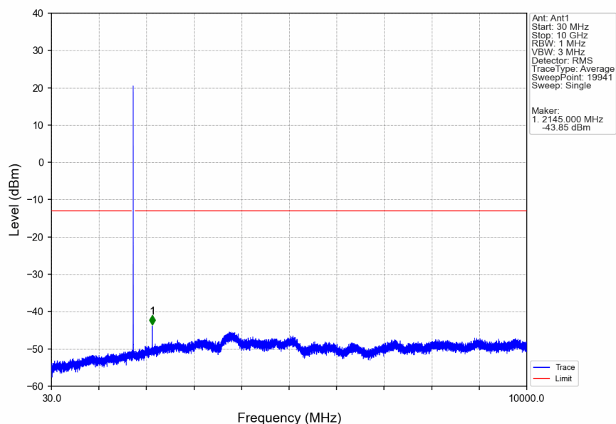
Band66_3MHz_QPSK_MCH_1745MHz_RB_1_0_NTNV
