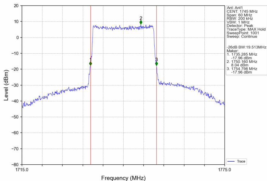
Band66_20MHz_256QAM_MCH_1745MHz_RB_100_0_NTNV
