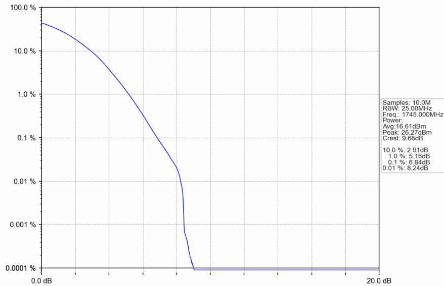
Band66_20MHz_256QAM_MCH_1745MHz_RB_100_0_NTNV
