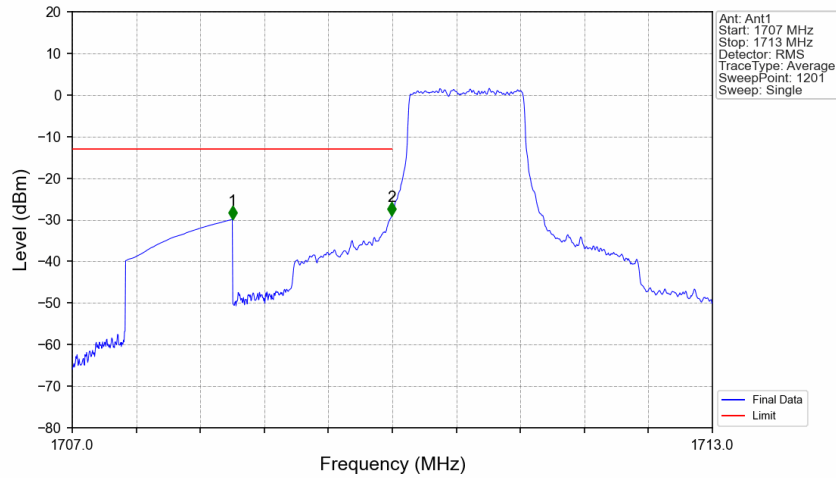
Band66_1.4MHz_QPSK_LCH_1710.7MHz_RB_6_0_NTNV
