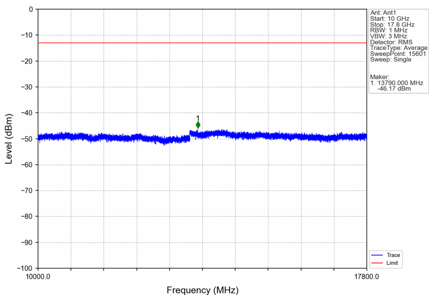
Band66_1.4MHz_QPSK_MCH_1745MHz_RB_1_0_NTNV
