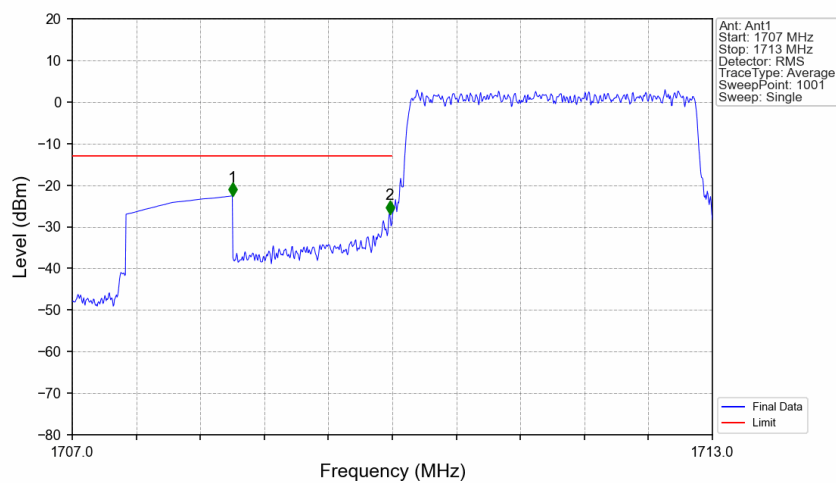
Band66_3MHz_QPSK_LCH_1711.5MHz_RB_15_0_NTNV
