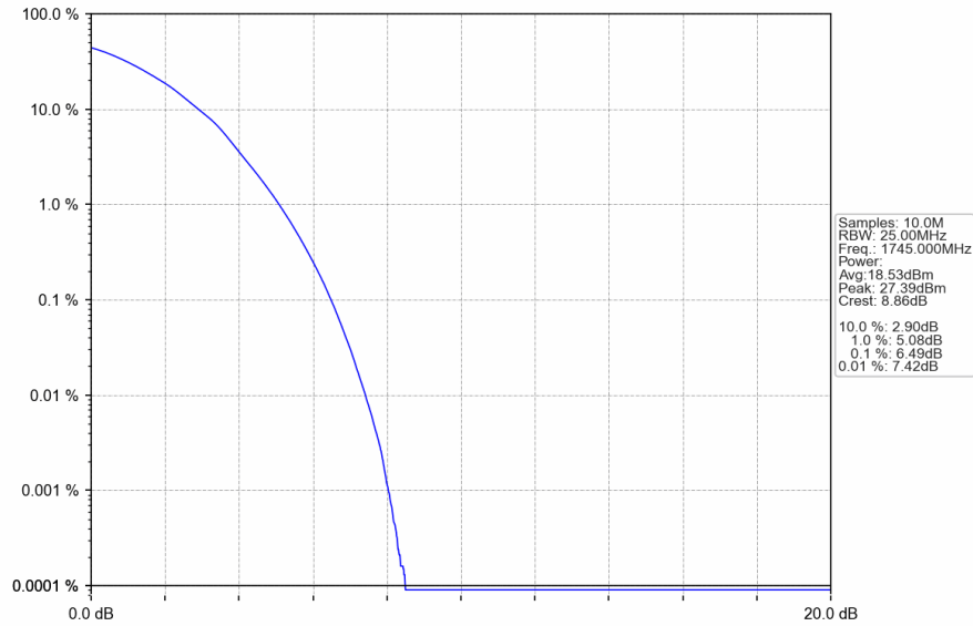
Band66_20MHz_64QAM_MCH_1745MHz_RB_100_0_NTNV
