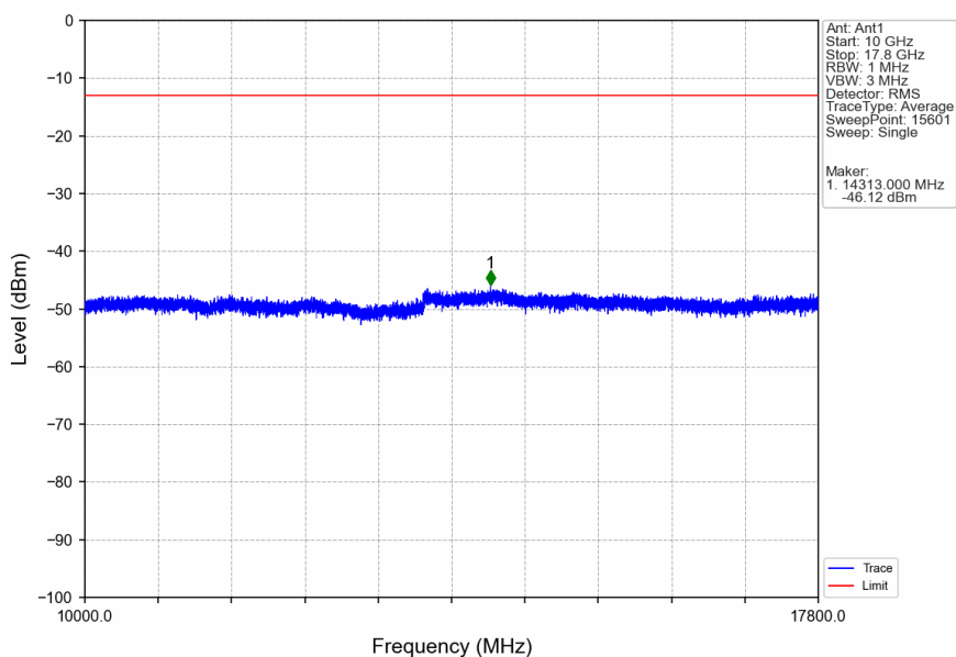
Band66_5MHz_QPSK_HCH_1777.5MHz_RB_1_0_NTNV
