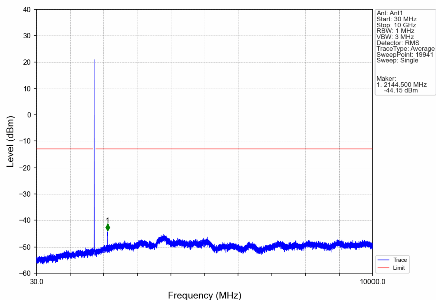
Band66_5MHz_QPSK_MCH_1745MHz_RB_1_0_NTNV
