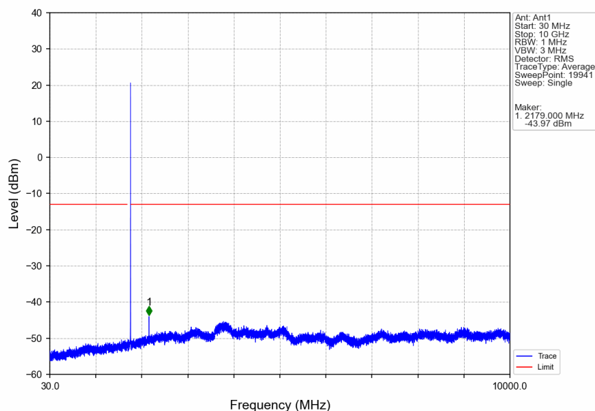
Band66_3MHz_QPSK_HCH_1778.5MHz_RB_1_0_NTNV
