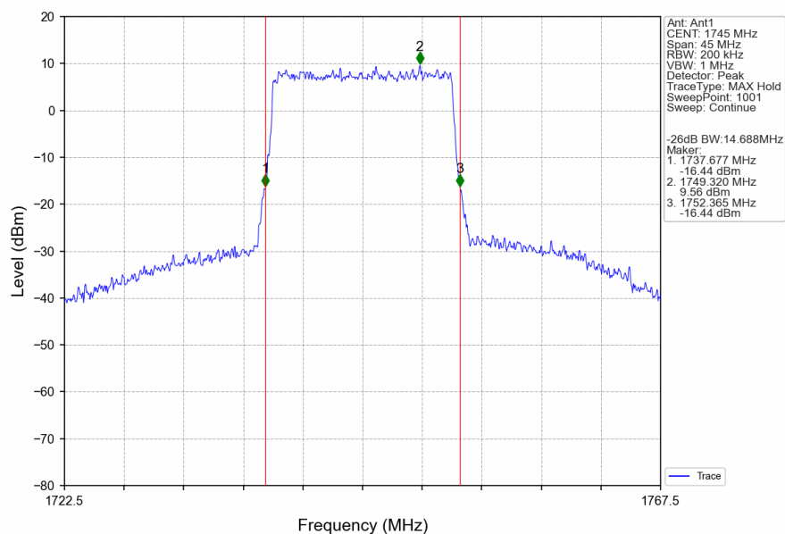
Band66_15MHz_256QAM_MCH_1745MHz_RB_75_0_NTNV
