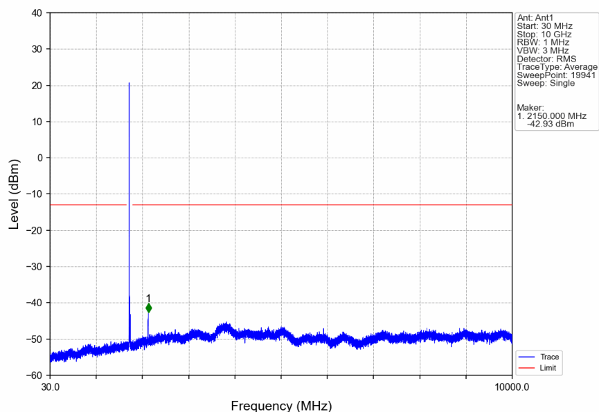
Band66_15MHz_QPSK_MCH_1745MHz_RB_1_0_NTNV
