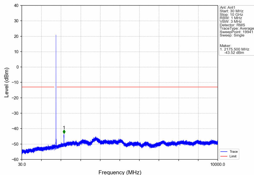
Band66_15MHz_QPSK_HCH_1772.5MHz_RB_1_0_NTNV
