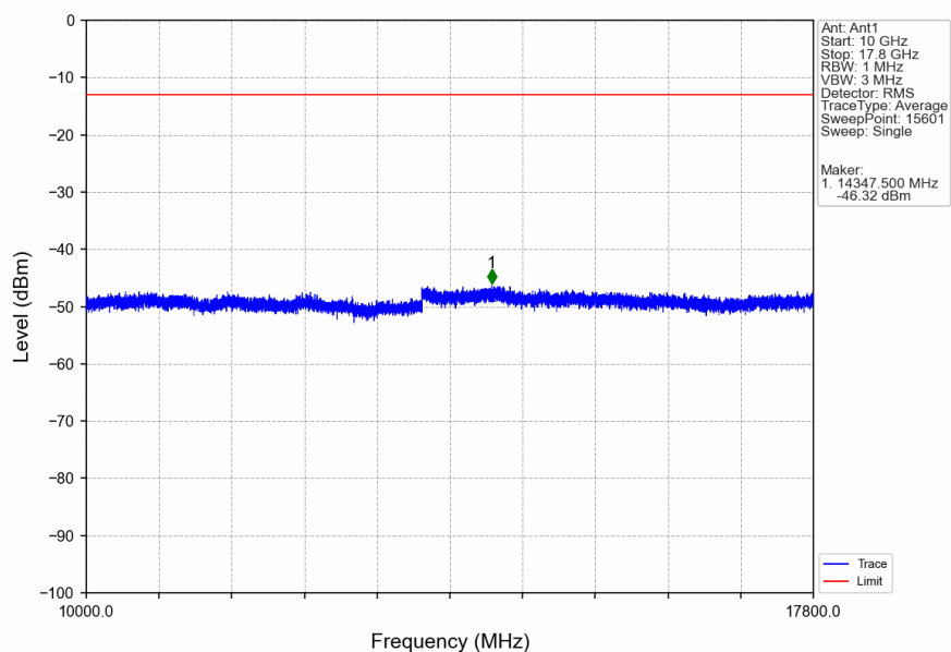
Band66_15MHz_QPSK_HCH_1772.5MHz_RB_1_0_NTNV
