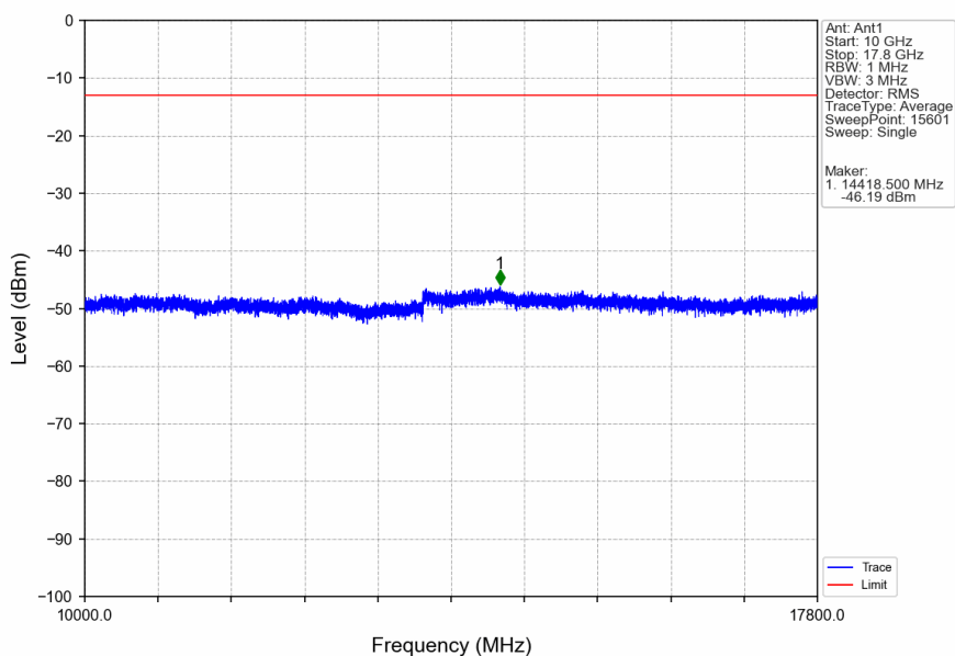
Band66_10MHz_QPSK_MCH_1745MHz_RB_1_0_NTNV
