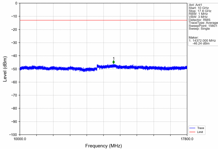
Band66_10MHz_QPSK_LCH_1715MHz_RB_50_0_NTNV
