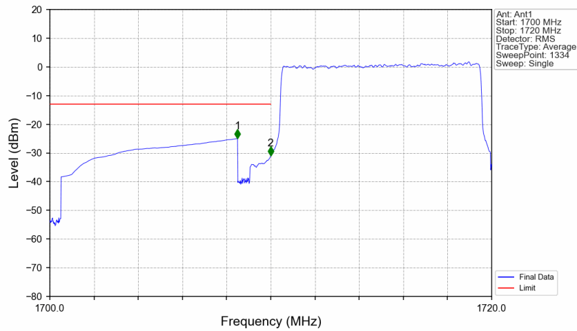
Band66_10MHz_QPSK_LCH_1715MHz_RB_50_0_NTNV
