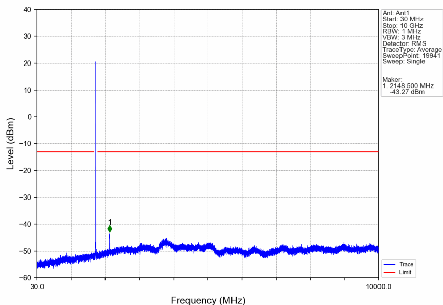
Band66_10MHz_QPSK_MCH_1745MHz_RB_1_0_NTNV
