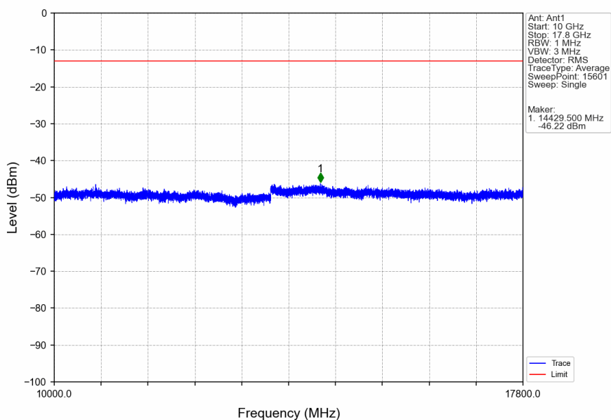
Band66_15MHz_QPSK_MCH_1745MHz_RB_1_0_NTNV
