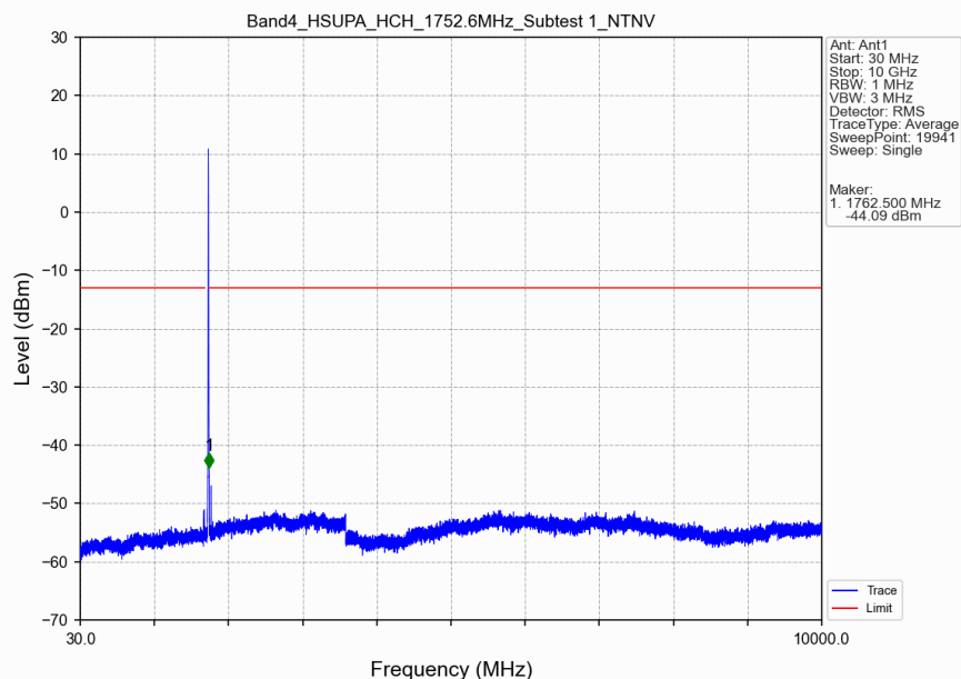
Band4_HSUPA_HCH_1752.6MHz_Subtest 1_NTNV
