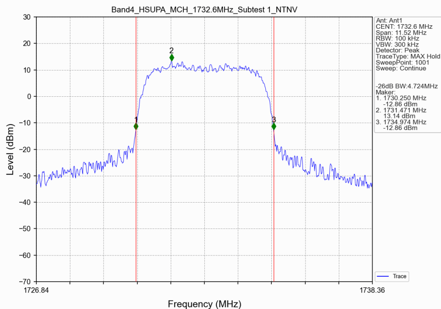
Band4_HSUPA_MCH_1732.6MHz_Subtest 1_NTNV
