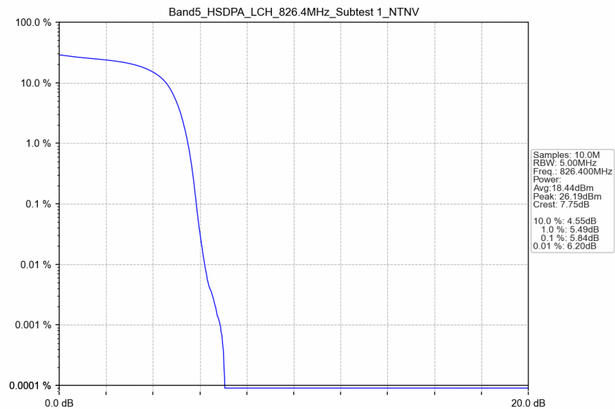
Band5_HSDPA_LCH_826.4MHz_Subtest 1_NTNV
