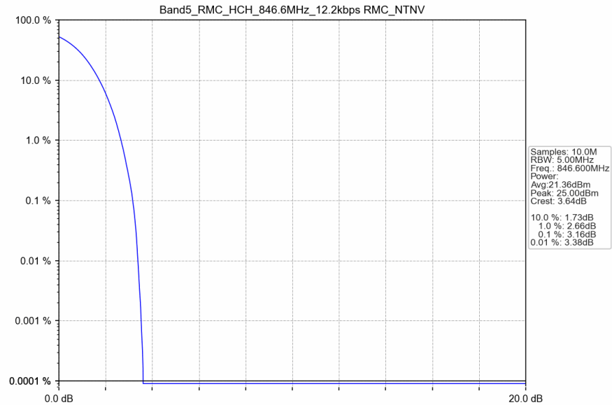
Band5_RMC_HCH_846.6MHz_12.2kbps RMC_NTNV
