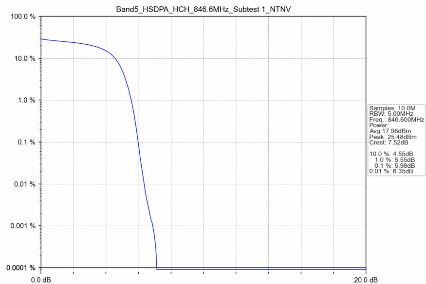
Band5_HSDPA_HCH_846.6MHz_Subtest 1_NTNV
