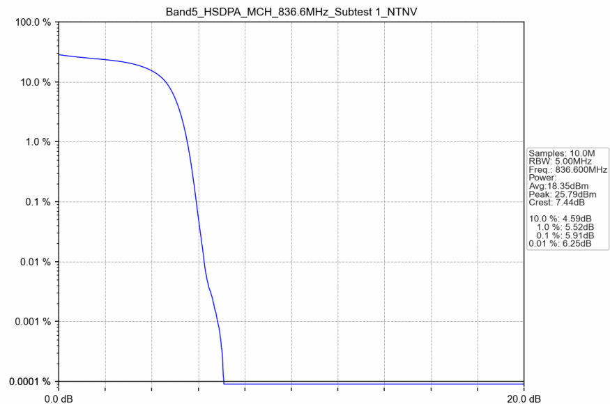
Band5_HSDPA_MCH_836.6MHz_Subtest 1_NTNV
