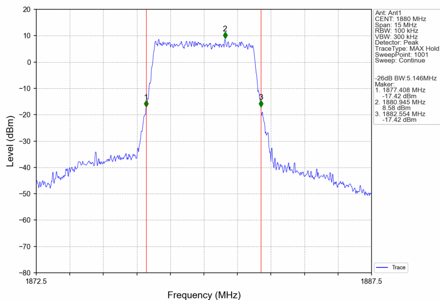
Band2_5MHz_256QAM_MCH_1880MHz_RB_25_0_NTNV
