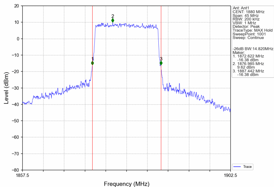
Band2_15MHz_16QAM_MCH_1880MHz_RB_75_0_NTNV
