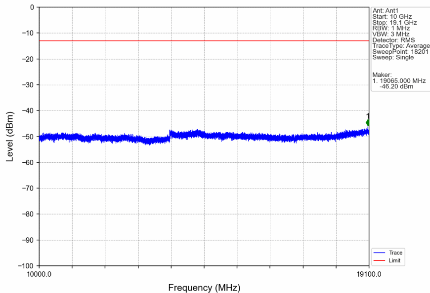
Band2_3MHz_QPSK_LCH_1851.5MHz_RB_15_0_NTNV
