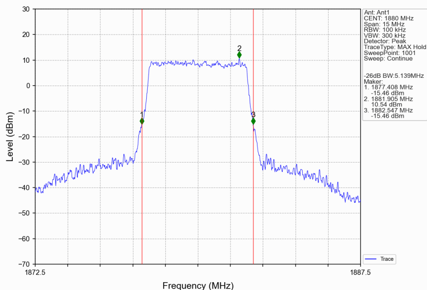
Band2_5MHz_256QAM_MCH_1880MHz_RB_25_0_NTNV
