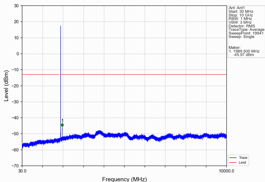
Band2_5MHz_QPSK_HCH_1907.5MHz_RB_1_0_NTNV
