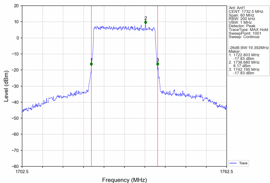
Band4_20MHz_256QAM_MCH_1732.5MHz_RB_100_0_NTNV
