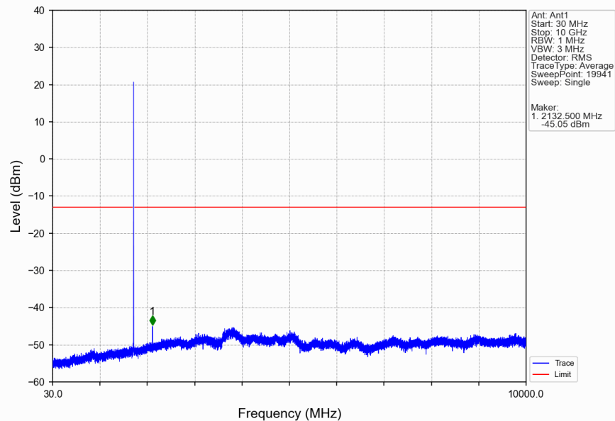
Band4_1.4MHz_QPSK_MCH_1732.5MHz_RB_1_0_NTNV
