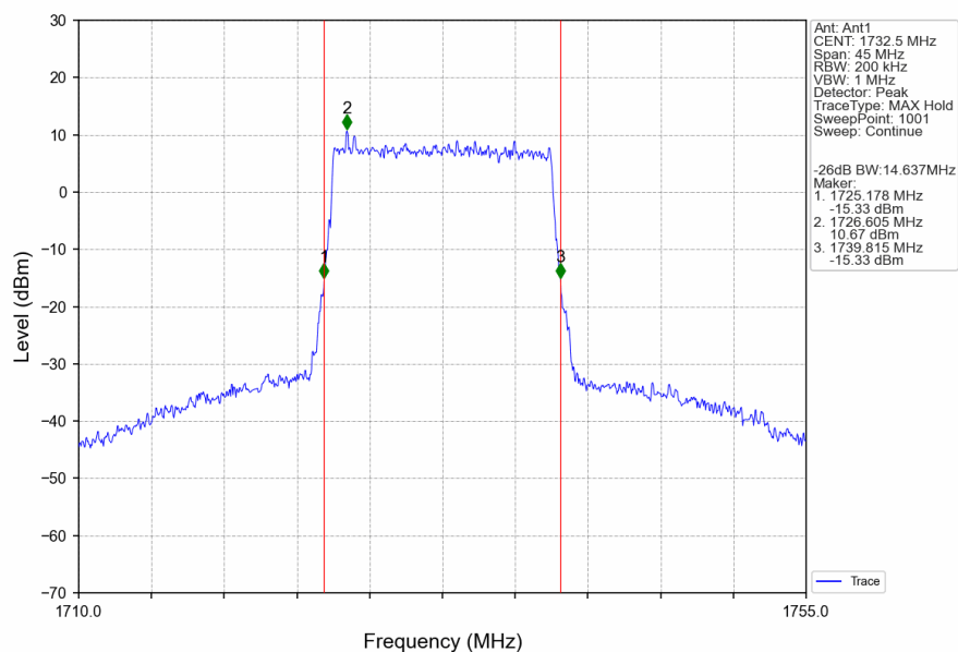
Band4_15MHz_256QAM_MCH_1732.5MHz_RB_75_0_NTNV
