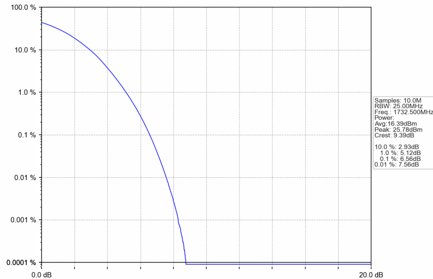
Band4_20MHz_256QAM_MCH_1732.5MHz_RB_100_0_NTNV
