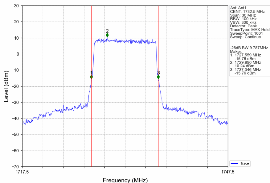
Band4_10MHz_256QAM_MCH_1732.5MHz_RB_50_0_NTNV
