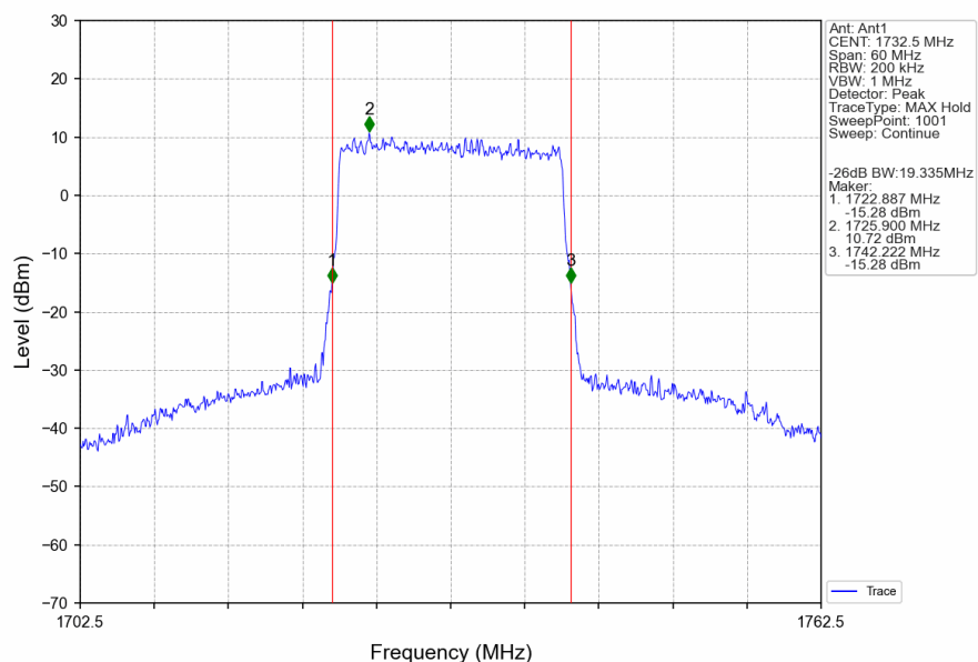
Band4_20MHz_256QAM_MCH_1732.5MHz_RB_100_0_NTNV
