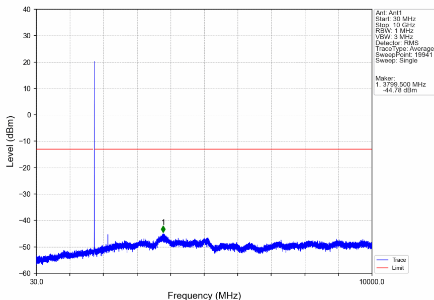
Band4_1.4MHz_QPSK_HCH_1754.3MHz_RB_1_0_NTNV
