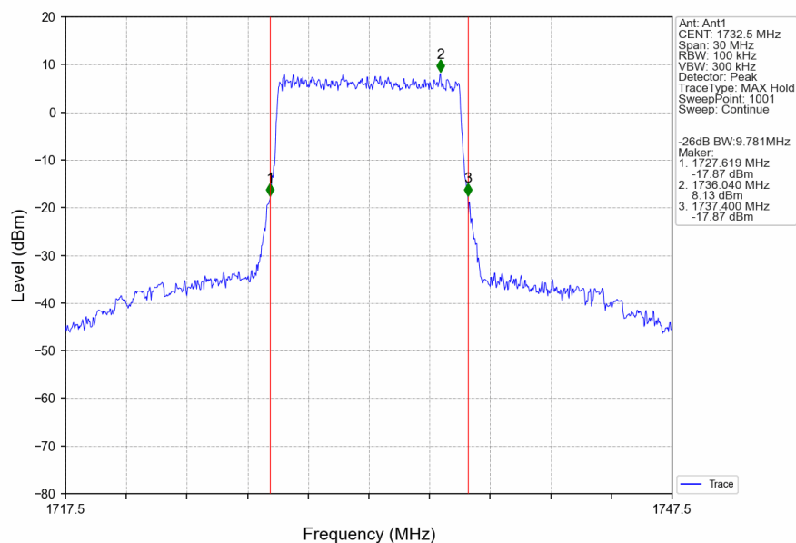
Band4_10MHz_256QAM_MCH_1732.5MHz_RB_50_0_NTNV
