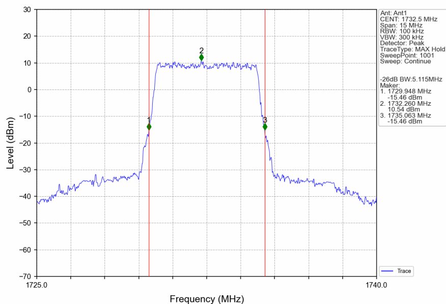
Band4_5MHz_256QAM_MCH_1732.5MHz_RB_25_0_NTNV
