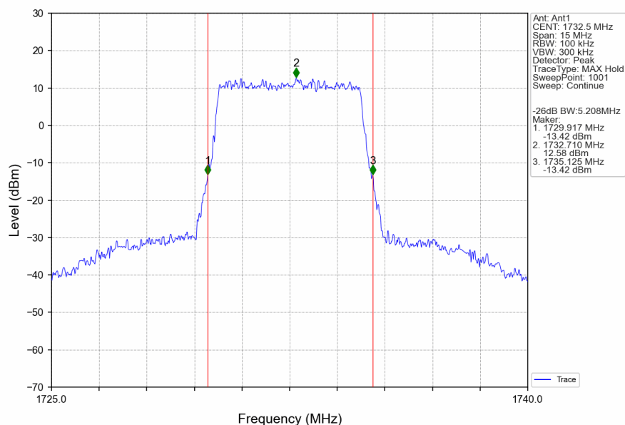
Band4_5MHz_256QAM_MCH_1732.5MHz_RB_25_0_NTNV
