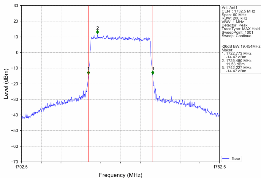
Band4_20MHz_16QAM_MCH_1732.5MHz_RB_100_0_NTNV
