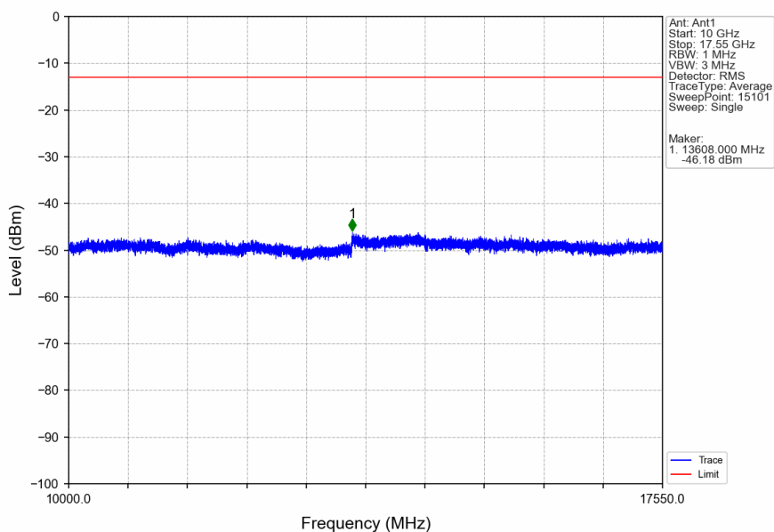
Band4_10MHz_QPSK_MCH_1732.5MHz_RB_1_0_NTNV
