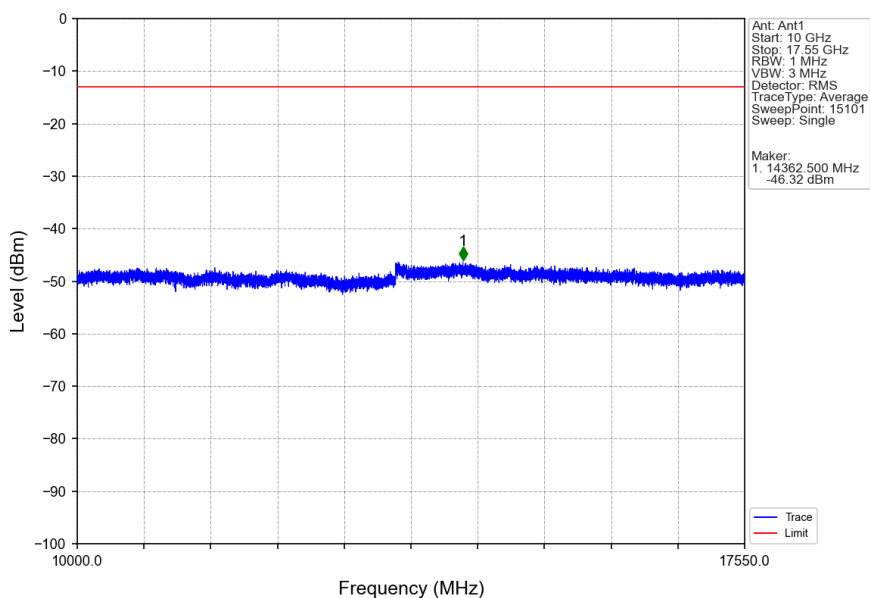
Band4_15MHz_QPSK_MCH_1732.5MHz_RB_1_0_NTNV
