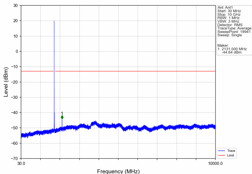
Band4_10MHz_QPSK_MCH_1732.5MHz_RB_1_0_NTNV
