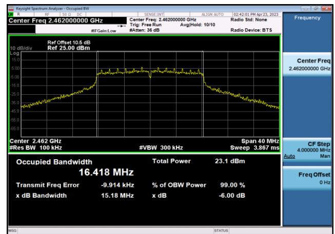
6dB Bandwidth-802.11g,2462MHz,Ant0
