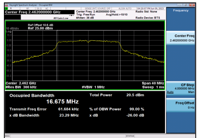
99% Bandwidth-802.11g,2462MHz,Ant0
