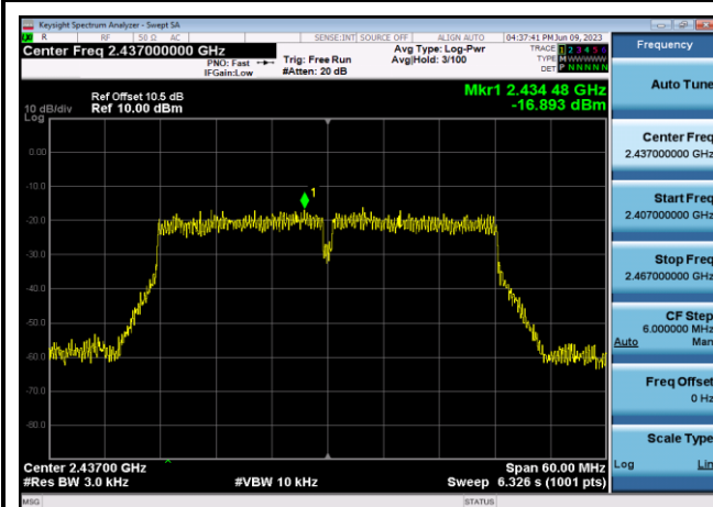
Power spectral density-802.11n(HT40) ,2437MHz,Ant0
