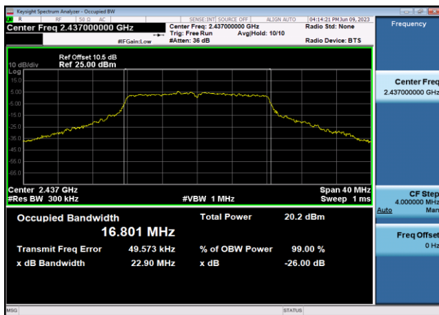
99% Bandwidth-802.11g,2437MHz,Ant0
