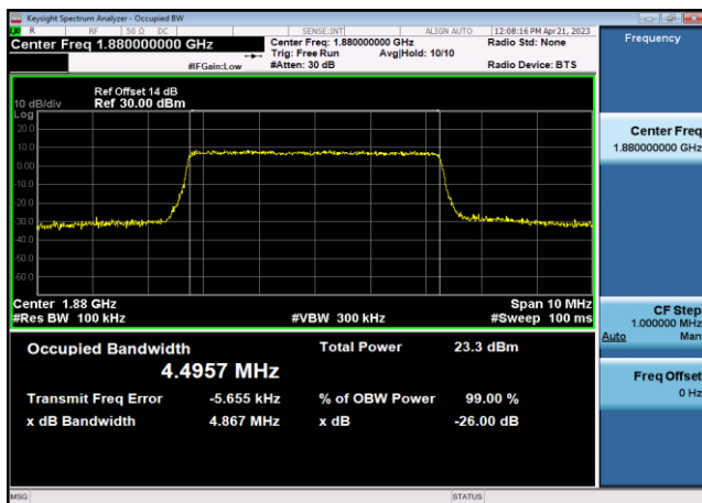
FDD02_MidRange_5_1880_QPSK
