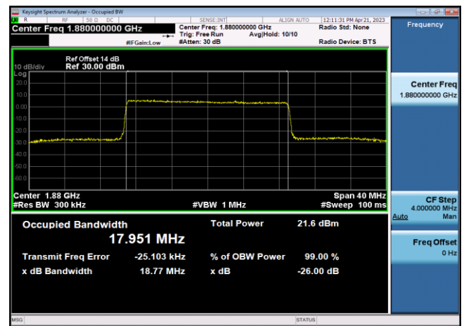
FDD02_MidRange_20_1880_Q16
