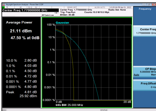
FDD66_HighRange_20MHz_1770_OneRB _high_Q16
