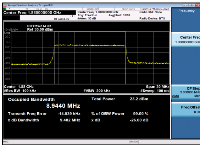
FDD02_MidRange_15_1880_QPSK
