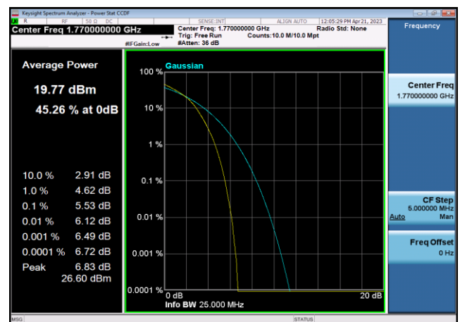
FDD66_HighRange_20MHz_1770_fullRB _Q16
