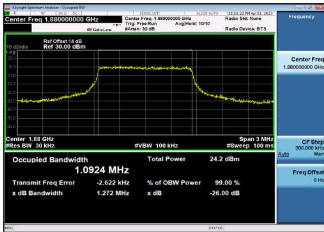
FDD02_MidRange_3_1880_QPSK
