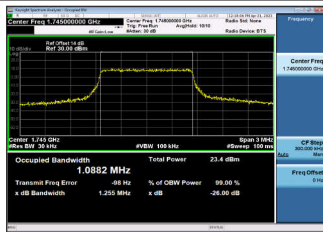
FDD66_MidRange_1.4_1745_QPSK
