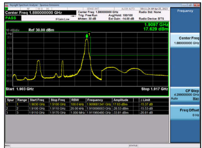
FDD2-5MHz-16QAM-HCH-25RB#0
