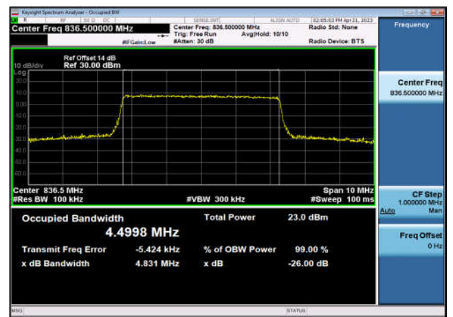
FDD05_MidRange_5_836.5_Q16
