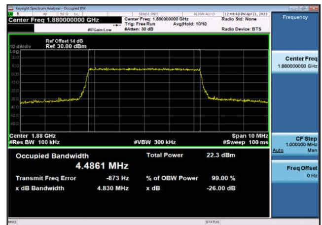
FDD02_MidRange_5_1880_Q16
