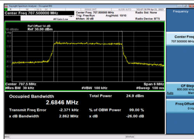
FDD12_MidRange_3_707.5_QPSK
