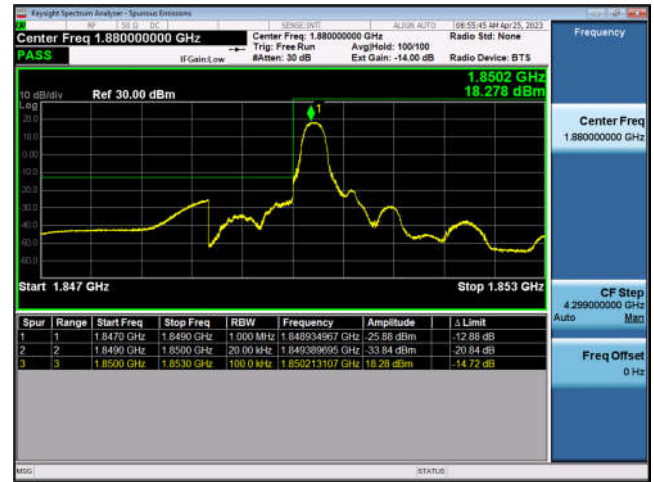
FDD2-1.4MHz-16QAM-LCH-6RB#0
