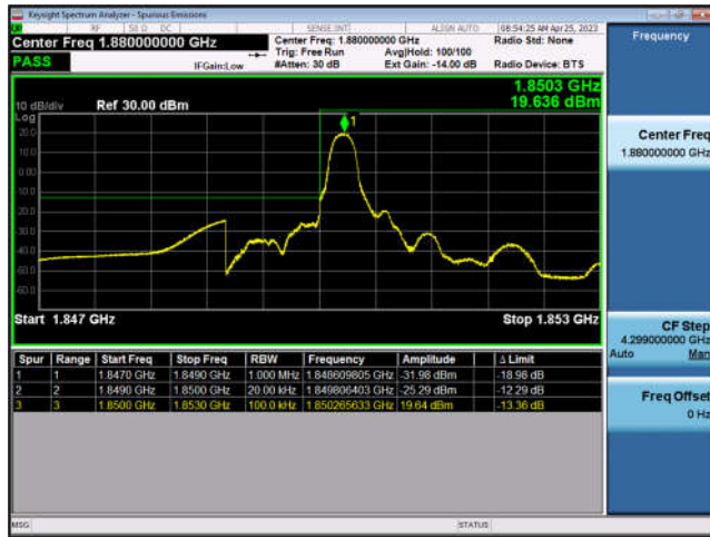
FDD2-1.4MHz-QPSK-LCH-6RB#0
