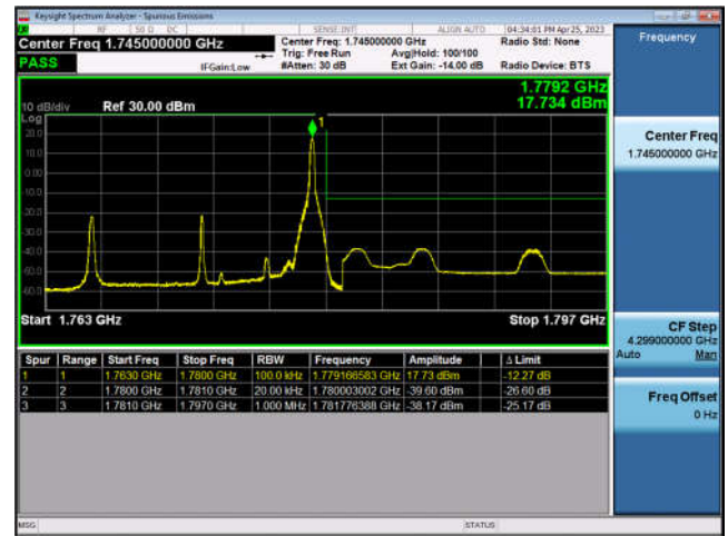
FDD66-15MHz-16QAM-HCH-75RB#0
