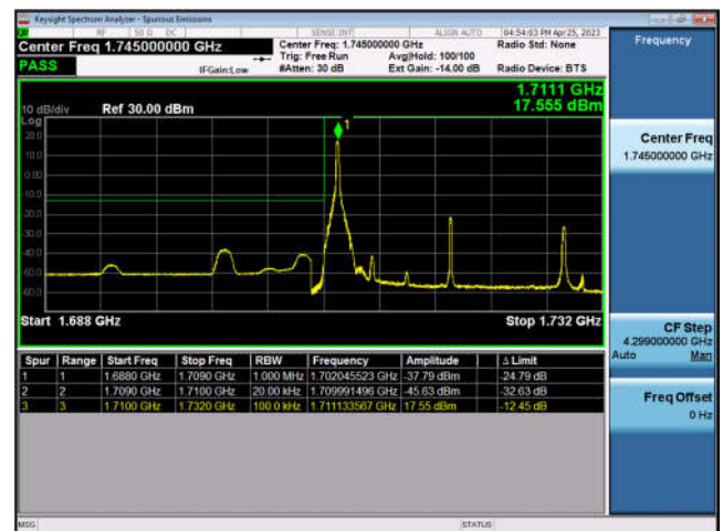
FDD66-20MHz-16QAM-LCH-1RB#0
