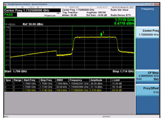
FDD4-3MHz-16QAM-LCH-15RB#0
