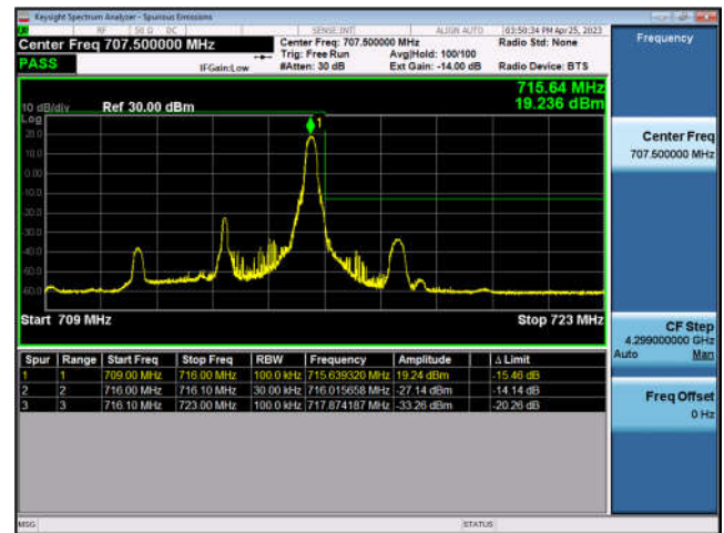
FDD12-5MHz-16QAM-HCH-25RB#0
