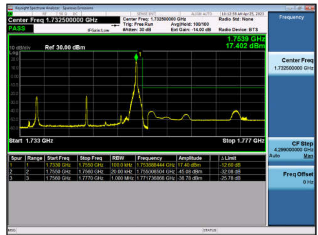
FDD4-20MHz-16QAM-HCH-100RB#0
