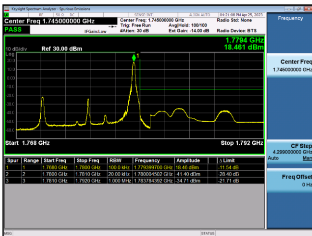
FDD66-10MHz-QPSK-HCH-1RB#49
