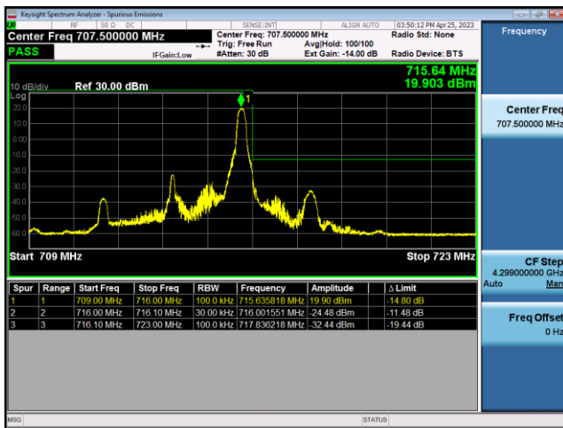
FDD12-5MHz-QPSK-HCH-25RB#0
