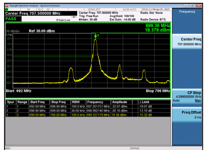
FDD12-5MHz-16QAM-LCH-1RB#0
