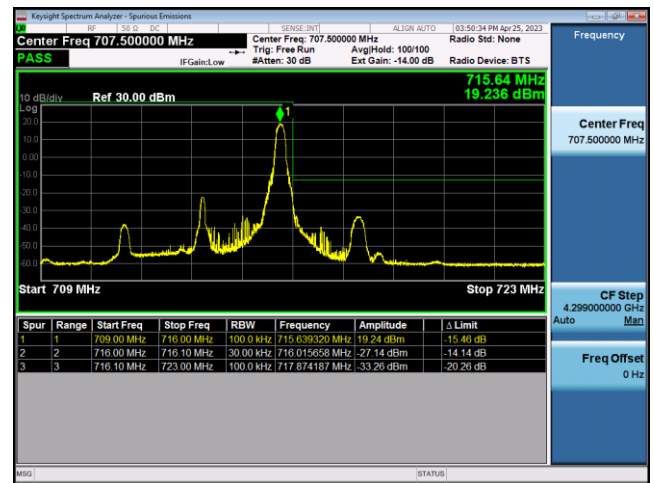
FDD12-5MHz-16QAM-HCH-25RB#0
