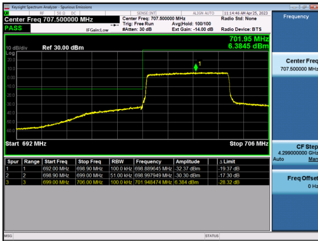
FDD12-5MHz-QPSK-HCH-1RB#24
