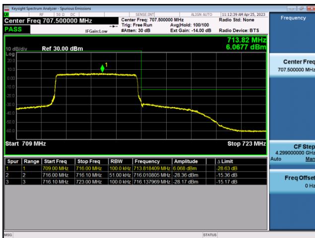
FDD12-5MHz-QPSK-HCH-25RB#0
