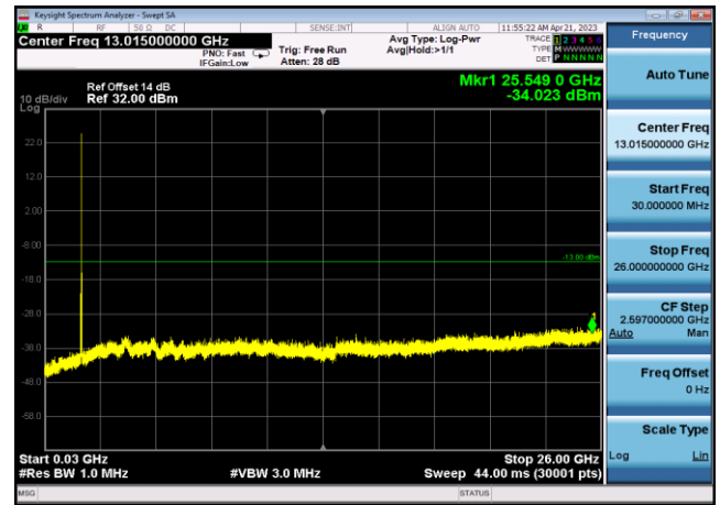
FDD66_MidRange_20MHz_30MHz~26GHz
