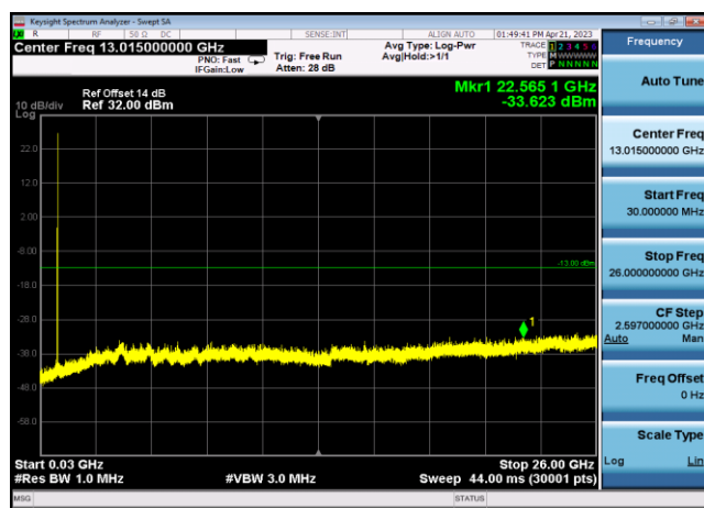
FDD12_MidRange_10MHz_30MHz~26GHz
