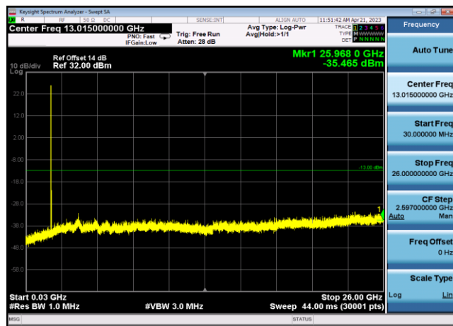
FDD02_HighRange_20MHz_30MHz~26GHz
