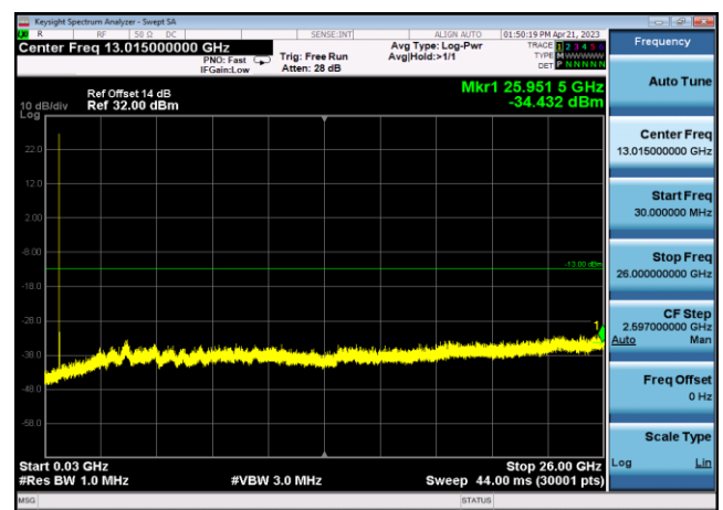
FDD12_HighRange_10MHz_30MHz~26GHz
