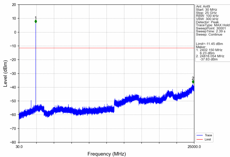
1M_LCH_2402MHz_Ant9_NTNV
