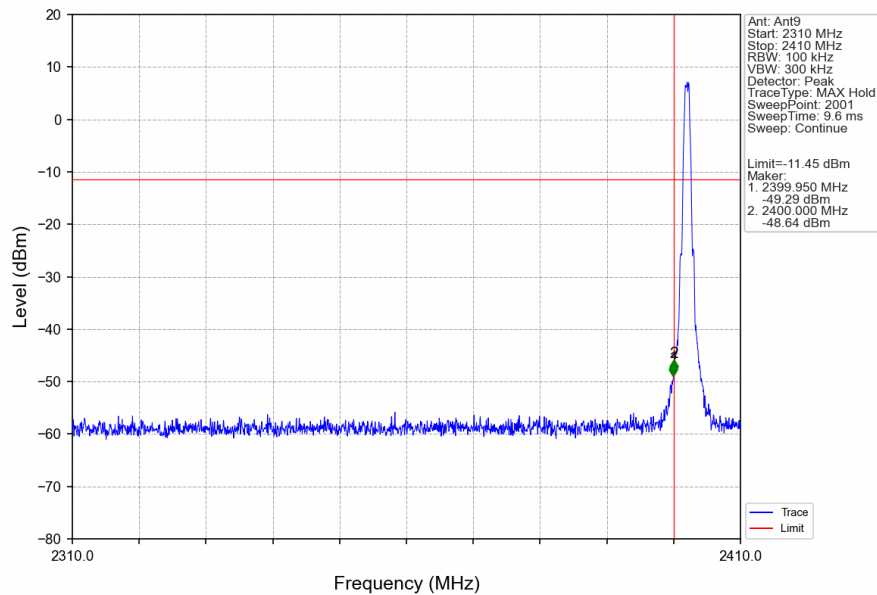
1M_LCH_2402MHz_Ant9_NTNV
