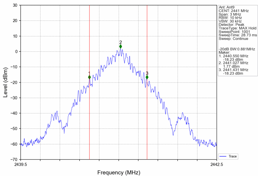
GFSK_DH5_MCH_2441MHz_Ant9_NTNV
