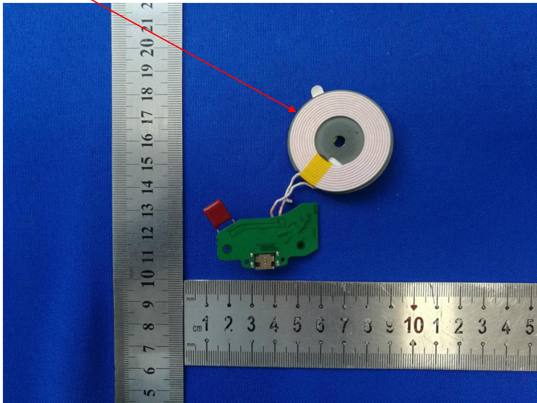
Coil Antenna:
