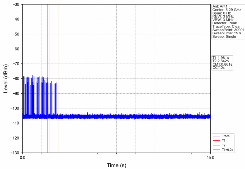
Channel Move Time and Closing Transmission Time_802.11ac_2A_5290MHz
