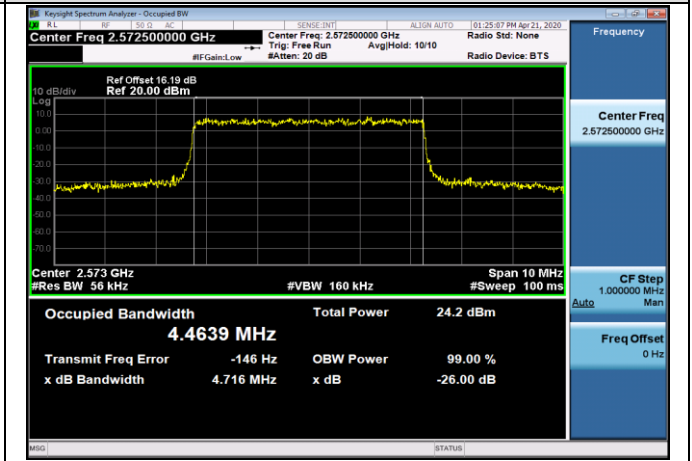
LCH_16QAM_25RB#0
