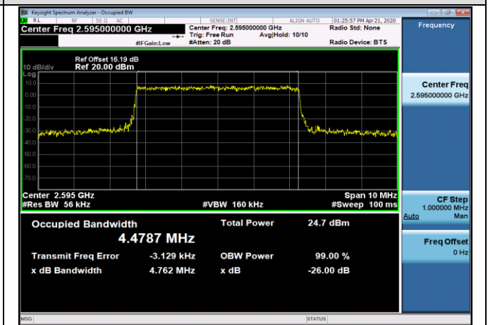
MCH_16QAM_25RB#0
