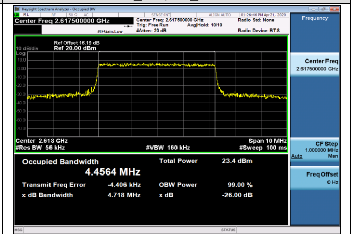
HCH_16QAM_25RB#0
