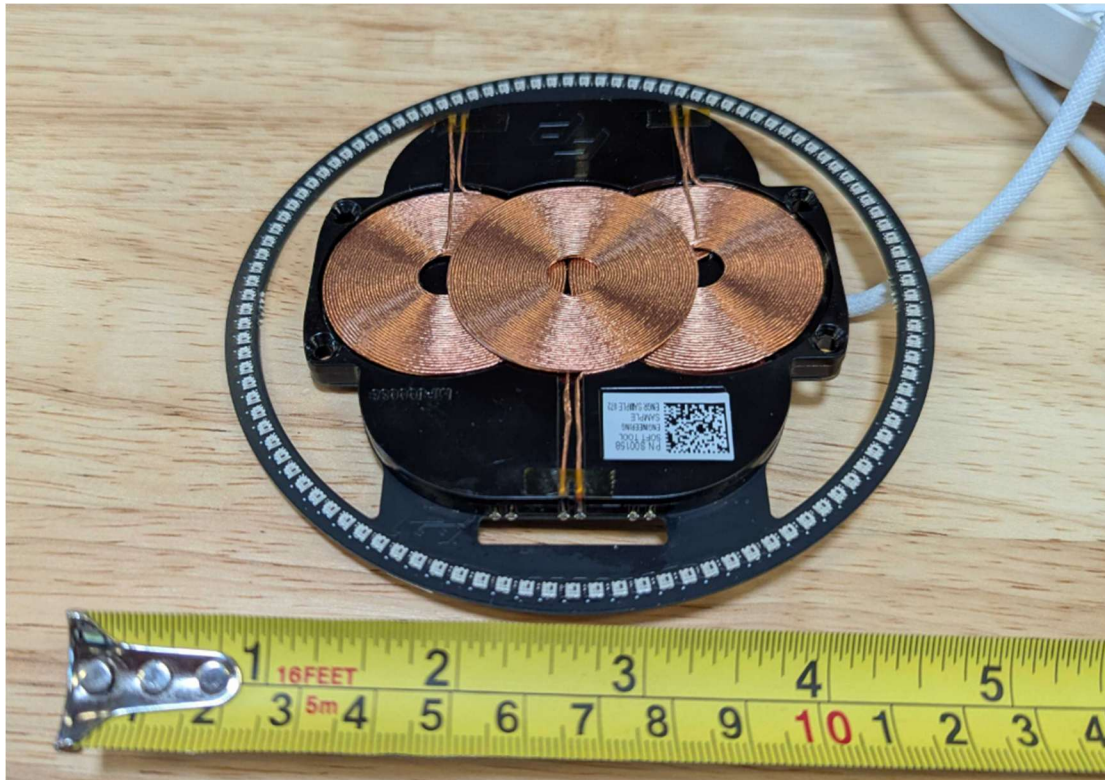
PCB Coil Array Top Side:
