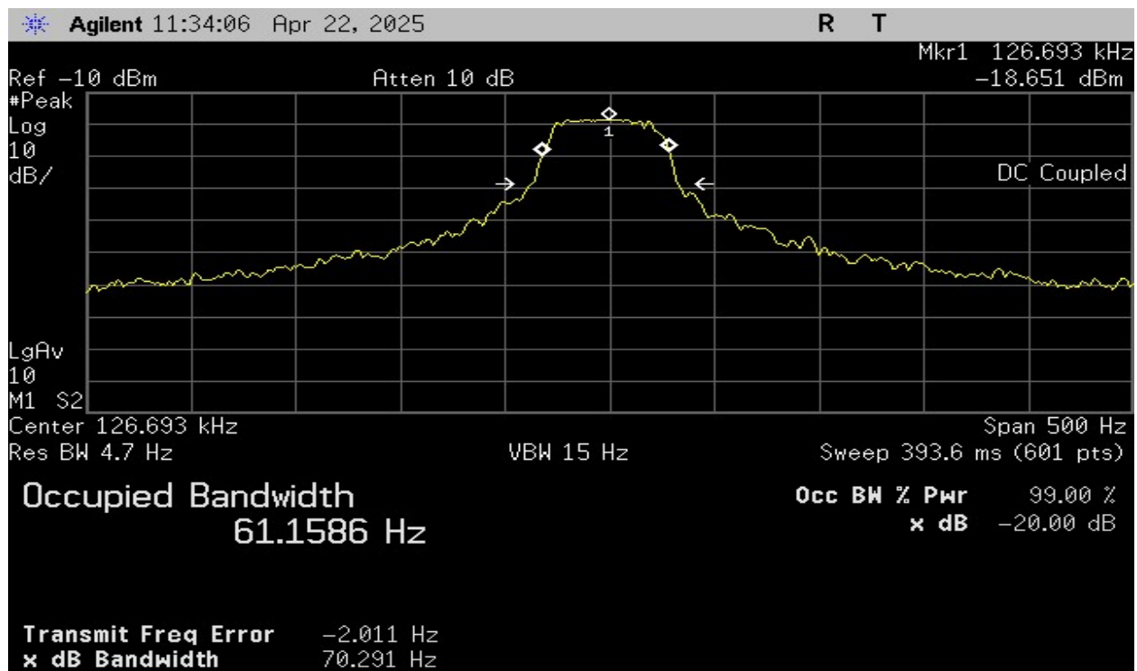
Plot 7 – 20dB BW – WPT Mode
