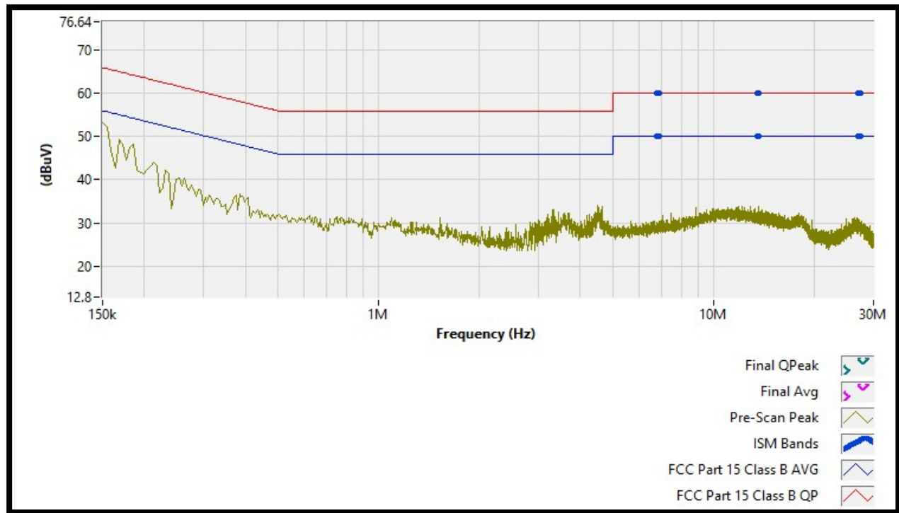
Plot 2 – Conducted Emission – Line Side (Idle Mode)
