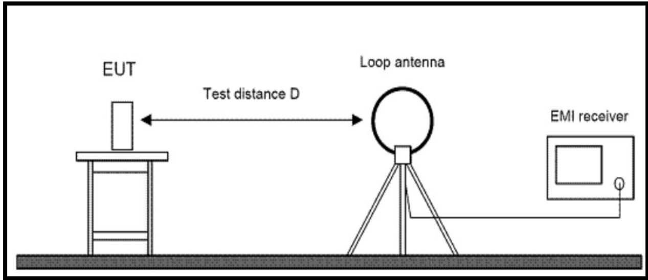
Figure 4. Radiated Emissions Test Setup (9kHz - 30MHz)
