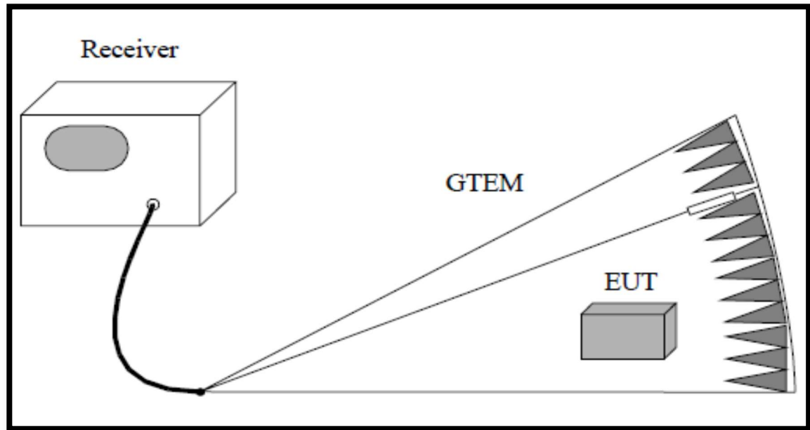
Figure 1. Radiated Emissions Test Setup (30MHz – 1GHz)
