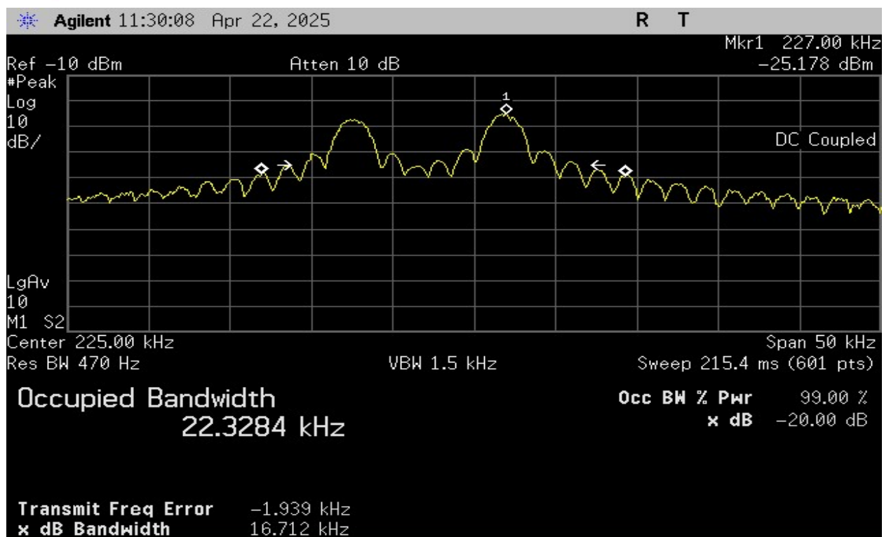
Plot 6 – 20dB BW – Idle Mode Analog Pings
