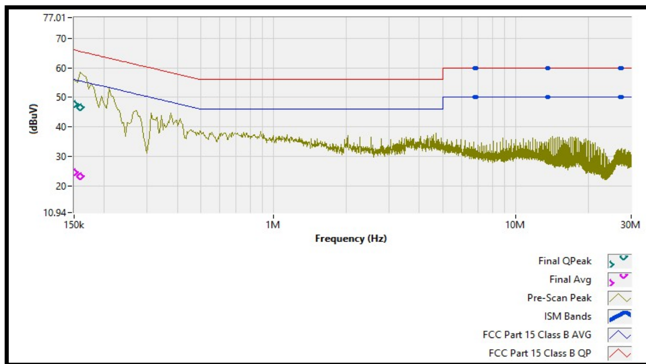
Plot 5 – Conducted Emissions – Neutral Side (WPT Mode)
