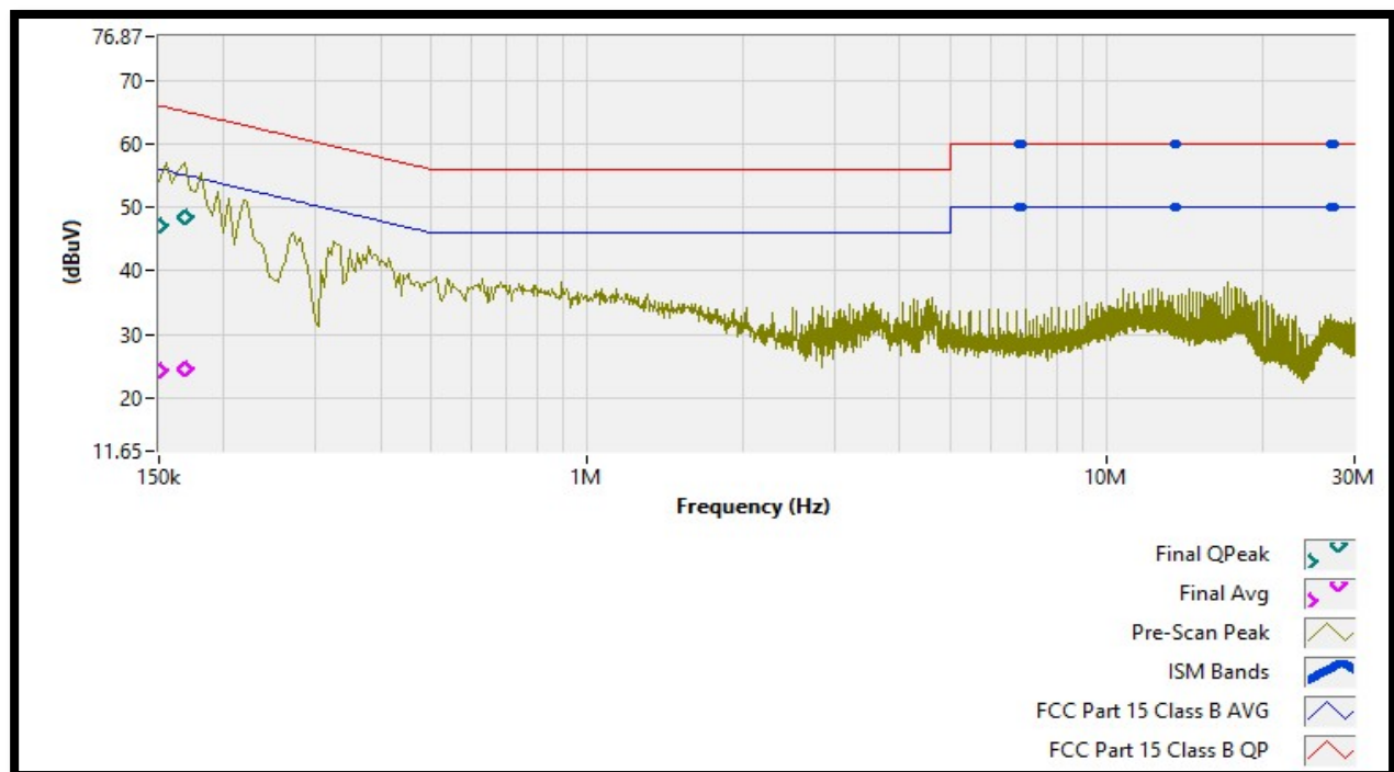
Plot 3 – Conducted Emission – Line Side (WPT Mode)
