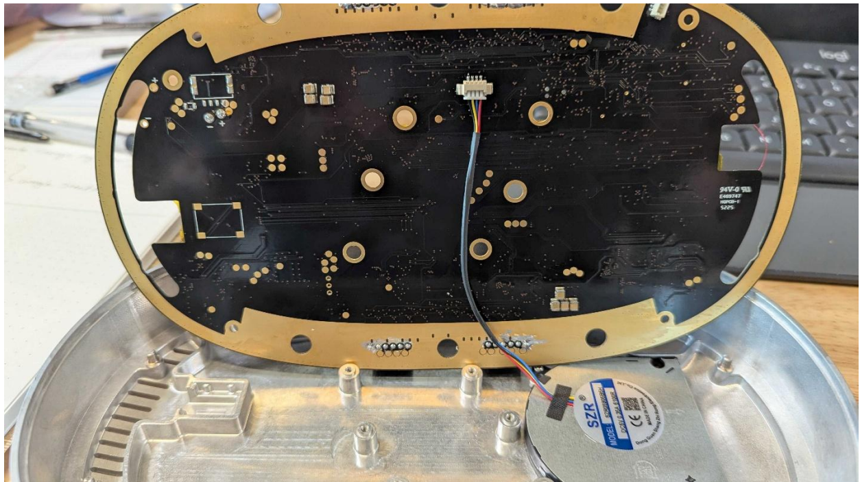
PCB Bottom Side
