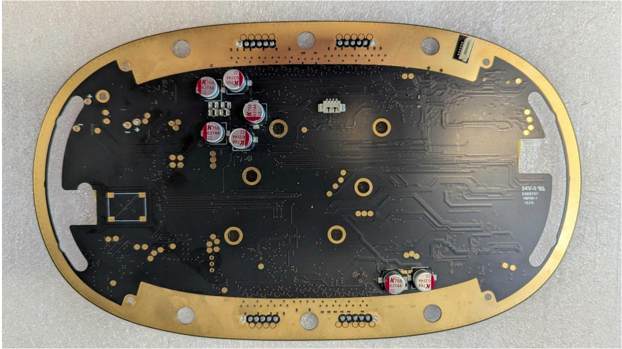
PCBA Bottom Side View
