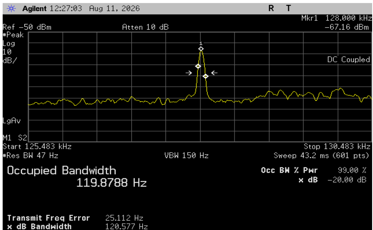
Plot 8 – 20dB BW – 5W WPT Mode
