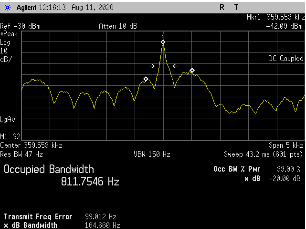
Plot 9 – 20dB BW – 25W WPT Mode
