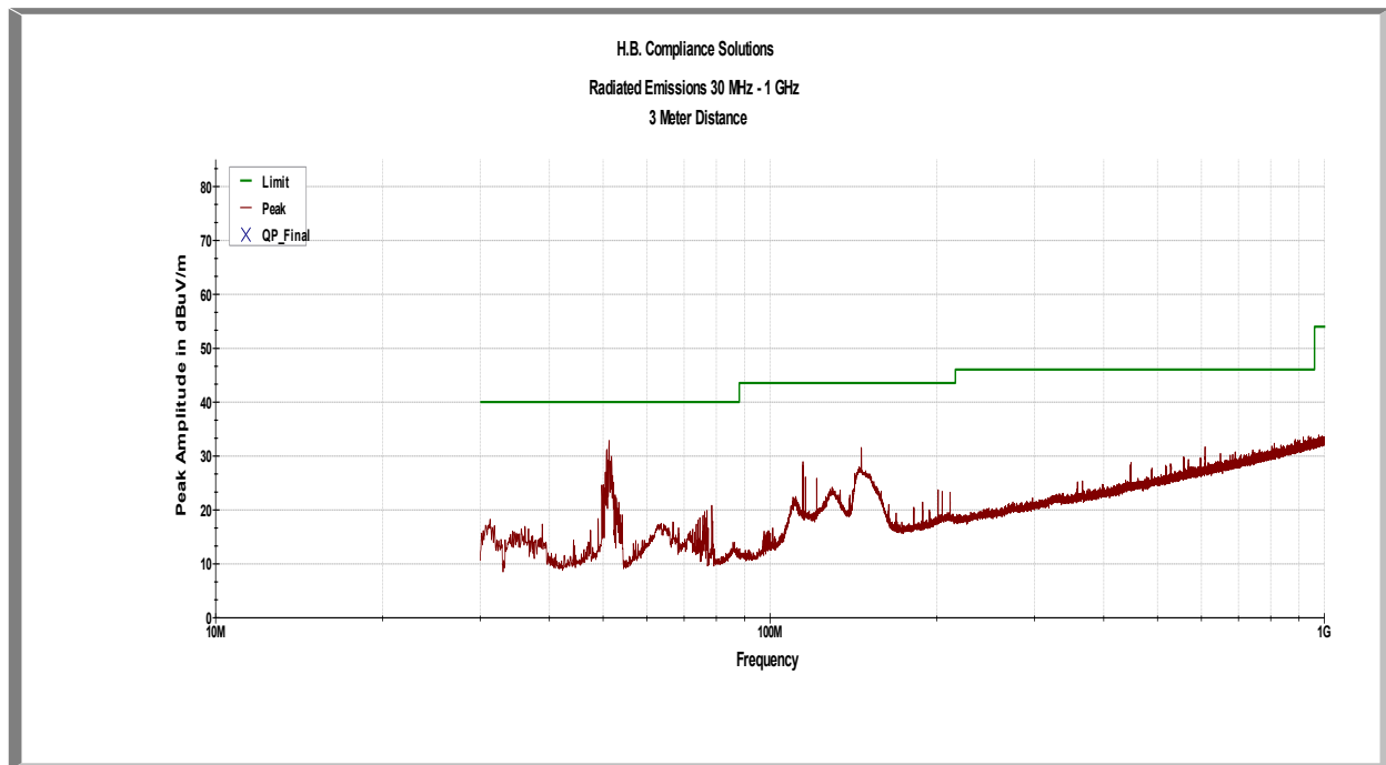
Plot 2 – Radiated Emissions – 30MHz to 1GHz – Idle Mode
