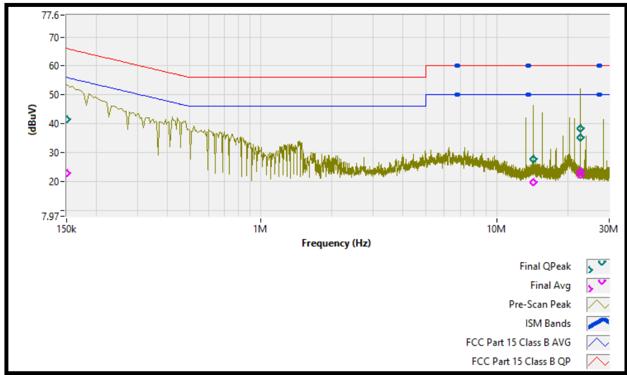
Plot 5 – Conducted Emissions – Neutral Side (Idle Mode)
