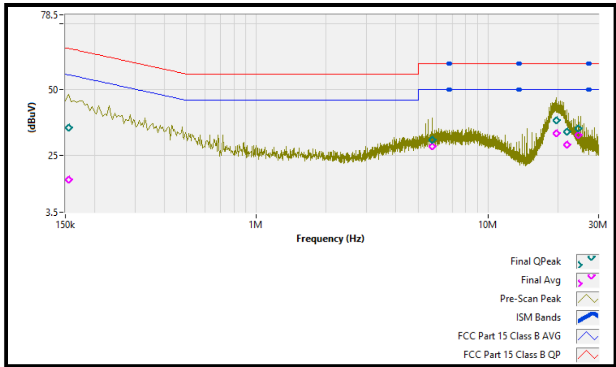
Plot 6 – Conducted Emissions – Neutral Side (WPT Mode)
