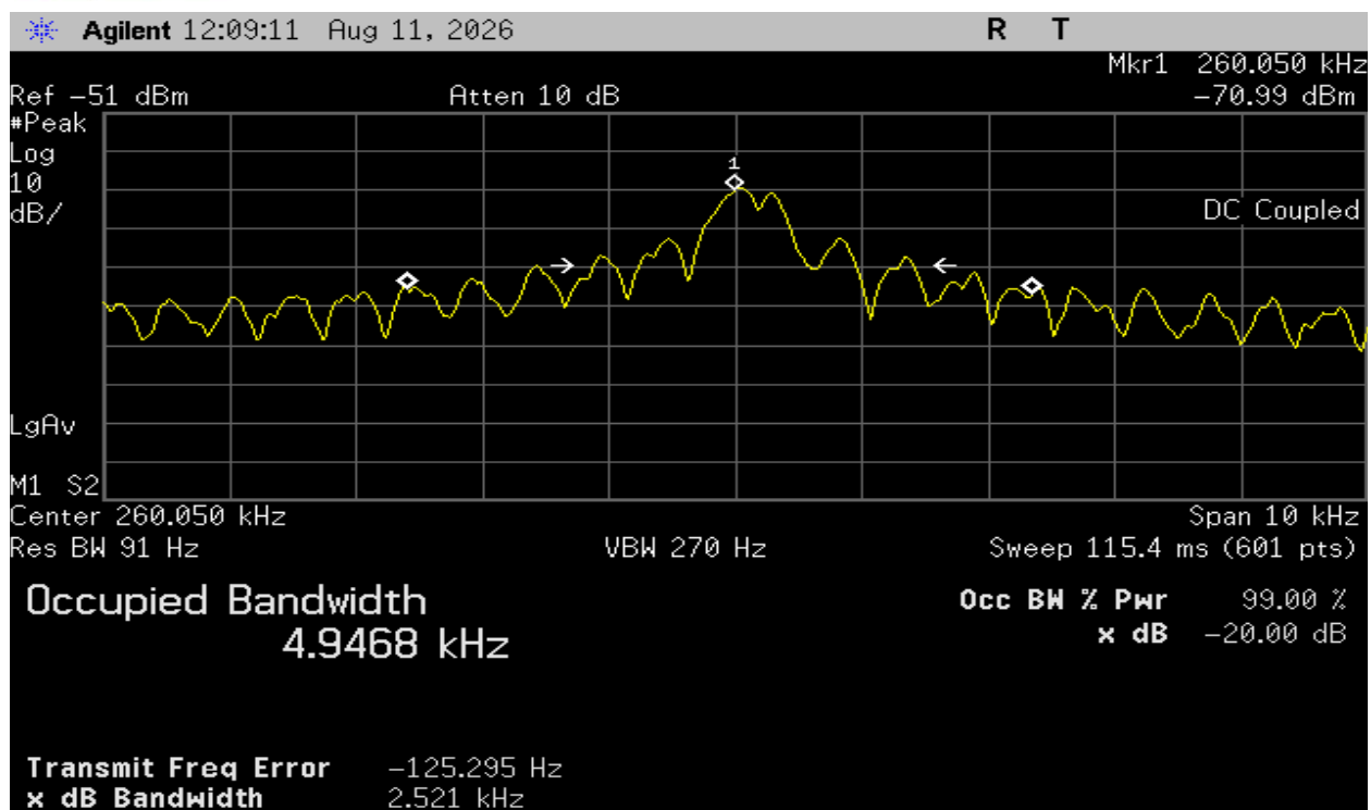
Plot 7 – 20dB BW – Idle Mode Analog Pings
