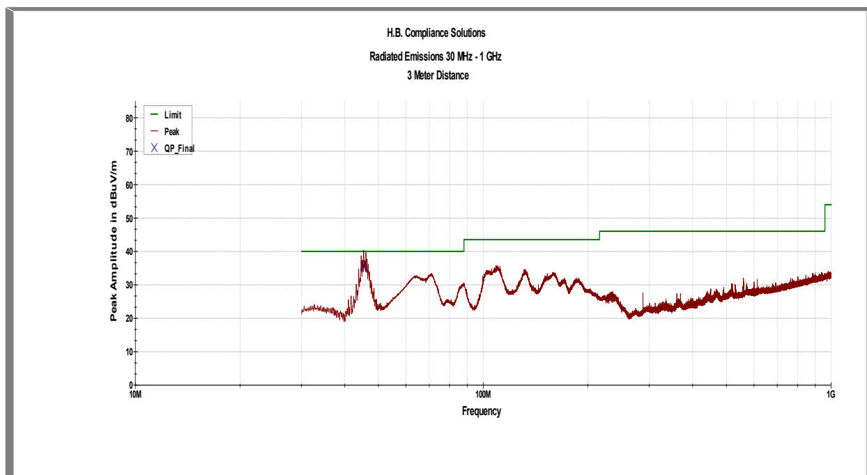
Plot 1 – Radiated Emissions – 30MHz to 1GHz – 25W MPP Mode
