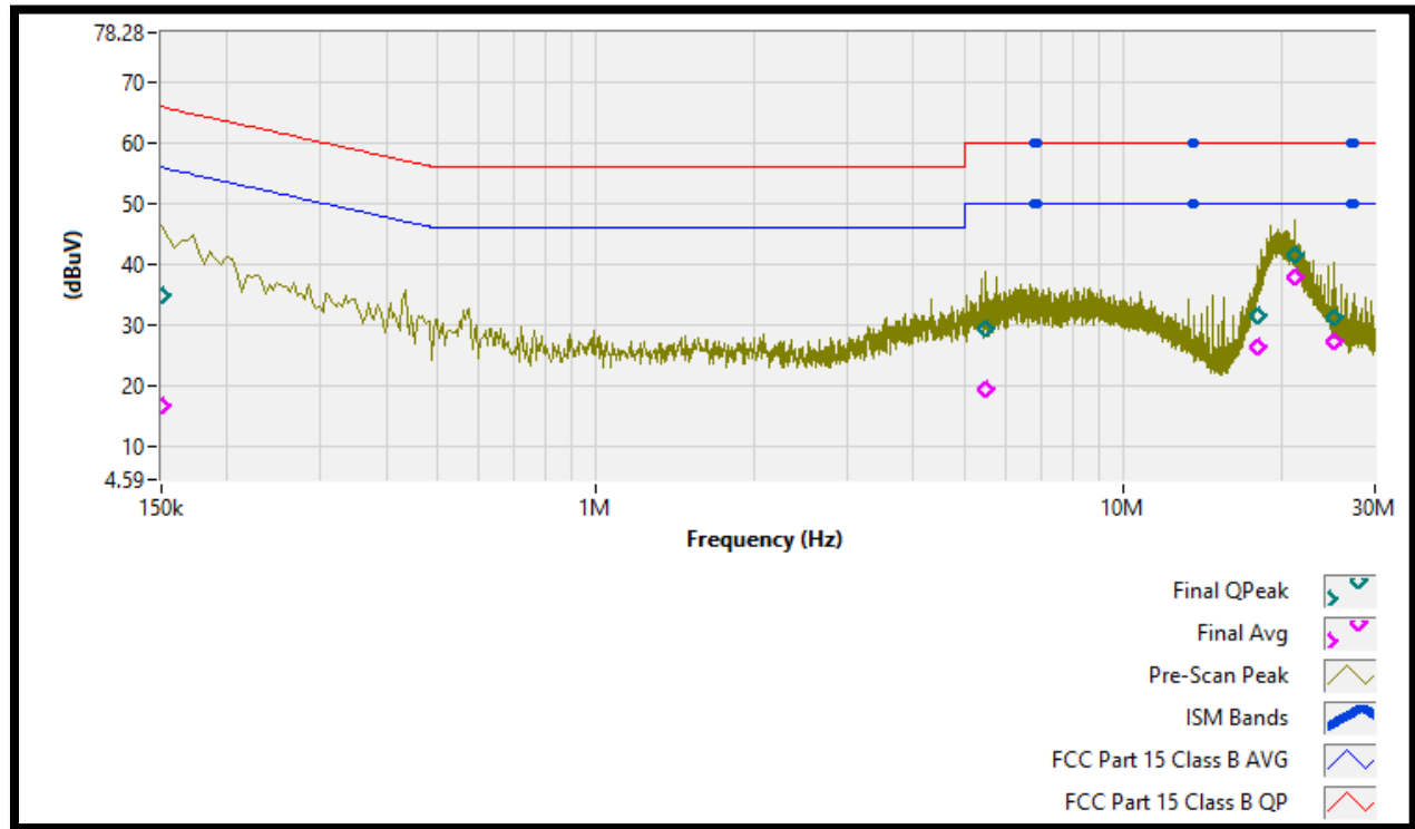
Plot 4 – Conducted Emission – Line Side (25W MPP Mode)
