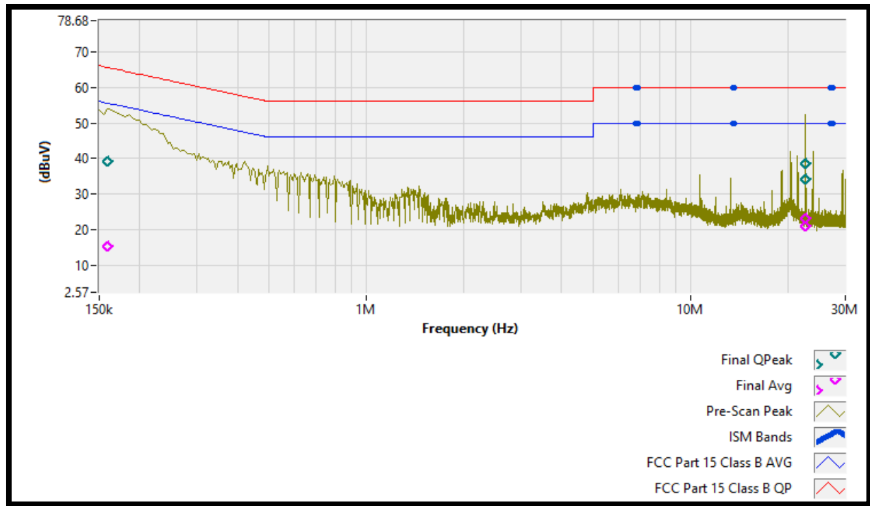
Plot 3 – Conducted Emission – Line Side (Idle Mode)
