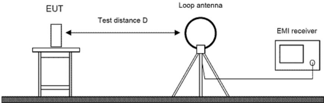
Figure 4. Radiated Emissions Test Setup (9kHz - 30MHz)
