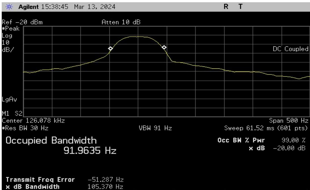
Plot 4 – 20dB BW
