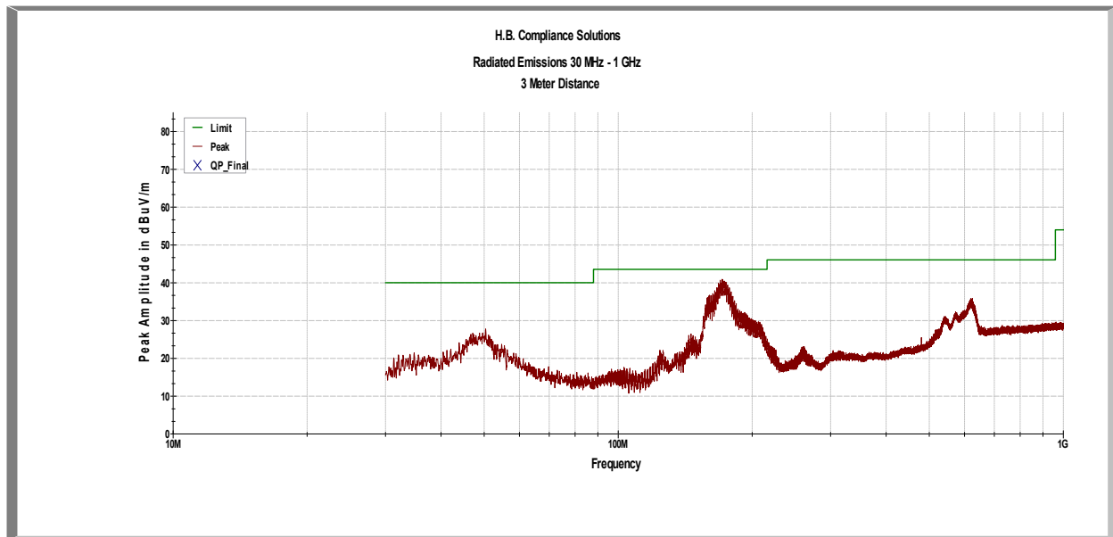
Plot 1 – Radiated Emissions – 30MHz to 1GHz
