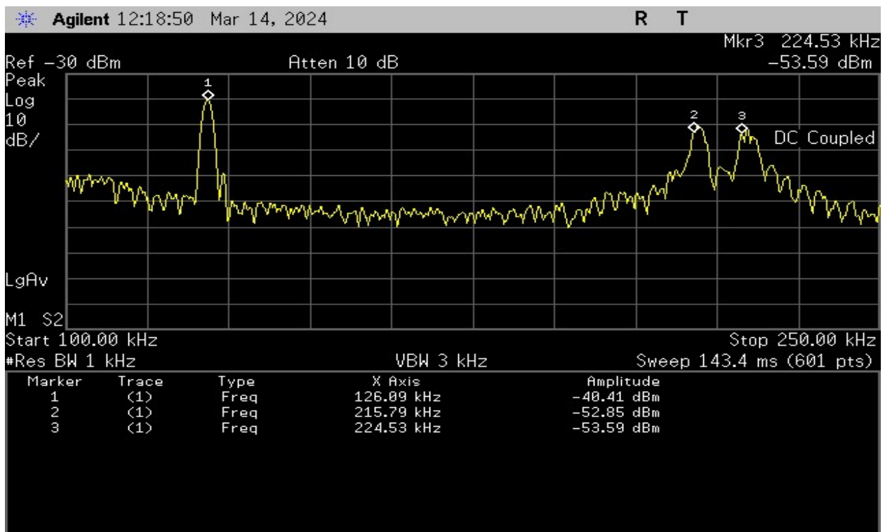
Plot 5 – Frequency of Fundamental WPT and Analog Pings
