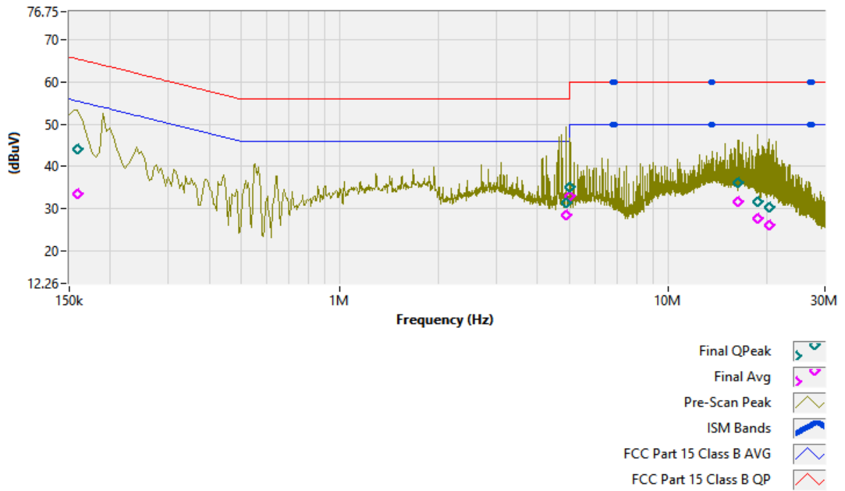
Plot 3 – Conducted Emissions – Neutral Side (Class B)
