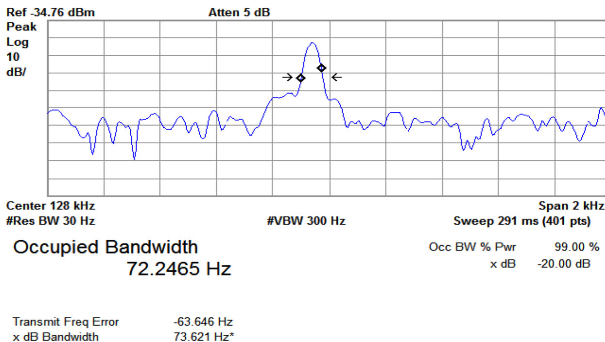
Plot 4 – 20dB BW
