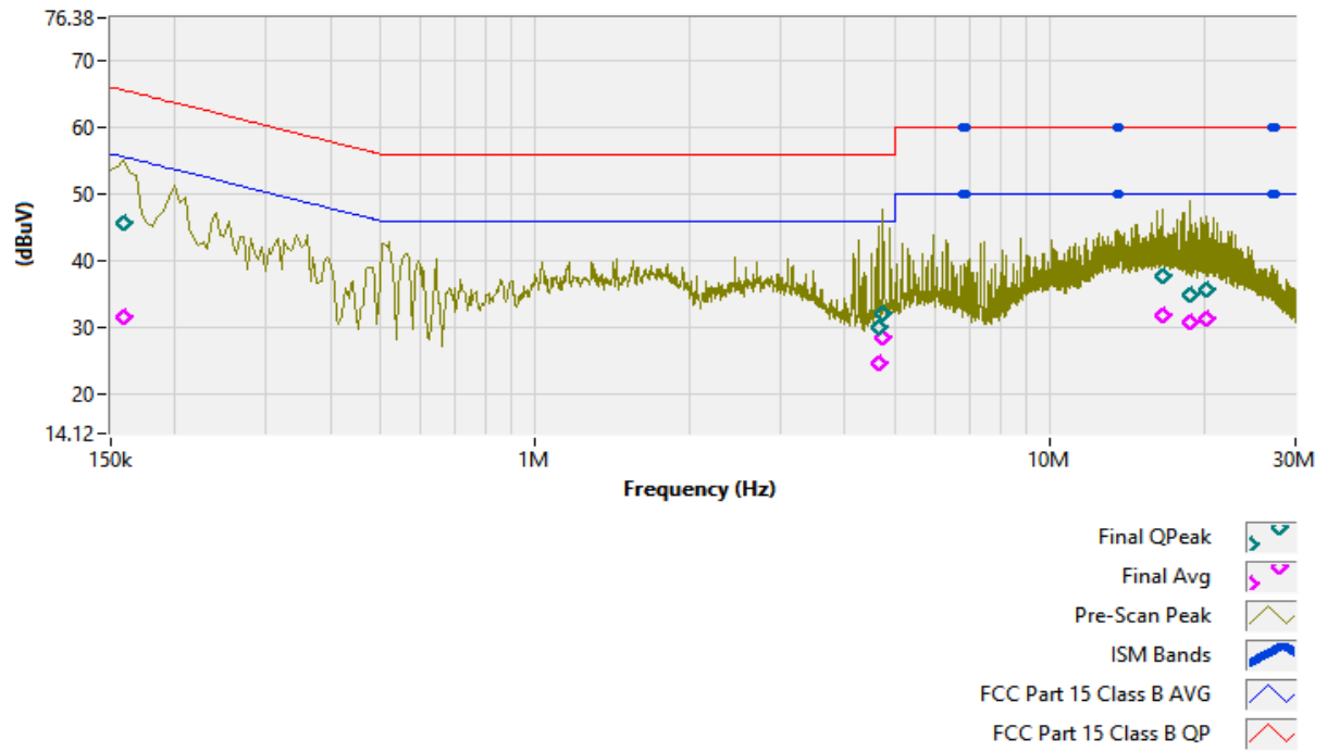
Plot 2 – Conducted Emission Plot – Line Side (Class B)
