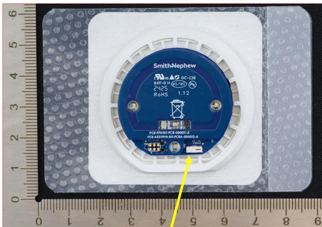
RF Chip Antenna location
