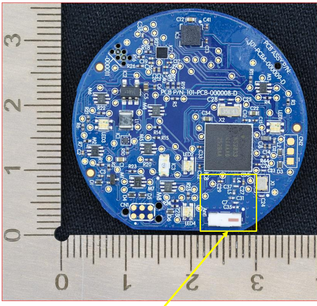
RF Section location including the RF Antenna (Ant 1)
