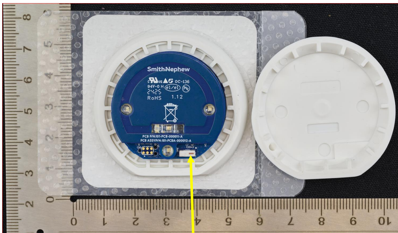
RF Chip Antenna location
