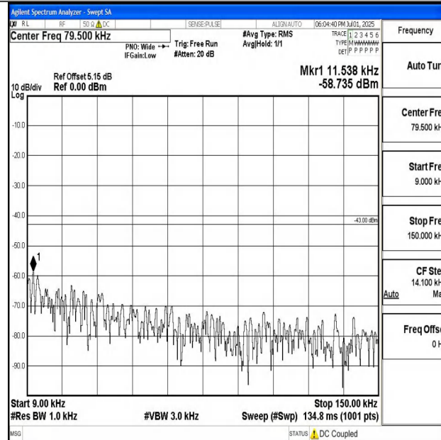
Band4_15MHz_QPSK_20025_1RB#0_0.009~0.15_0.009~0.15
