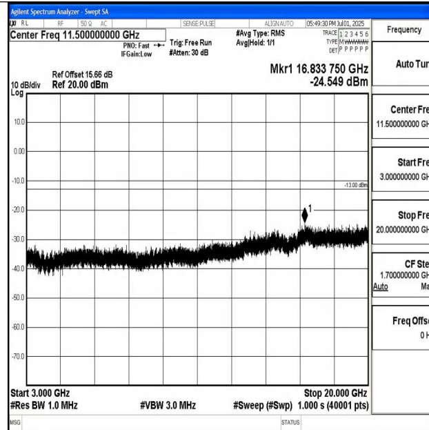
Band4_10MHz_16QAM_20175_1RB#0_3000~20000_3000~20000
