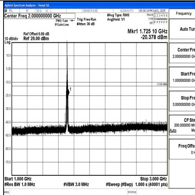
Band4_5MHz_16QAM_19975_1RB#0_1000~3000_1000~3000
