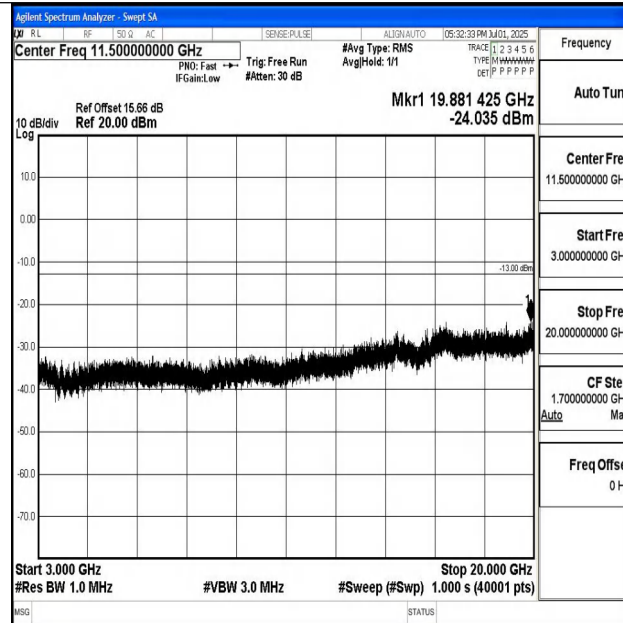
Band4_5MHz_16QAM_20375_1RB#0_3000~20000_3000~20000
