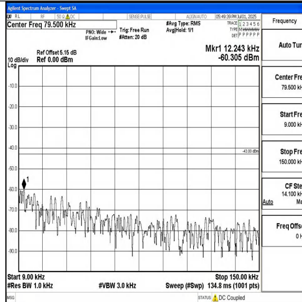
Band4_10MHz_QPSK_20350_1RB#0_0.009~0.15_0.009~0.15
