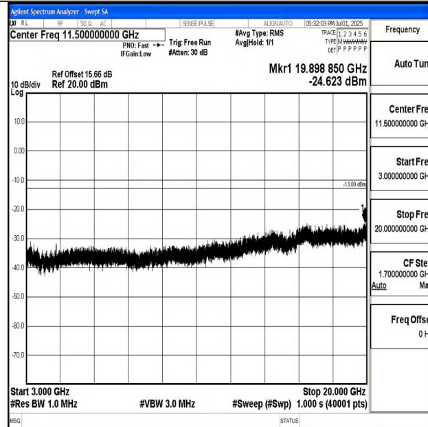
Band4_5MHz_QPSK_20375_1RB#0_3000~20000_3000~20000
