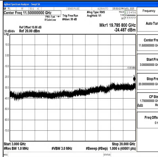
Band4_10MHz_QPSK_20350_1RB#0_3000~20000_3000~20000
