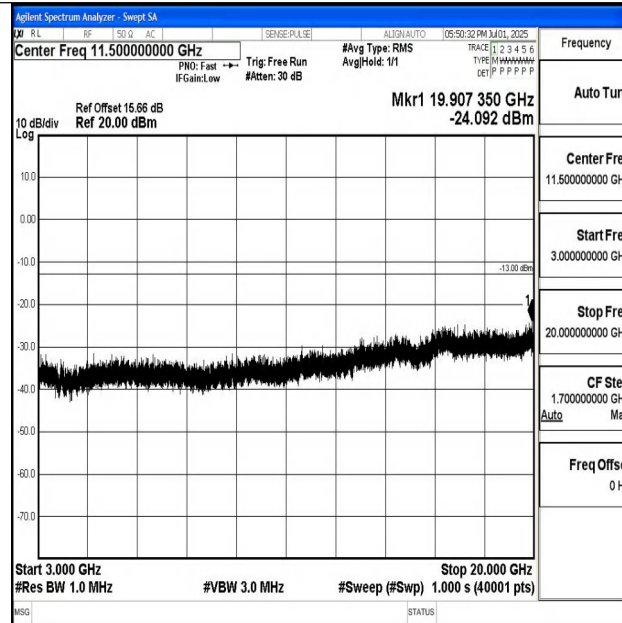
Band4_10MHz_16QAM_20350_1RB#0_3000~20000_3000~20000
