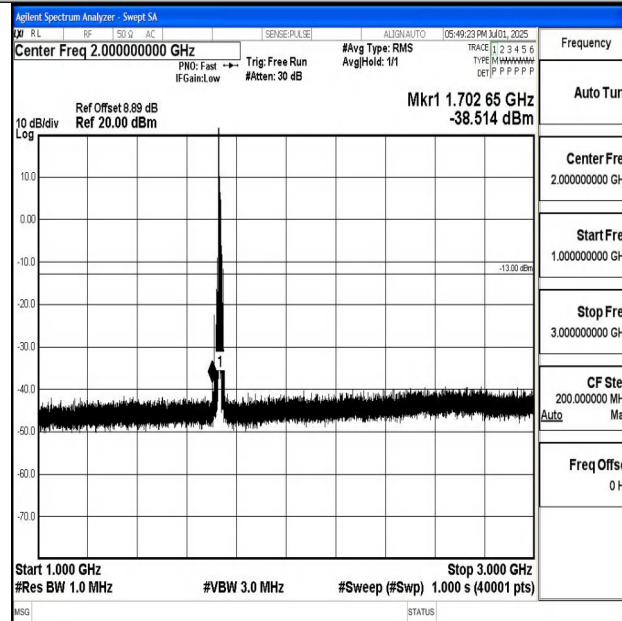
Band4_10MHz_16QAM_20175_1RB#0_1000~3000_1000~3000
