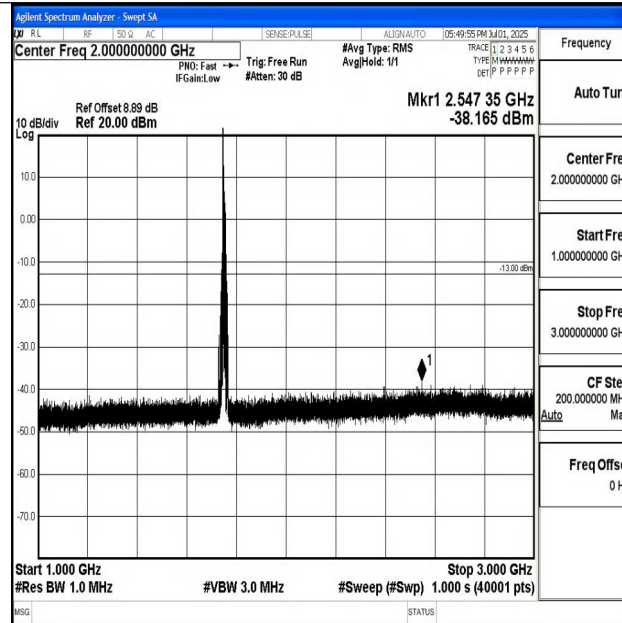
Band4_10MHz_QPSK_20350_1RB#0_1000~3000_1000~3000
