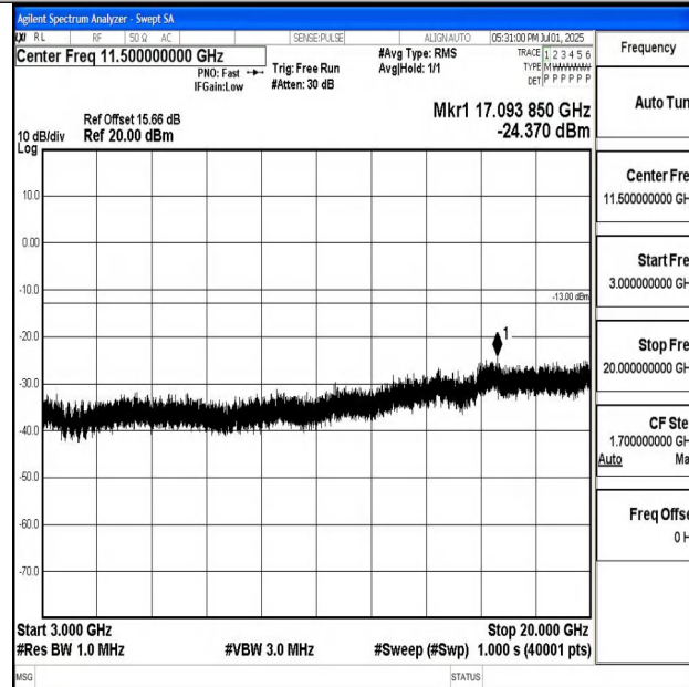
Band4_5MHz_QPSK_20175_1RB#0_3000~20000_3000~20000
