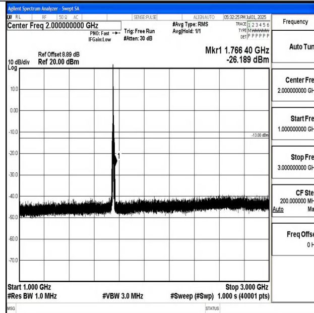
Band4_5MHz_16QAM_20375_1RB#0_1000~3000_1000~3000
