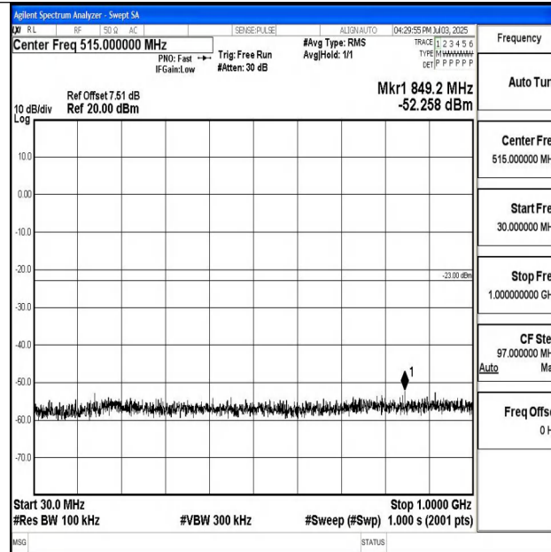
Band4_3MHz_16QAM_20385_1RB#0_30~1000_30~1000
