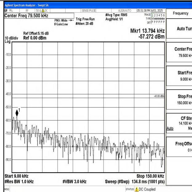
Band4_5MHz_QPSK_20375_1RB#0_0.009~0.15_0.009~0.15
