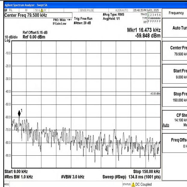
Band4_10MHz_QPSK_20175_1RB#0_0.009~0.15_0.009~0.15
