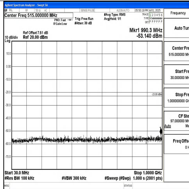
Band4_10MHz_16QAM_20350_1RB#0_30~1000_30~1000
