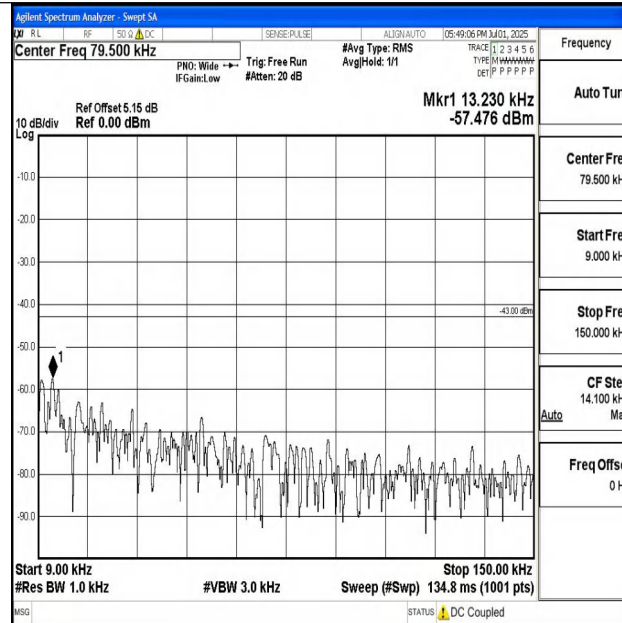
Band4_10MHz_16QAM_20175_1RB#0_0.009~0.15_0.009~0.15
