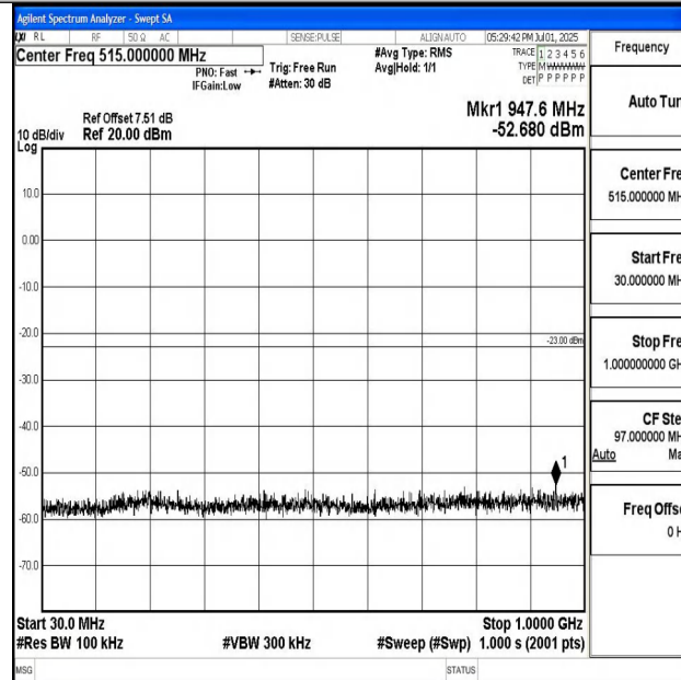
Band4_5MHz_QPSK_19975_1RB#0_30~1000_30~1000
