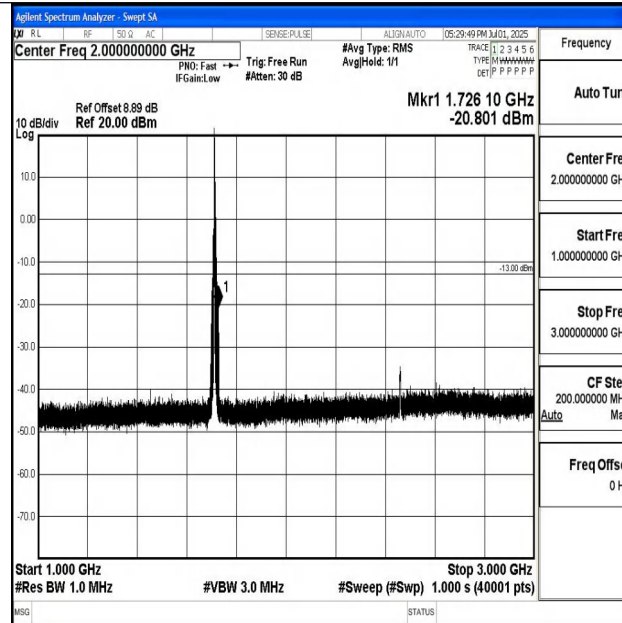
Band4_5MHz_QPSK_19975_1RB#0_1000~3000_1000~3000
