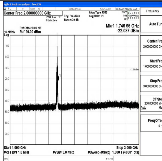
Band4_5MHz_16QAM_20175_1RB#0_1000~3000_1000~3000
