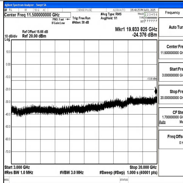
Band4_10MHz_16QAM_20000_1RB#0_3000~20000_3000~20000
