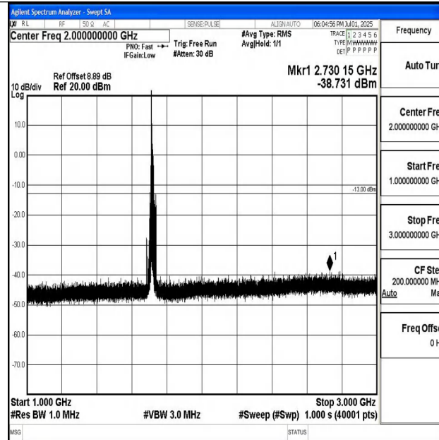
Band4_15MHz_QPSK_20025_1RB#0_1000~3000_1000~3000
