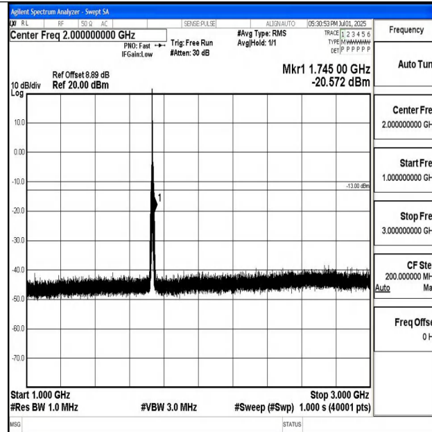
Band4_5MHz_QPSK_20175_1RB#0_1000~3000_1000~3000
