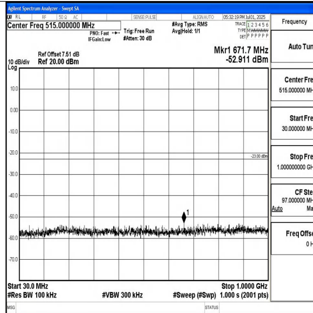
Band4_5MHz_16QAM_20375_1RB#0_30~1000_30~1000
