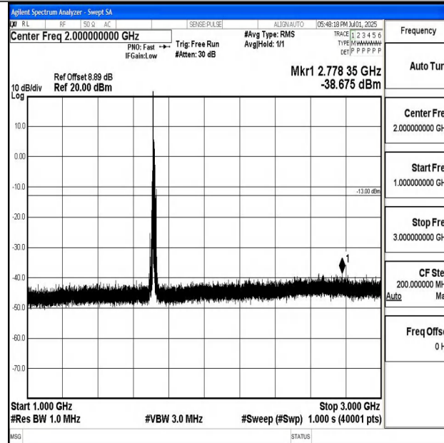
Band4_10MHz_16QAM_20000_1RB#0_1000~3000_1000~3000
