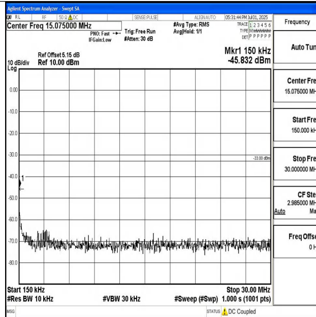
Band4_5MHz_QPSK_20375_1RB#0_0.15~30_0.15~30
