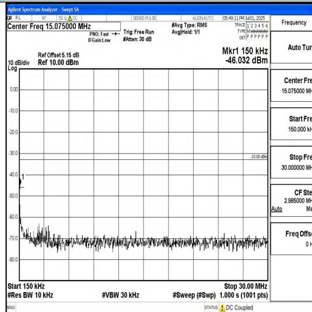
Band4_10MHz_16QAM_20175_1RB#0_0.15~30_0.15~30
