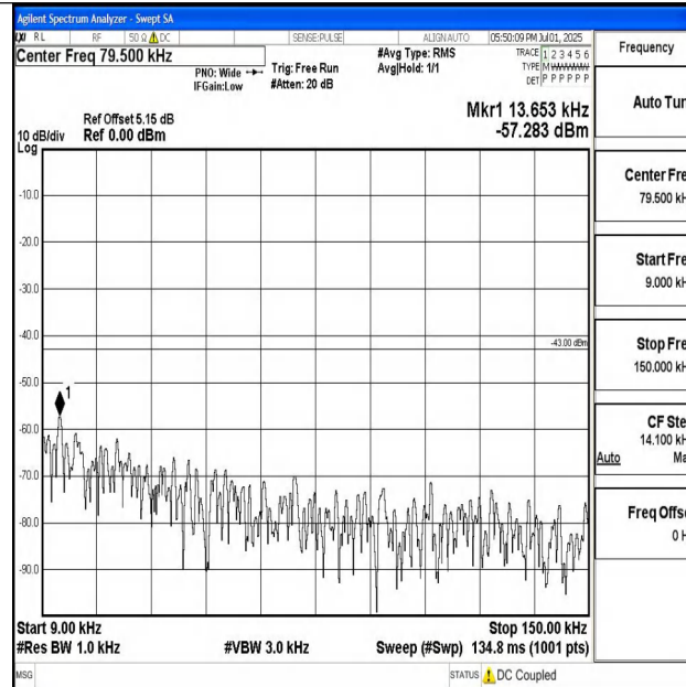
Band4_10MHz_16QAM_20350_1RB#0_0.009~0.15_0.009~0.15
