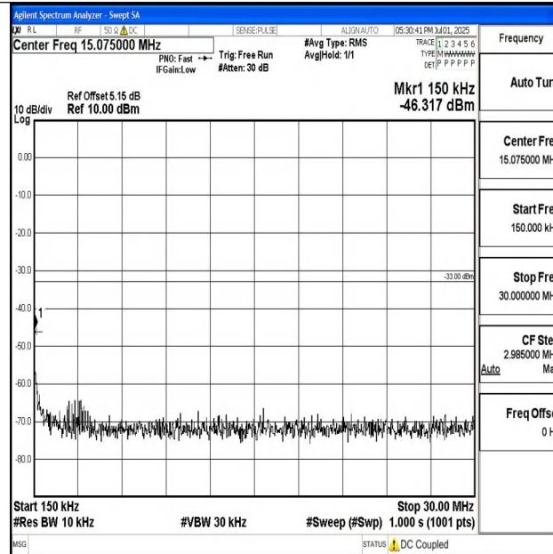
Band4_5MHz_QPSK_20175_1RB#0_0.15~30_0.15~30
