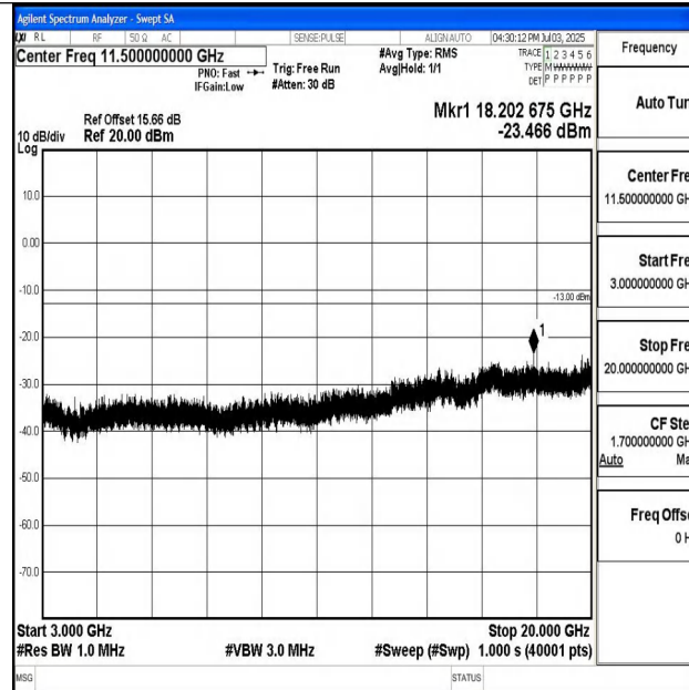
Band4_3MHz_16QAM_20385_1RB#0_3000~20000_3000~20000
