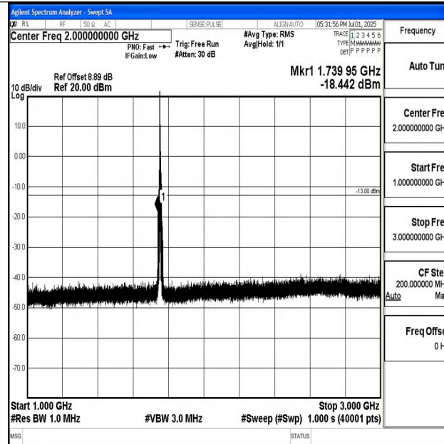
Band4_5MHz_QPSK_20375_1RB#0_1000~3000_1000~3000
