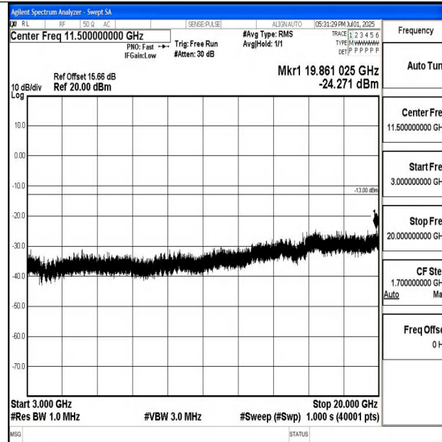
Band4_5MHz_16QAM_20175_1RB#0_3000~20000_3000~20000
