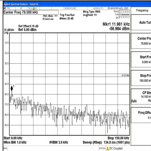
Band4_10MHz_16QAM_20000_1RB#0_0.009~0.15_0.009~0.15
