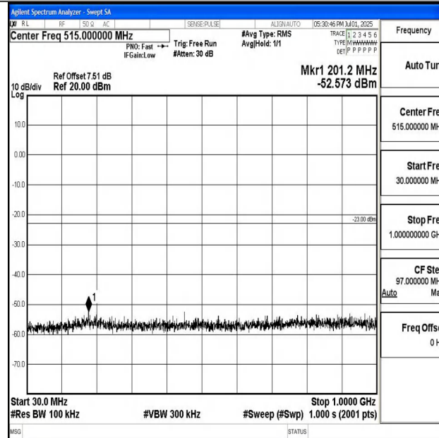
Band4_5MHz_QPSK_20175_1RB#0_30~1000_30~1000
