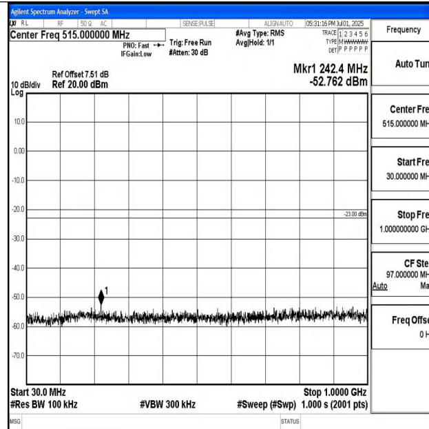
Band4_5MHz_16QAM_20175_1RB#0_30~1000_30~1000
