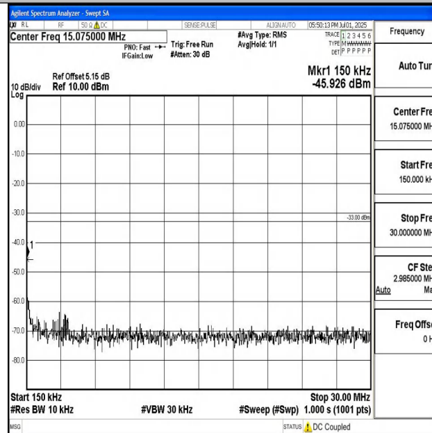
Band4_10MHz_16QAM_20350_1RB#0_0.15~30_0.15~30
