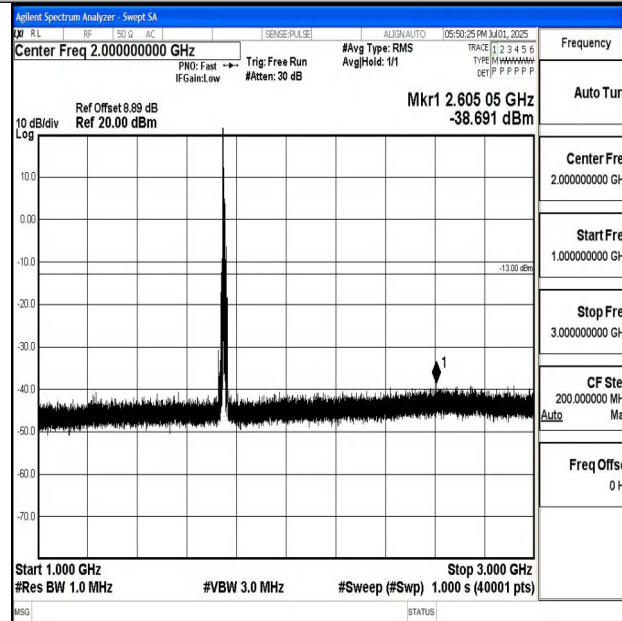
Band4_10MHz_16QAM_20350_1RB#0_1000~3000_1000~3000
