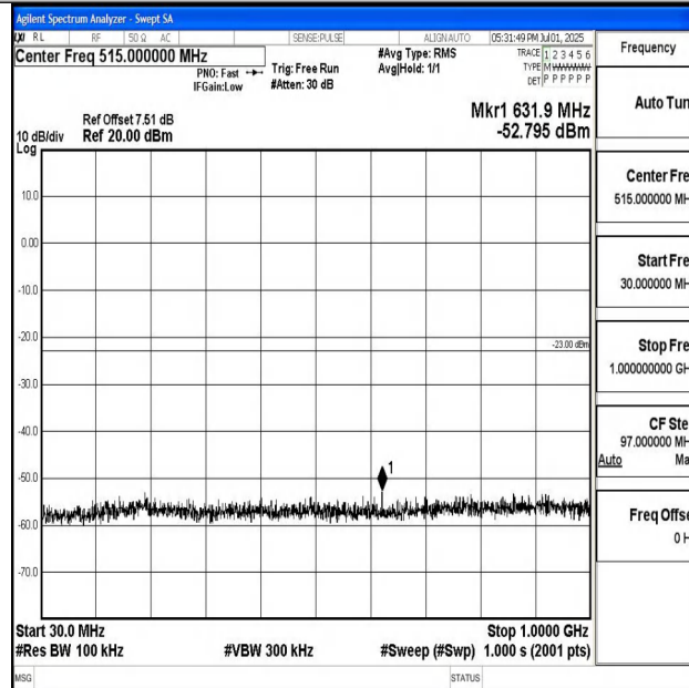
Band4_5MHz_QPSK_20375_1RB#0_30~1000_30~1000
