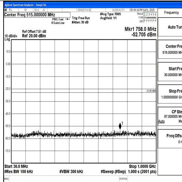
Band4_10MHz_16QAM_20175_1RB#0_30~1000_30~1000
