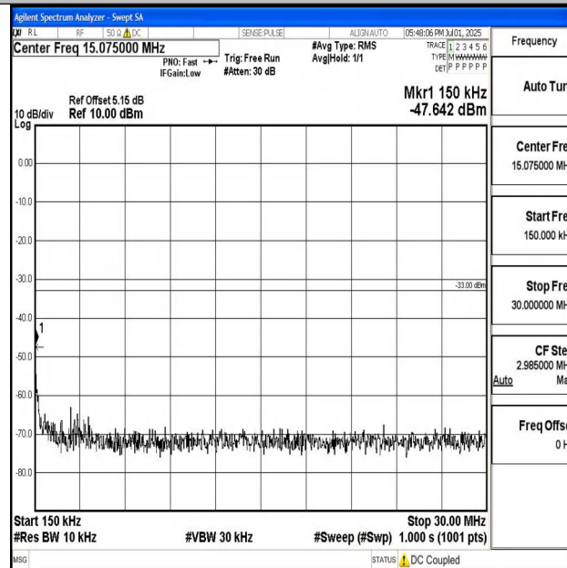
Band4_10MHz_16QAM_20000_1RB#0_0.15~30_0.15~30
