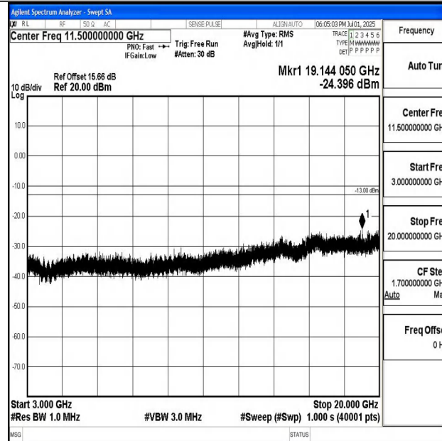
Band4_15MHz_QPSK_20025_1RB#0_3000~20000_3000~20000
