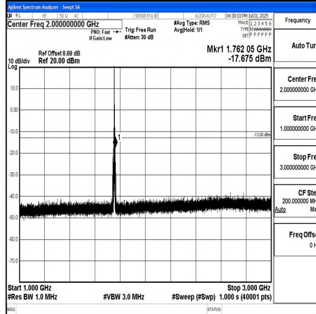
Band4_3MHz_16QAM_20385_1RB#0_1000~3000_1000~3000
