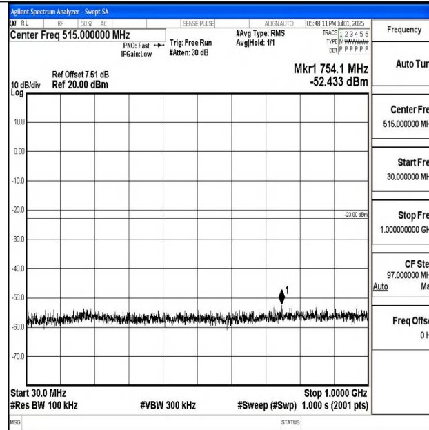
Band4_10MHz_16QAM_20000_1RB#0_30~1000_30~1000
