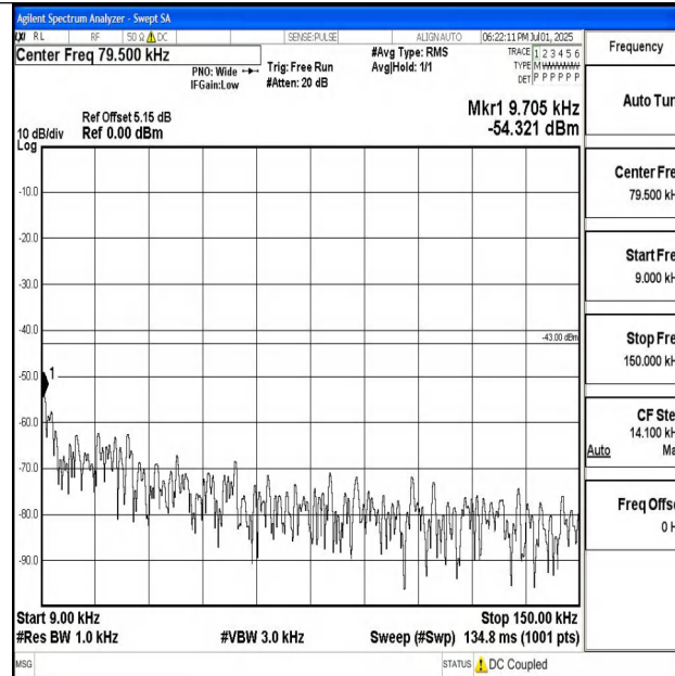
Band4_20MHz_16QAM_20050_1RB#0_0.009~0.15_0.009~0.15
