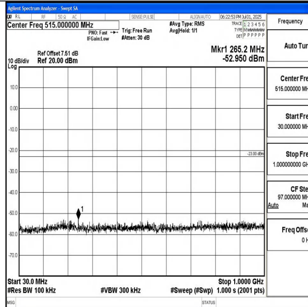
Band4_20MHz_QPSK_20175_1RB#0_30~1000_30~1000
