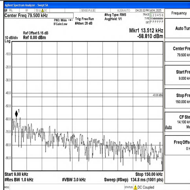
Band4_1.4MHz_QPSK_19957_1RB#0_0.009~0.15_0.009~0.15
