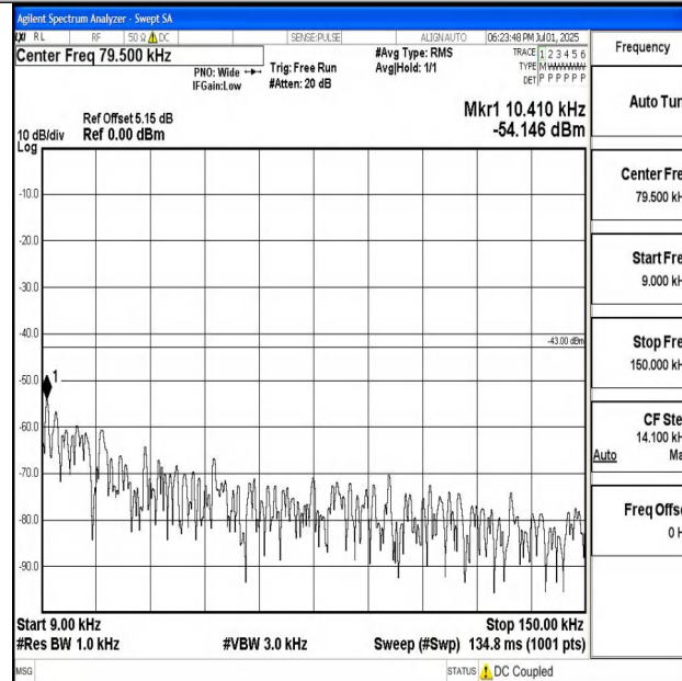
Band4_20MHz_QPSK_20300_1RB#0_0.009~0.15_0.009~0.15
