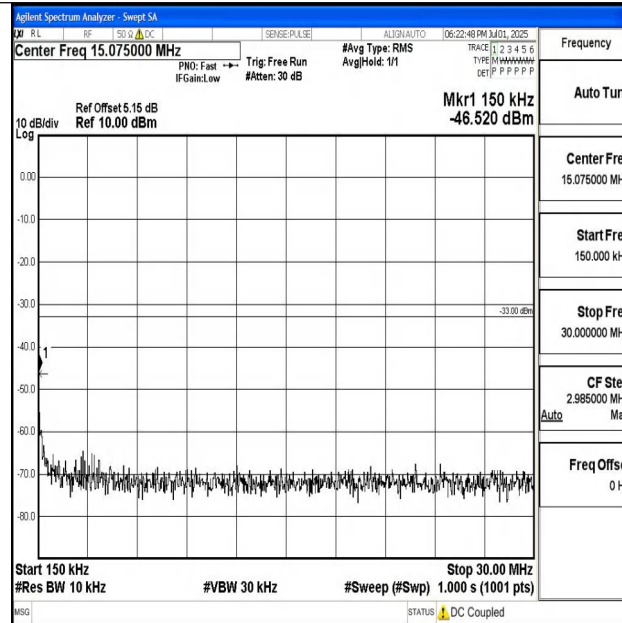
Band4_20MHz_QPSK_20175_1RB#0_0.15~30_0.15~30
