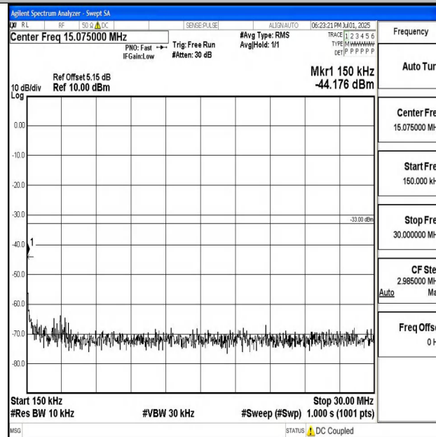
Band4_20MHz_16QAM_20175_1RB#0_0.15~30_0.15~30
