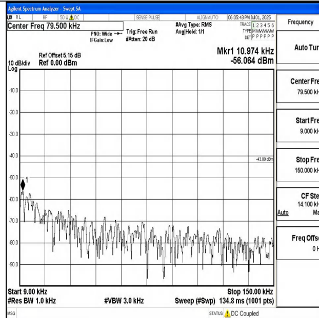
Band4_15MHz_QPSK_20175_1RB#0_0.009~0.15_0.009~0.15
