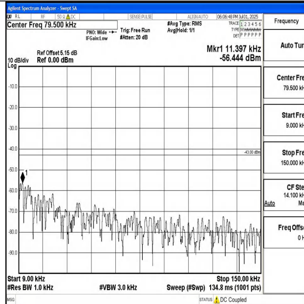
Band4_15MHz_QPSK_20325_1RB#0_0.009~0.15_0.009~0.15
