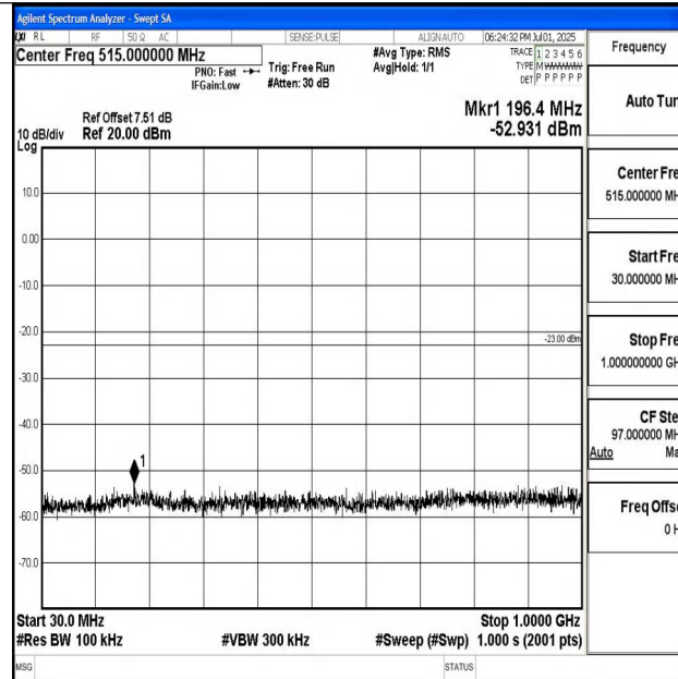
Band4_20MHz_16QAM_20300_1RB#0_30~1000_30~1000
