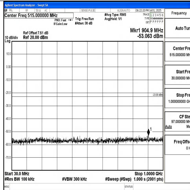
Band4_20MHz_16QAM_20050_1RB#0_30~1000_30~1000
