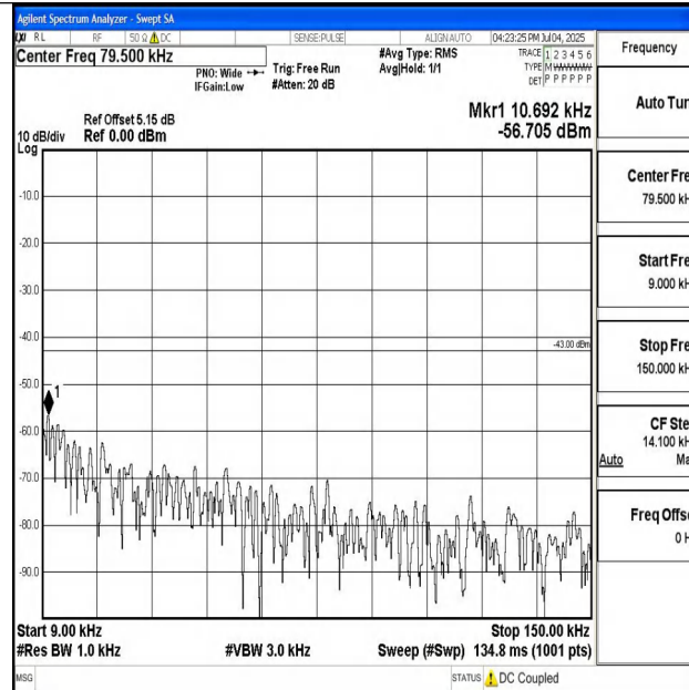
Band4_1.4MHz_16QAM_20393_1RB#0_0.009~0.15_0.009~0.15
