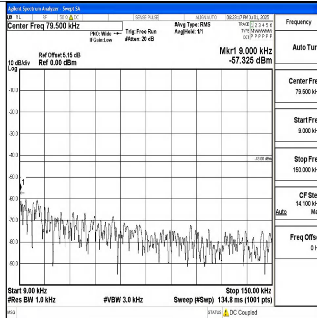
Band4_20MHz_16QAM_20175_1RB#0_0.009~0.15_0.009~0.15
