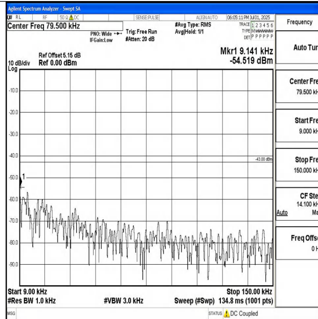
Band4_15MHz_16QAM_20025_1RB#0_0.009~0.15_0.009~0.15
