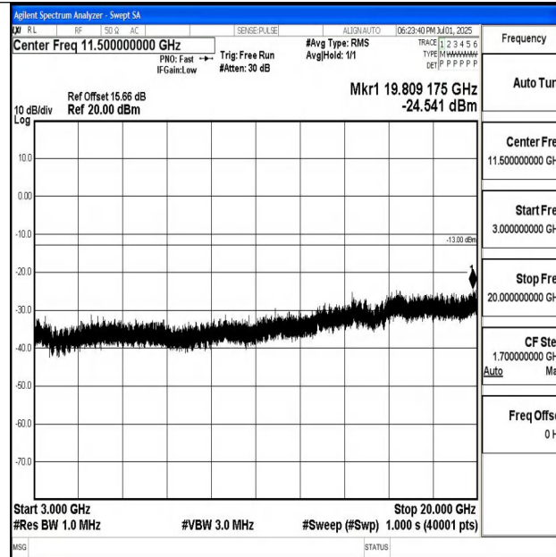
Band4_20MHz_16QAM_20175_1RB#0_3000~20000_3000~20000
