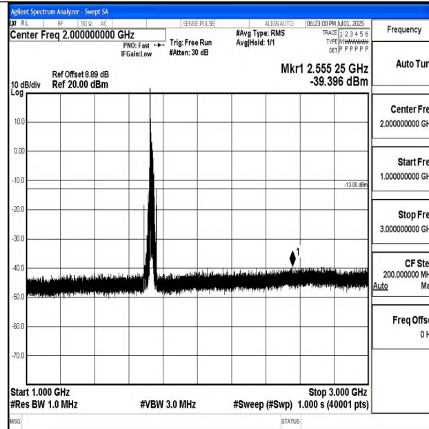
Band4_20MHz_QPSK_20175_1RB#0_1000~3000_1000~3000
