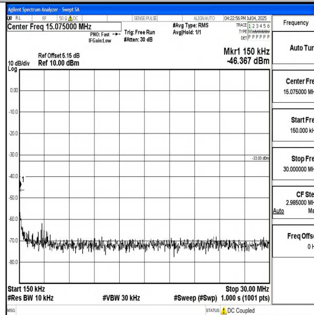
Band4_1.4MHz_QPSK_20393_1RB#0_0.15~30_0.15~30
