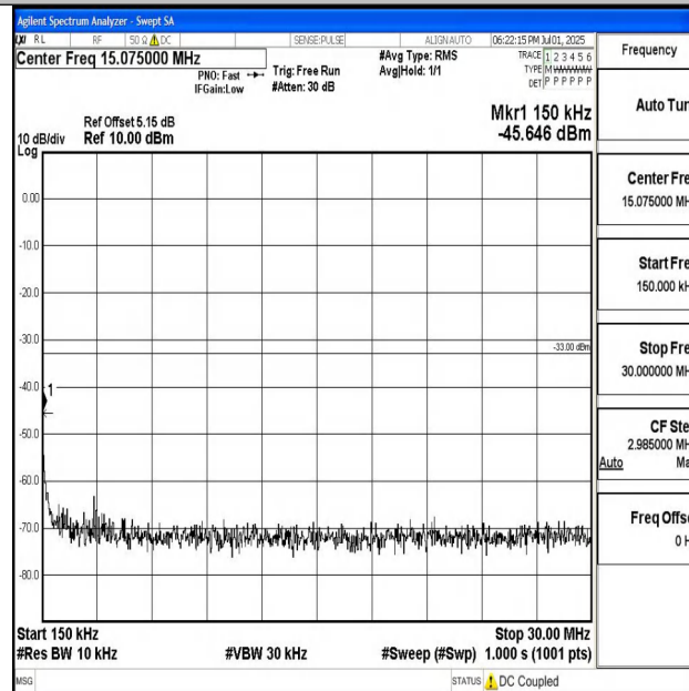
Band4_20MHz_16QAM_20050_1RB#0_0.15~30_0.15~30
