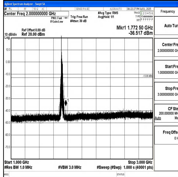
Band4_20MHz_16QAM_20050_1RB#0_1000~3000_1000~3000
