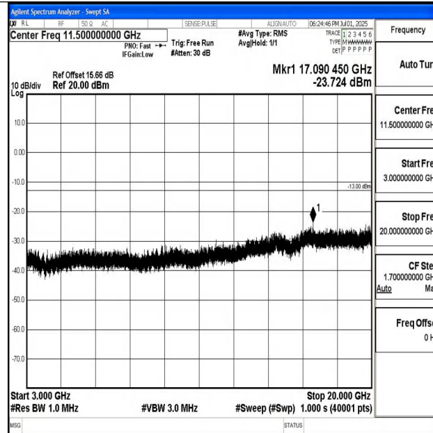
Band4_20MHz_16QAM_20300_1RB#0_3000~20000_3000~20000
