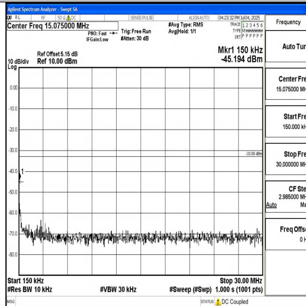
Band4_1.4MHz_16QAM_20393_1RB#0_0.15~30_0.15~30
