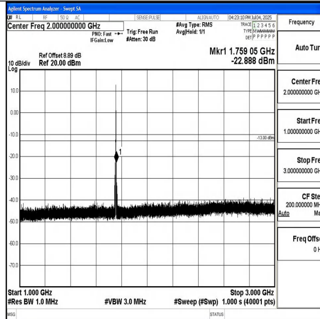
Band4_1.4MHz_QPSK_20393_1RB#0_1000~3000_1000~3000
