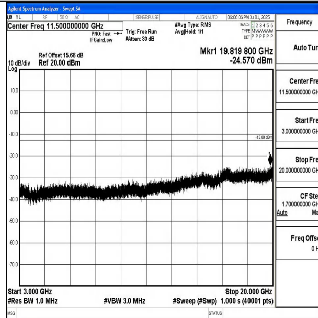
Band4_15MHz_QPSK_20175_1RB#0_3000~20000_3000~20000
