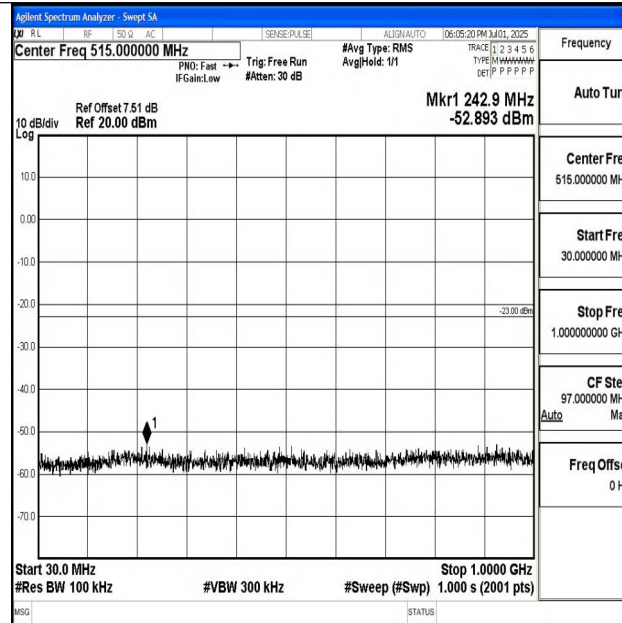
Band4_15MHz_16QAM_20025_1RB#0_30~1000_30~1000
