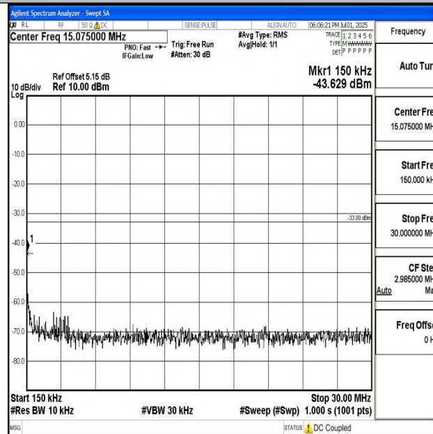
Band4_15MHz_16QAM_20175_1RB#0_0.15~30_0.15~30
