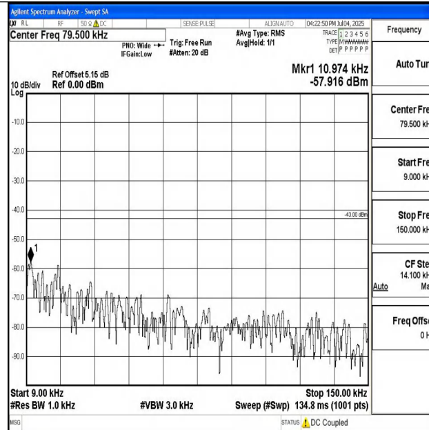
Band4_1.4MHz_QPSK_20393_1RB#0_0.009~0.15_0.009~0.15
