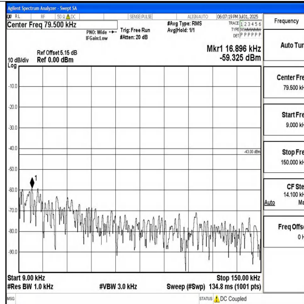
Band4_15MHz_16QAM_20325_1RB#0_0.009~0.15_0.009~0.15
