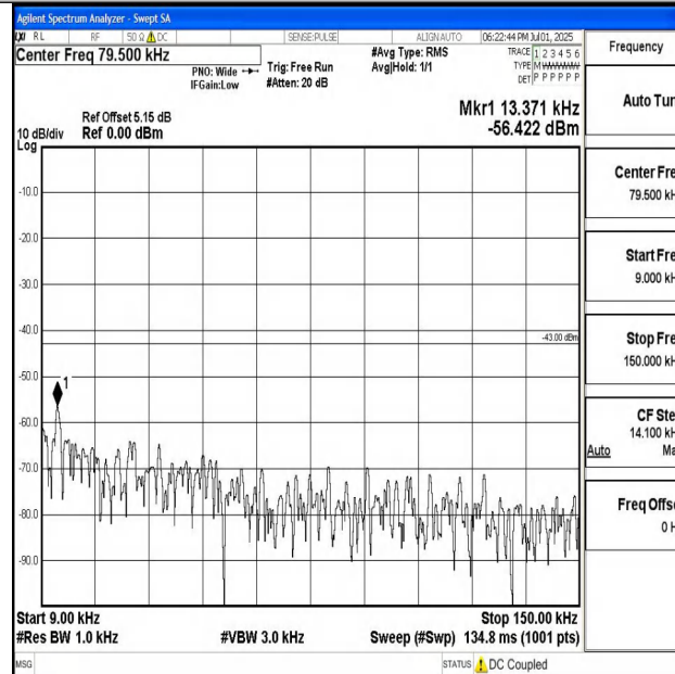
Band4_20MHz_QPSK_20175_1RB#0_0.009~0.15_0.009~0.15
