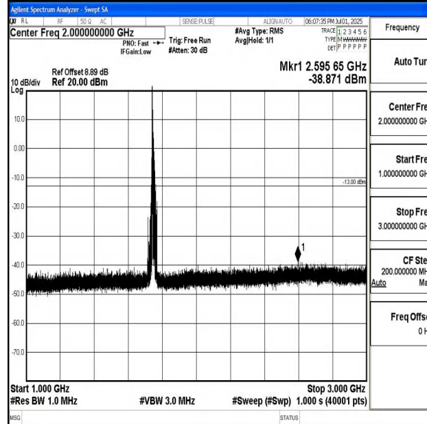
Band4_15MHz_16QAM_20325_1RB#0_1000~3000_1000~3000
