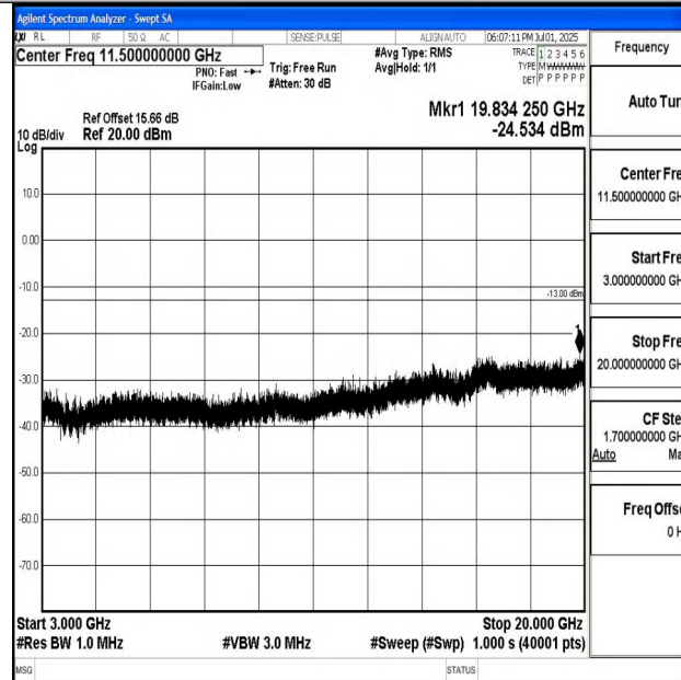
Band4_15MHz_QPSK_20325_1RB#0_3000~20000_3000~20000
