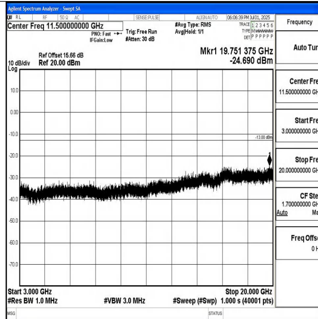
Band4_15MHz_16QAM_20175_1RB#0_3000~20000_3000~20000
