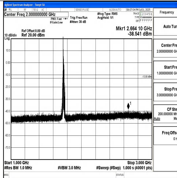
Band4_15MHz_QPSK_20325_1RB#0_1000~3000_1000~3000
