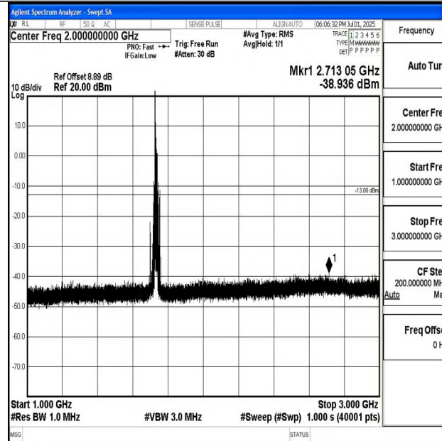
Band4_15MHz_16QAM_20175_1RB#0_1000~3000_1000~3000
