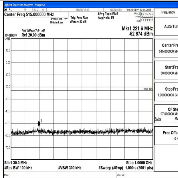
Band4_1.4MHz_QPSK_20393_1RB#0_30~1000_30~1000
