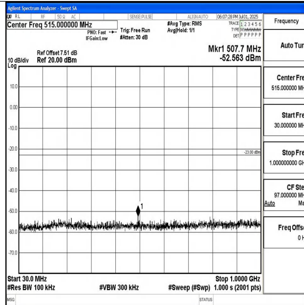
Band4_15MHz_16QAM_20325_1RB#0_30~1000_30~1000
