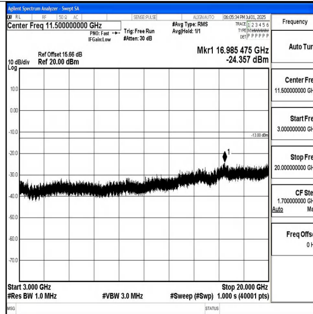
Band4_15MHz_16QAM_20025_1RB#0_3000~20000_3000~20000
