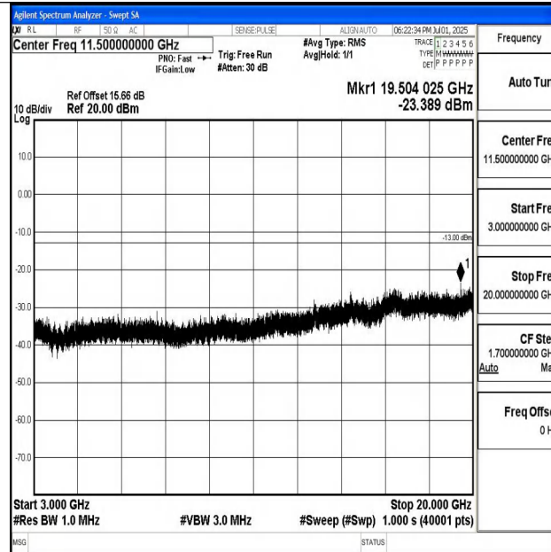
Band4_20MHz_16QAM_20050_1RB#0_3000~20000_3000~20000
