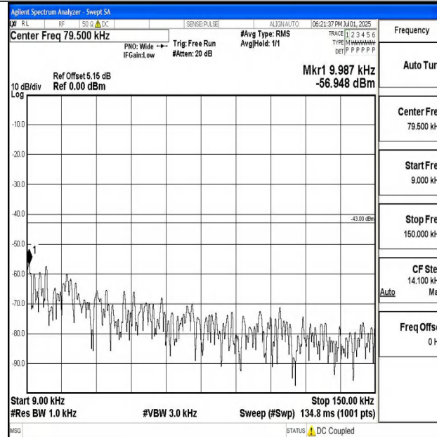
Band4_20MHz_QPSK_20050_1RB#0_0.009~0.15_0.009~0.15
