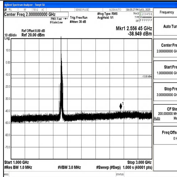
Band4_15MHz_16QAM_20025_1RB#0_1000~3000_1000~3000
